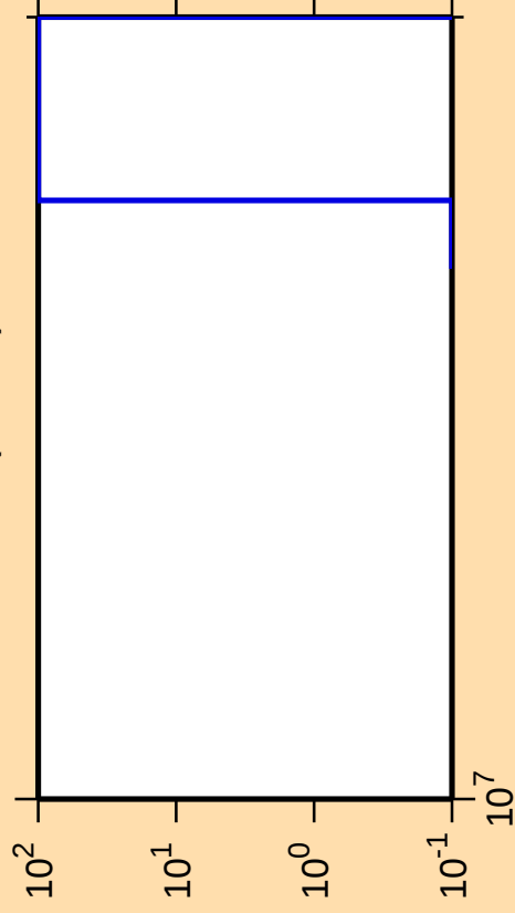
\Delta\sigma/\sigma vs. E for ^{83}\text{Sr}(\text{mt } 34)
