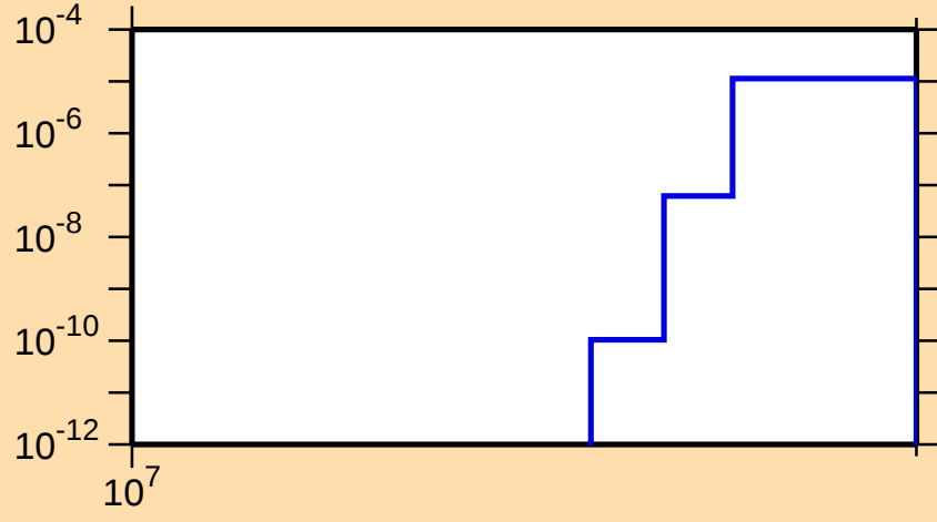
\sigma vs. E for ^{83}\text{Sr}(n,\text{nd})
