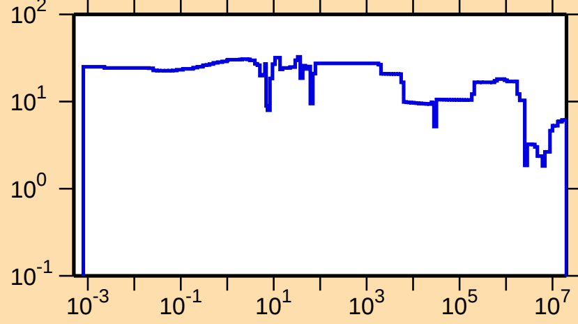
\Delta\sigma/\sigma vs. E for ^{83}\text{Sr}(n,\text{tot.})
