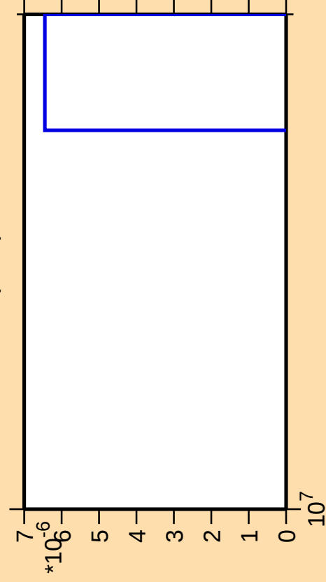
\Delta\sigma/\sigma vs. E for ^{83}\text{Sr}(n,\text{nt})
