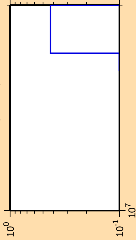
\Delta\sigma/\sigma vs. E for ^{83}\text{Sr}(\text{mt117})
