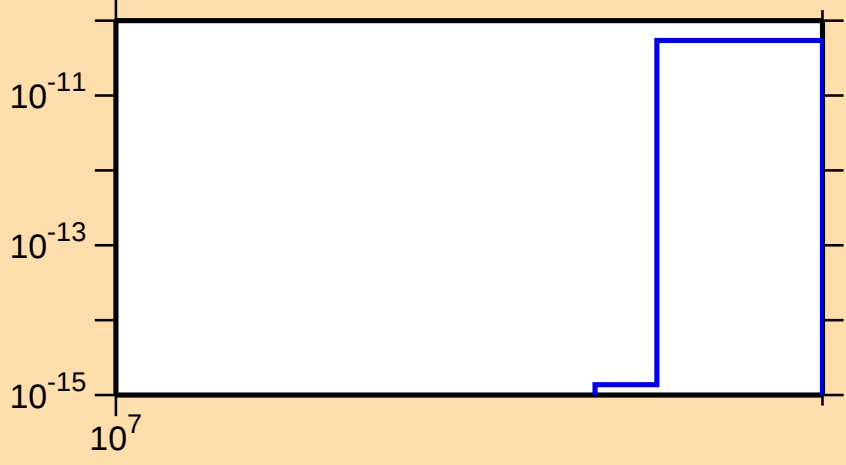
\sigma vs. E for ^{83}\text{Sr}(\text{mt } 34)
