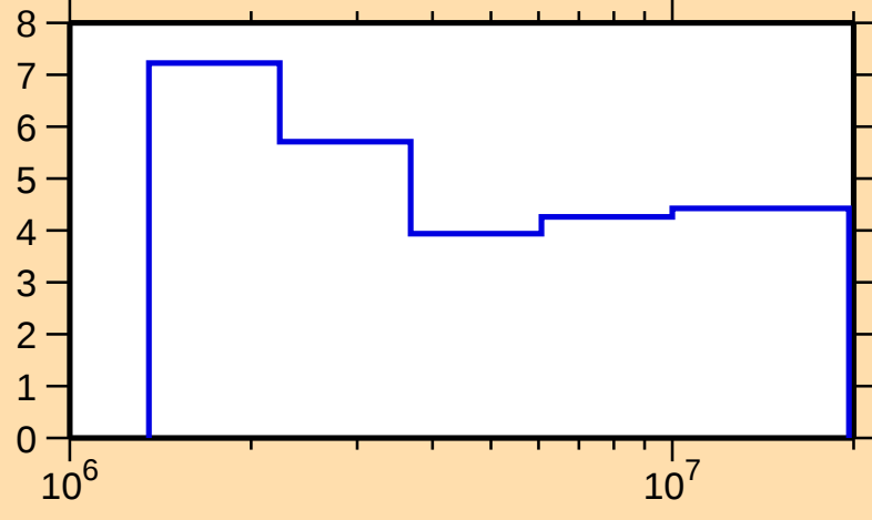
\Delta\sigma/\sigma vs. E for ^{83}\text{Sr}(n,n\text{onel.})
