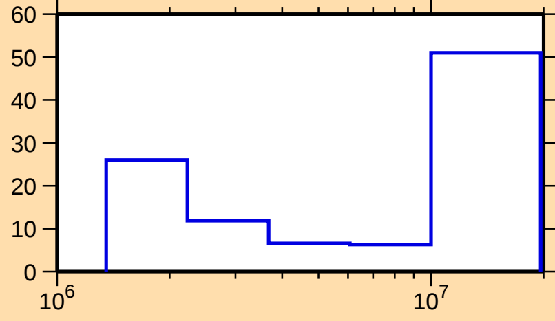
\Delta\sigma/\sigma vs. E for ^{83}\text{Sr}(n,\text{ncont.})
