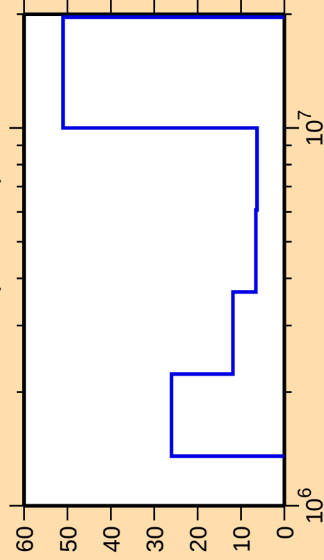
\Delta\sigma/\sigma vs. E for ^{83}\text{Sr}(n,\text{ncont.})
