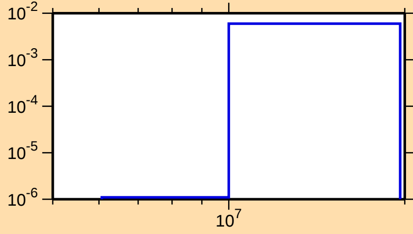
\sigma vs. E for ^{83}\text{Sr}(n,d)
