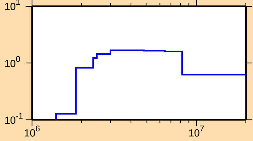
\sigma vs. E for ^{83}\text{Sr}(n,n\text{cont.})
