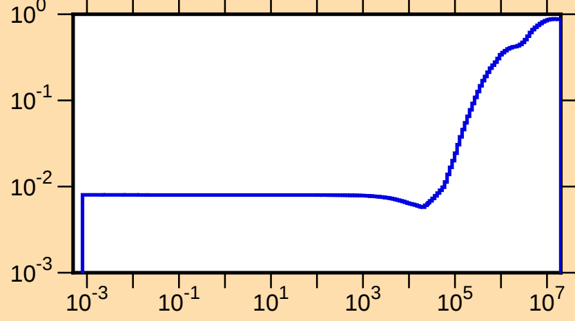
\mu vs. E for ^{84}\text{Sr}(\text{mt251})
