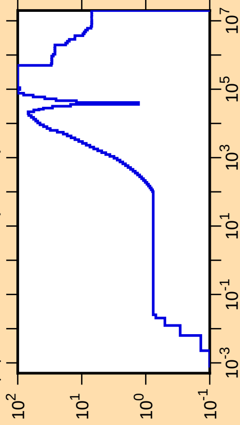
\Delta\mu/\mu vs. E for ^{84}\text{Sr}(\text{mt251})
