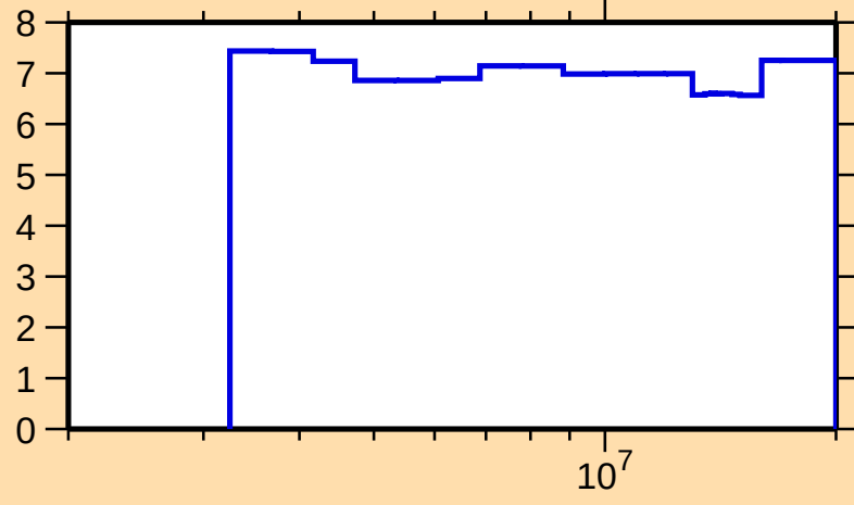
\Delta\sigma/\sigma vs. E for ^{84}\text{Sr}(n,n\text{oncl.})
