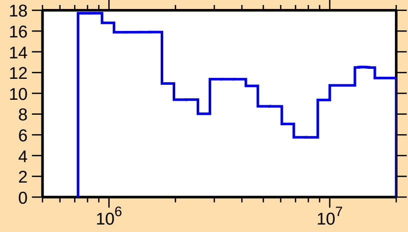
\Delta\sigma/\sigma vs. E for ^{84}\text{Sr}(\text{n,el.})
