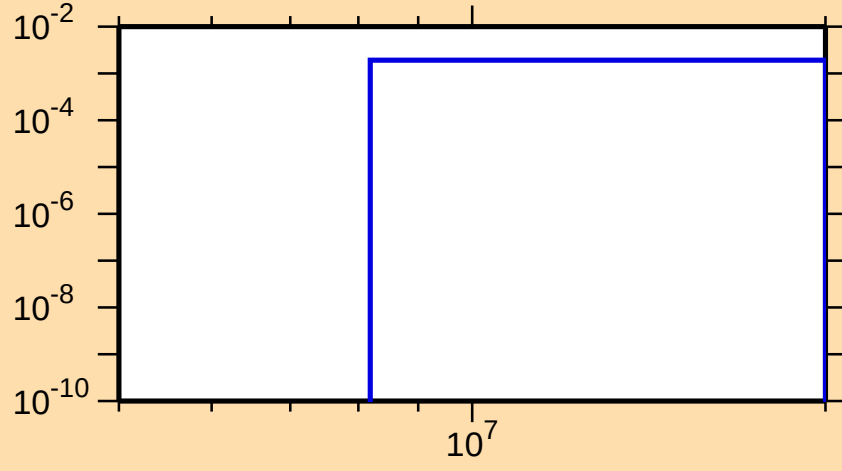
\sigma vs. E for ^{84}\text{Sr}(n,d)
