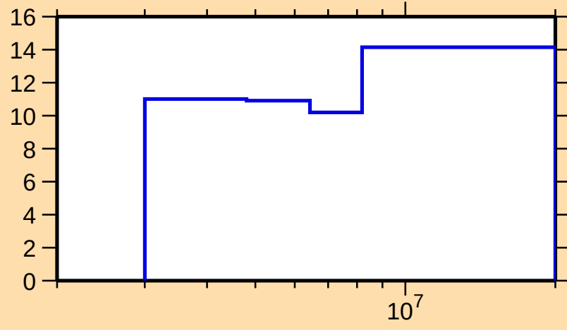
\Delta\sigma/\sigma vs. E for ^{84}\text{Sr}(n,n\text{cont.})
