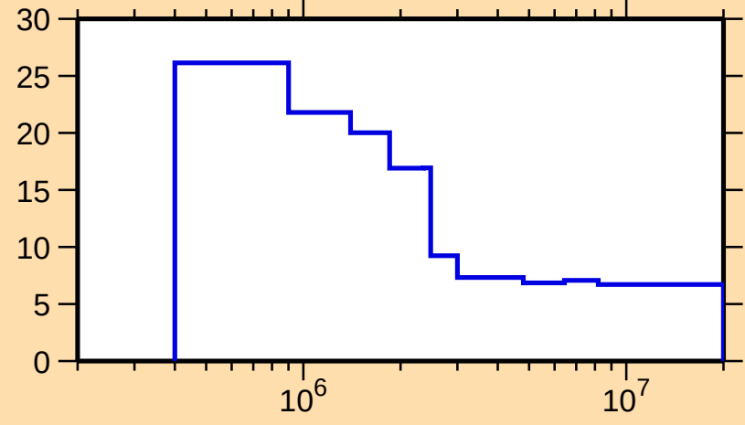
\Delta\sigma/\sigma vs. E for ^{84}\text{Sr}(\text{n,nonel.})
