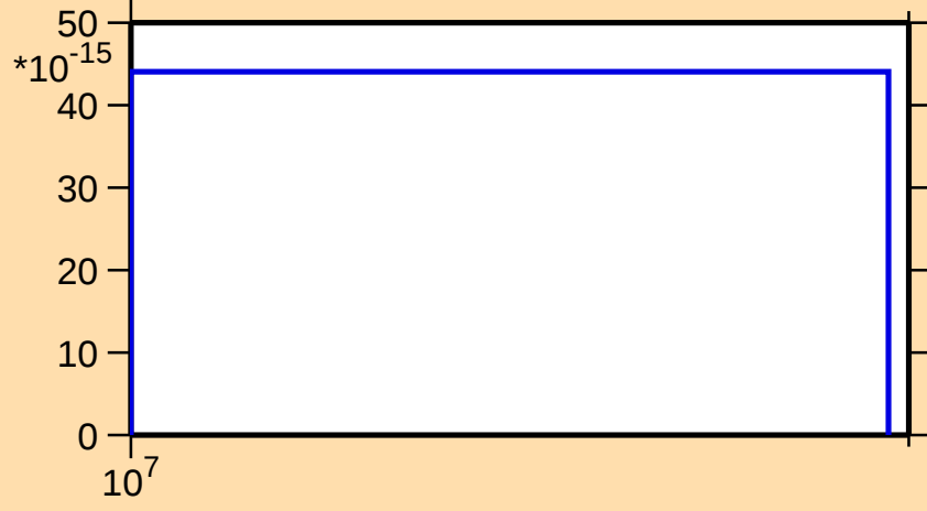
\sigma vs. E for ^{85}\text{Sr}(n,\text{pt})
