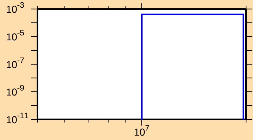
\sigma vs. E for ^{85}\text{Sr}(n,n\alpha)
