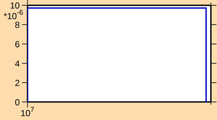
\sigma vs. E for ^{85}\text{Sr}(n,t)
