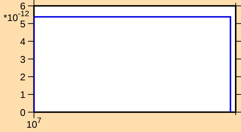
\sigma vs. E for ^{85}\text{Sr}(n,2n\alpha)
