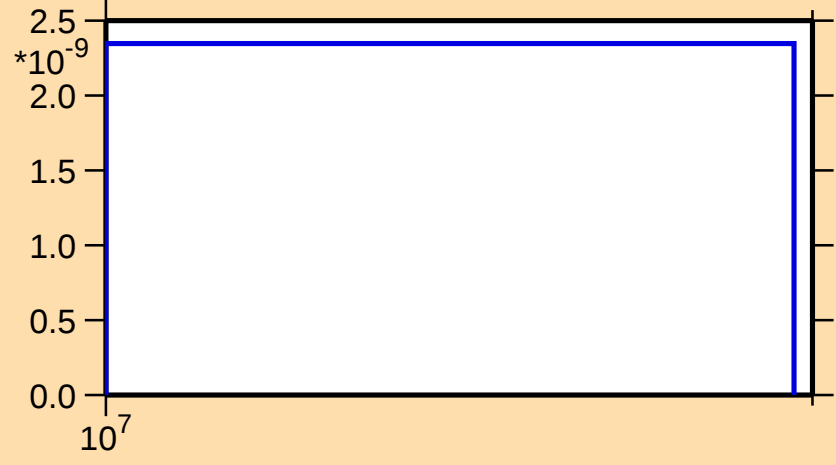
\sigma vs. E for ^{85}\text{Sr}(n,2np)
