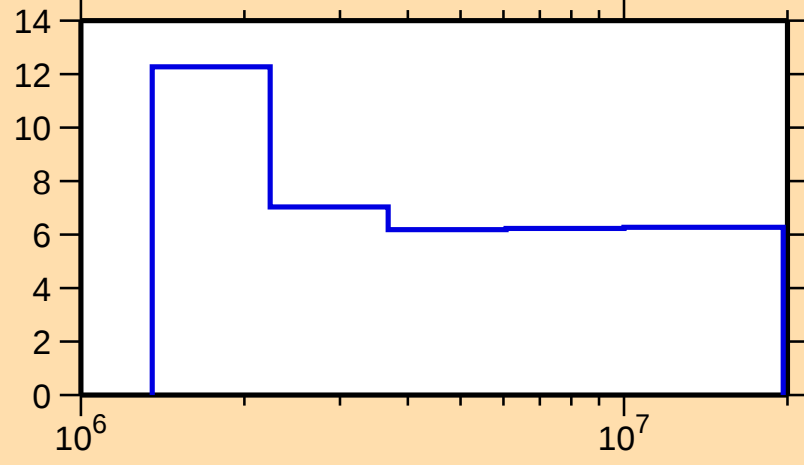
\Delta\sigma/\sigma vs. E for ^{85}\text{Sr}(n,\text{nonel.})
