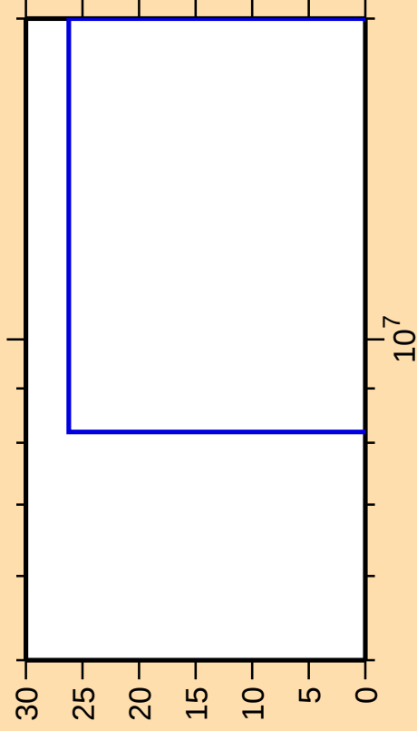
\Delta\sigma/\sigma vs. E for ^{85}\text{Sr}(n,2n)
