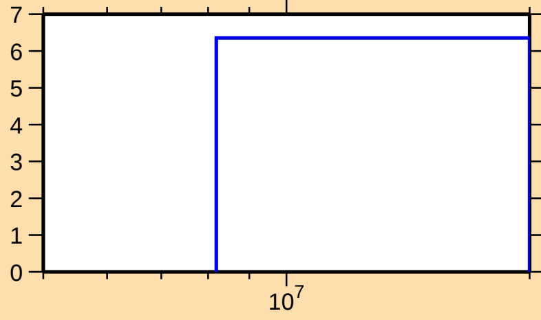
\Delta\sigma/\sigma vs. E for ^{85}\text{Sr}(n,\text{tot.})
