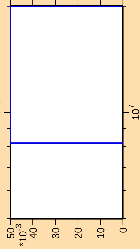
\Delta\sigma/\sigma vs. E for ^{85}\text{Sr}(n,\text{pt})
