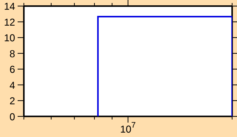
\Delta\sigma/\sigma vs. E for ^{85}\text{Sr}(n,\text{el.})
