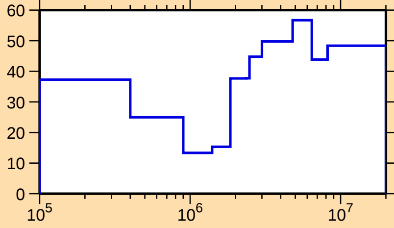
\Delta\sigma/\sigma vs. E for ^{85}\text{Sr}(n,n_1)
