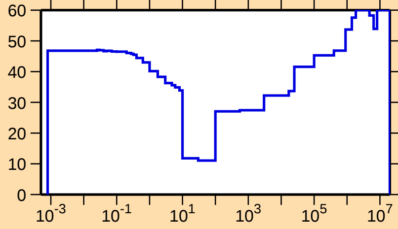
\Delta\sigma/\sigma vs. E for ^{85}\text{Sr}(n,\gamma)
