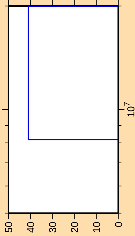
\Delta\sigma/\sigma vs. E for ^{85}\text{Sr}(n,n\text{cont.})
