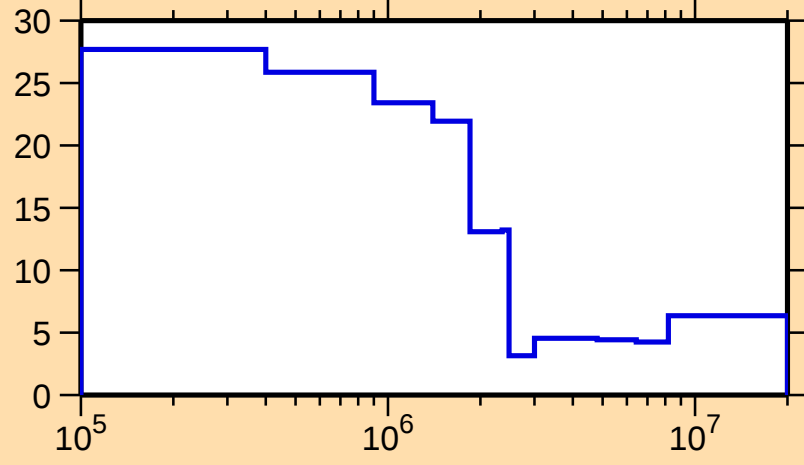
\Delta\sigma/\sigma vs. E for ^{85}\text{Sr}(n,\text{tot.})
