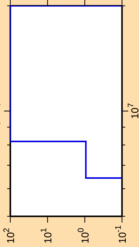
\Delta\sigma/\sigma vs. E for ^{85}\text{Sr}(n,d)
