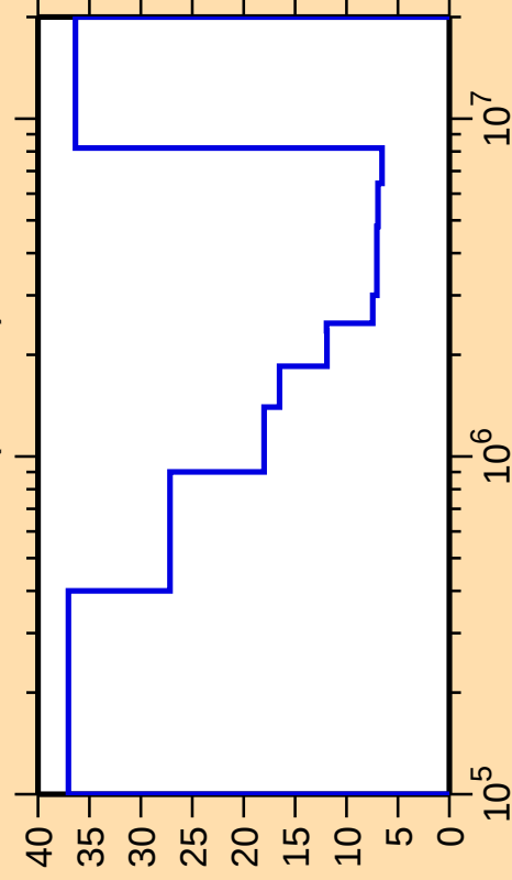
\Delta\sigma/\sigma vs. E for ^{85}\text{Sr}(\text{n,inel.})
