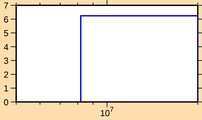
\Delta\sigma/\sigma vs. E for ^{85}\text{Sr}(n,\text{nonel.})
