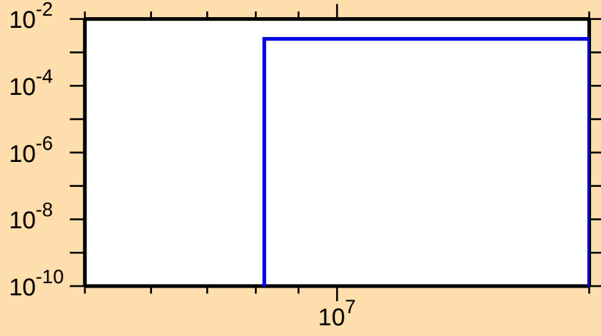
\sigma vs. E for ^{85}\text{Sr}(n,d)
