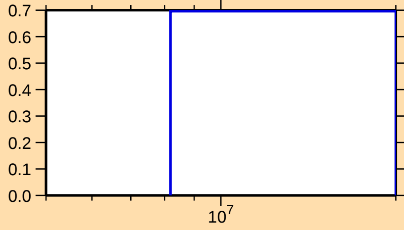
\sigma vs. E for ^{85}\text{Sr}(n,2n)
