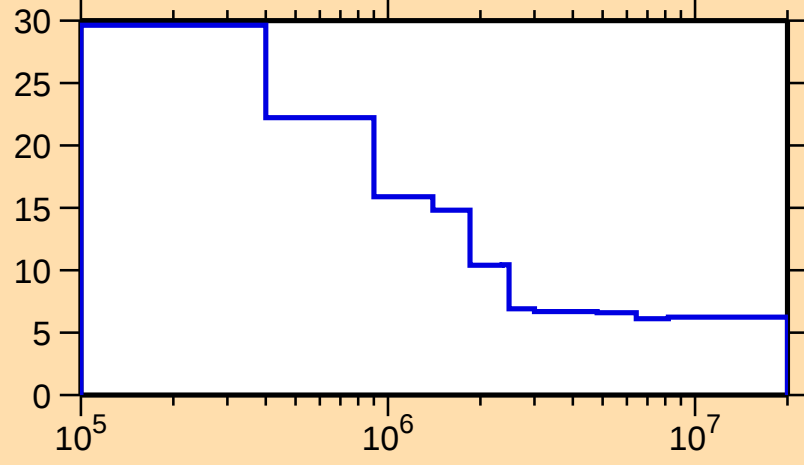
\Delta\sigma/\sigma vs. E for ^{85}\text{Sr}(\text{n,nonel.})
