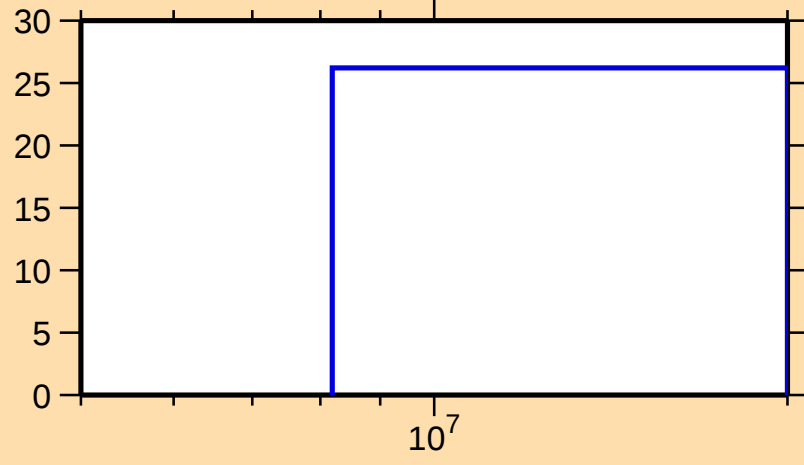
\Delta\sigma/\sigma vs. E for ^{85}\text{Sr}(n,2n)
