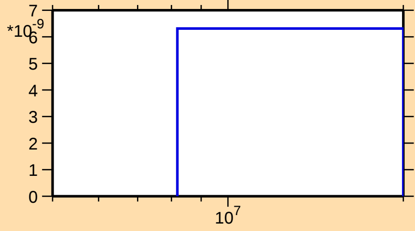
\sigma vs. E for ^{85}\text{Sr}(n,\text{He}3)
