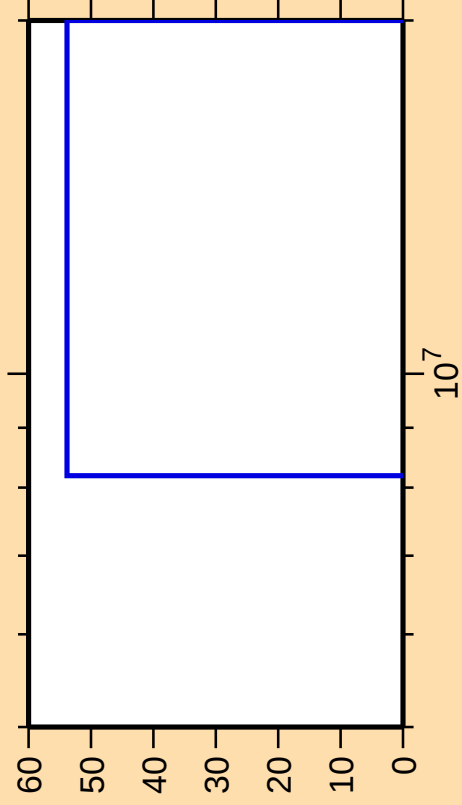
\Delta\sigma/\sigma vs. E for ^{85}\text{Sr}(n,n\alpha)
