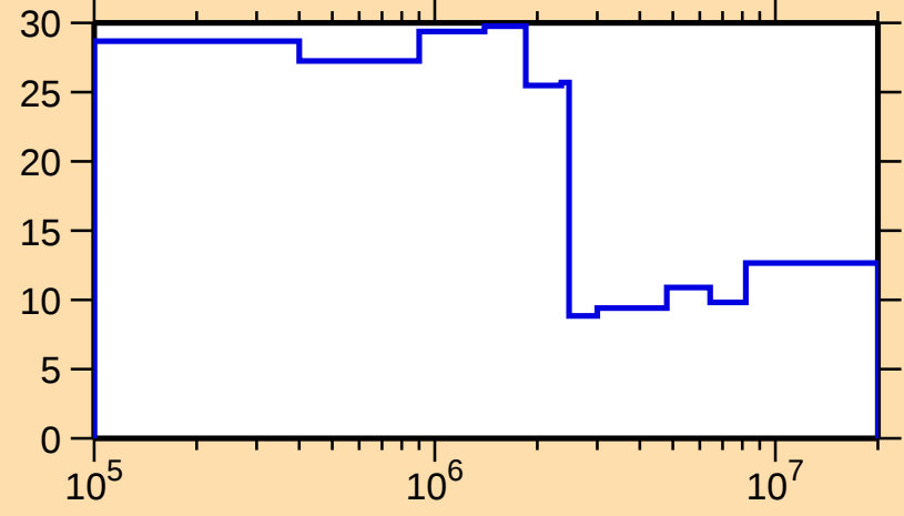
\Delta\sigma/\sigma vs. E for ^{85}\text{Sr}(\text{n,el.})
