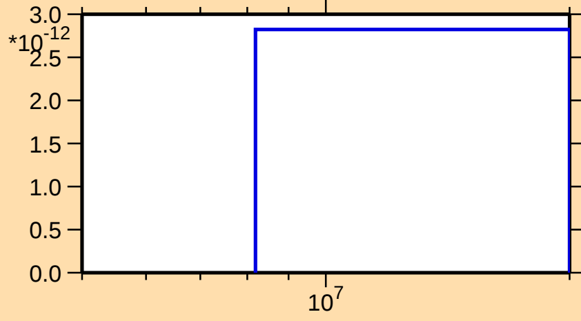
\sigma vs. E for ^{85}\text{Sr}(n,\text{pd})
