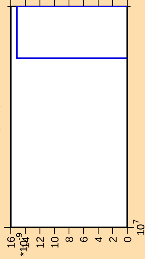
\Delta\sigma/\sigma vs. E for ^{85}\text{Sr}(n,\text{nt})
