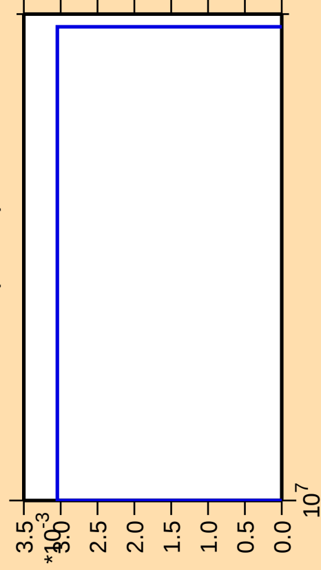
\Delta\sigma/\sigma vs. E for ^{85}\text{Sr}(\text{mt } 34)
