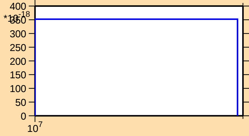
\sigma vs. E for ^{85}\text{Sr}(\text{mt } 34)
