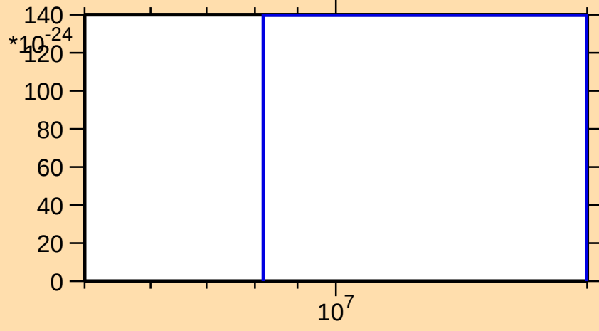
\sigma vs. E for ^{85}\text{Sr}(n,nt)
