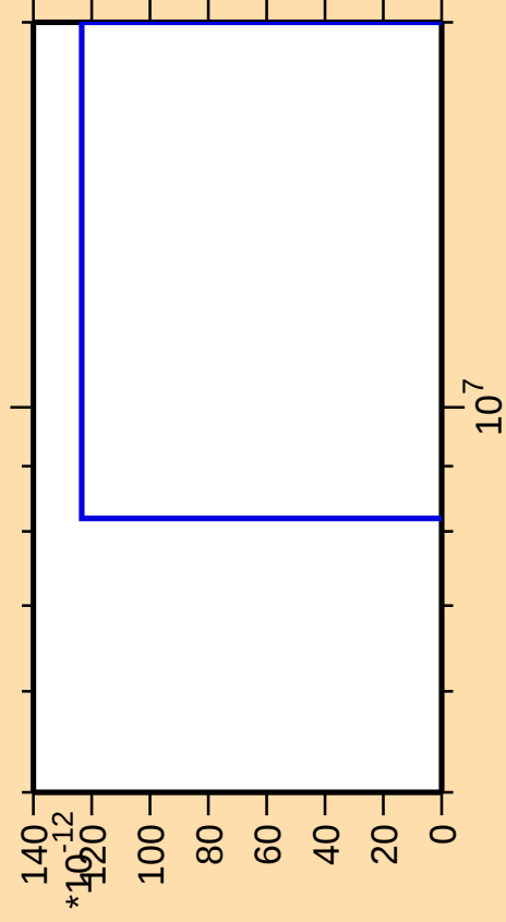
\Delta\sigma/\sigma vs. E for ^{85}\text{Sr}(n,nt)
