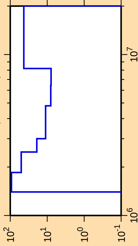
\Delta\sigma/\sigma vs. E for ^{85}\text{Sr}(n,\text{ncont.})
