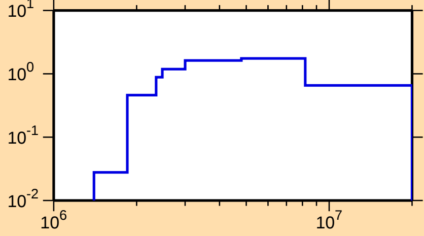
\sigma vs. E for ^{85}\text{Sr}(n,n\text{cont.})
