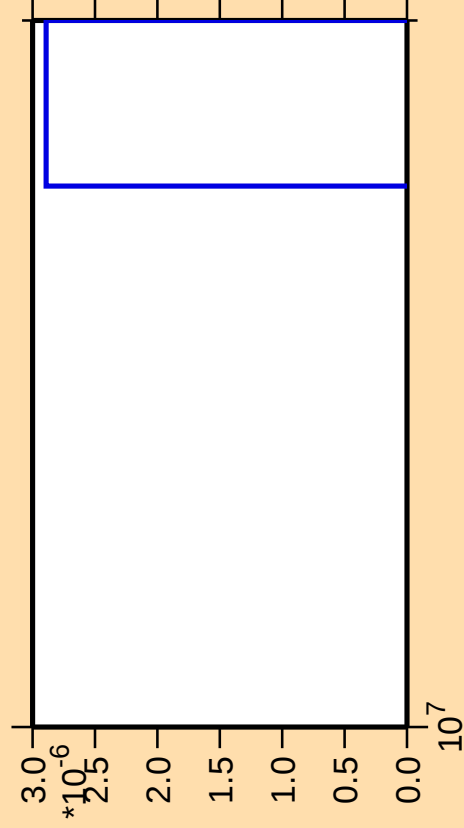
\Delta\sigma/\sigma vs. E for ^{86}\text{Sr}(\text{n},\text{pt})
