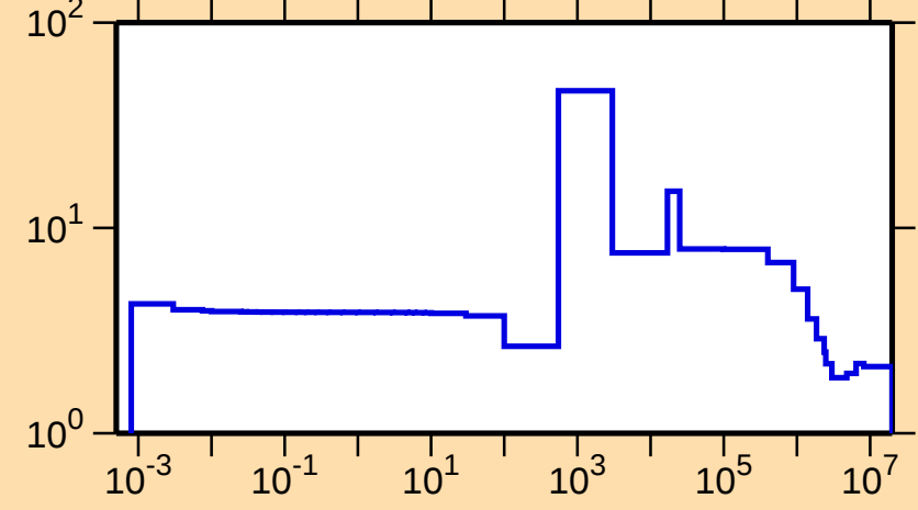
\sigma vs. E for ^{86}\text{Sr}(n,\text{el.})
