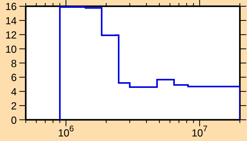
\Delta\sigma/\sigma vs. E for ^{86}\text{Sr}(\text{n,nonel.})
