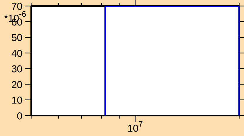
\sigma vs. E for ^{86}\text{Sr}(n,n\alpha)
