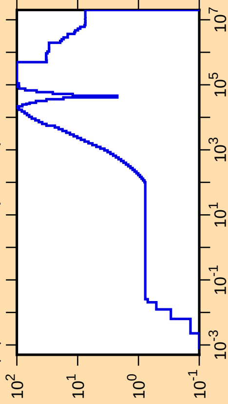
\Delta\mu/\mu vs. E for ^{87}\text{Sr}(\text{mt251})
