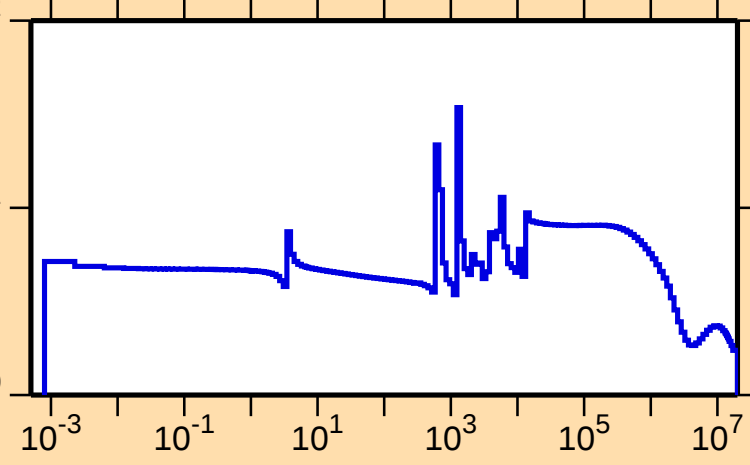
\sigma vs. E for ^{87}\text{Sr}(n,\text{el.})
