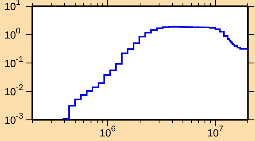
\sigma vs. E for ^{87}\text{Sr}(n,\text{inel.})
