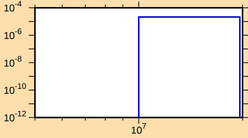
\sigma vs. E for ^{87}\text{Sr}(n,n\alpha)
