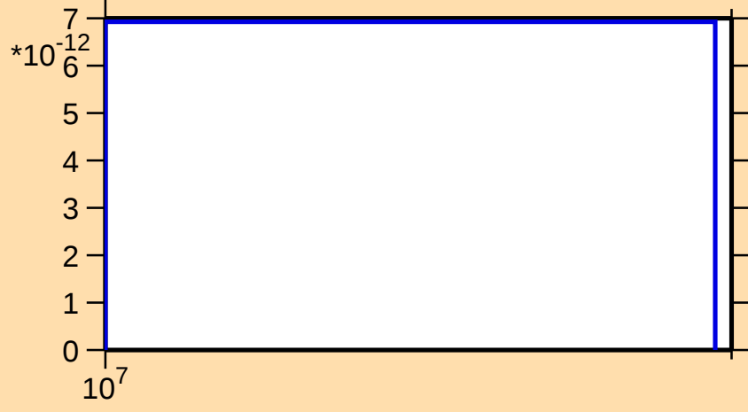
\sigma vs. E for ^{87}\text{Sr}(n,2np)
