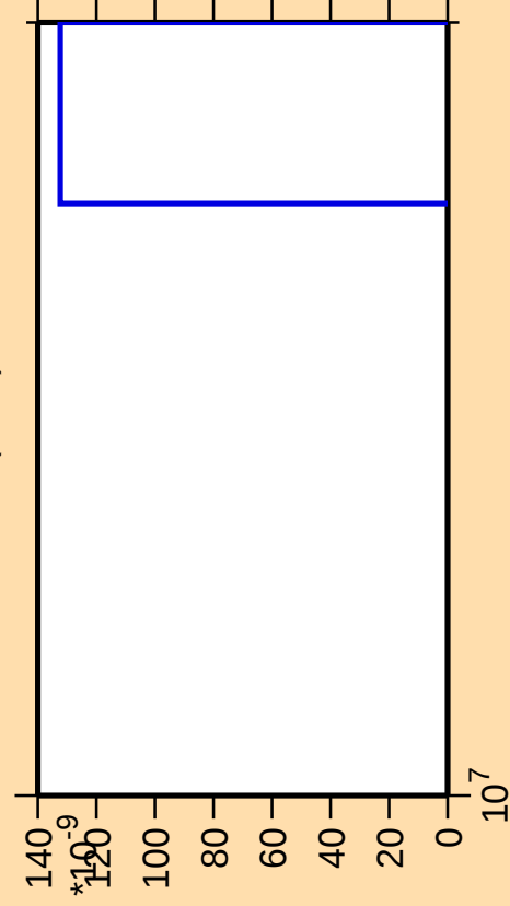
\Delta\sigma/\sigma vs. E for ^{87}\text{Sr}(n,nt)
