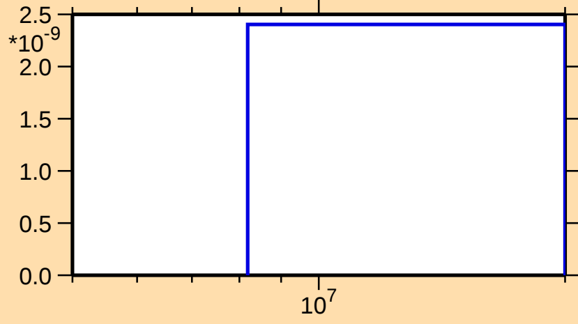
\sigma vs. E for ^{87}\text{Sr}(n,\text{nd})
