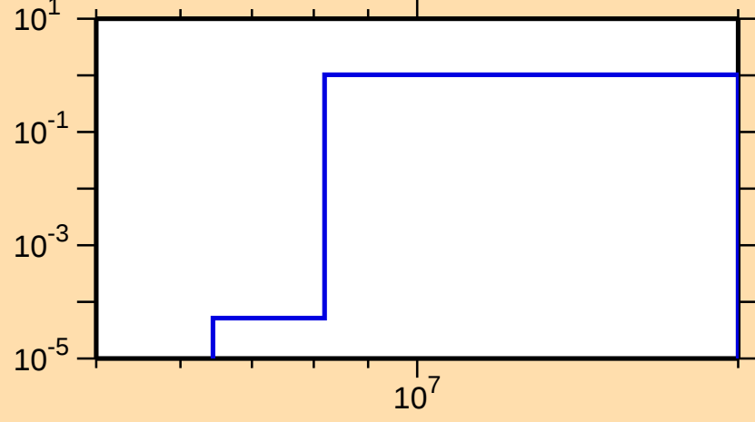
\sigma vs. E for ^{87}\text{Sr}(n,2n)
