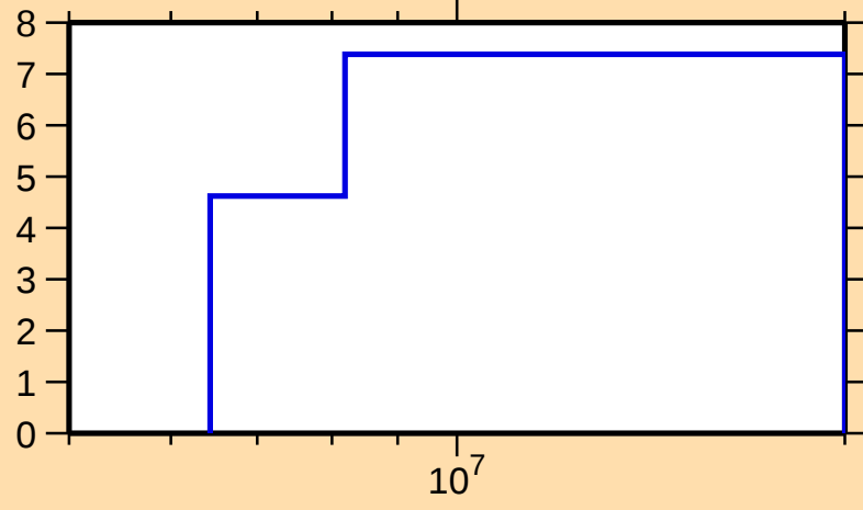
\Delta\sigma/\sigma vs. E for ^{87}\text{Sr}(n,\text{tot.})
