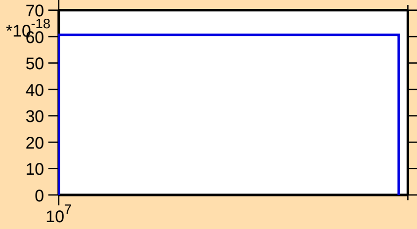
\sigma vs. E for ^{88}\text{Sr}(n,\text{nd})
