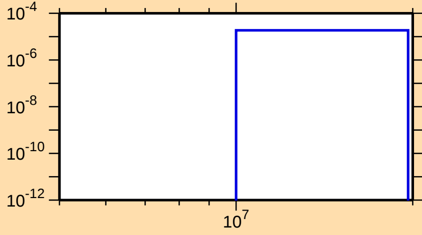
\sigma vs. E for ^{88}\text{Sr}(n,n\alpha)
