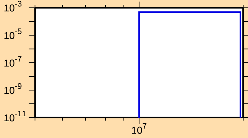
\sigma vs. E for ^{88}\text{Sr}(n,d)
