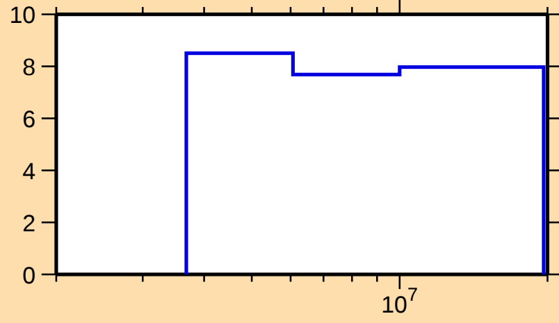
\Delta\sigma/\sigma vs. E for ^{88}\text{Sr}(\text{n},\text{nonel.})
