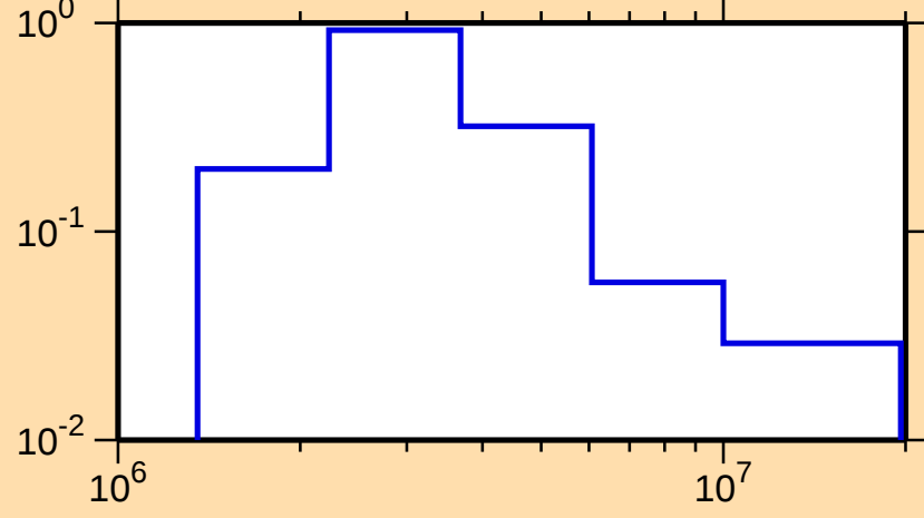
\sigma vs. E for ^{88}\text{Sr}(n,n_1)
