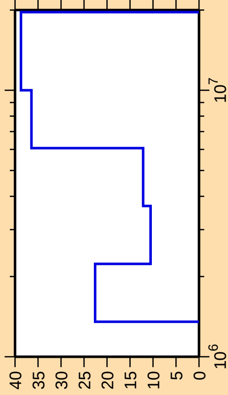
\Delta\sigma/\sigma vs. E for ^{88}\text{Sr}(n,n_1)
