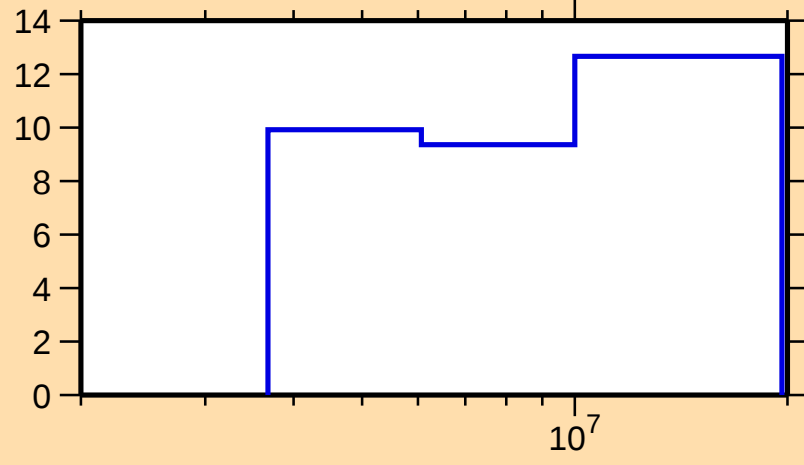
\Delta\sigma/\sigma vs. E for ^{88}\text{Sr}(\text{n},\text{el.})
