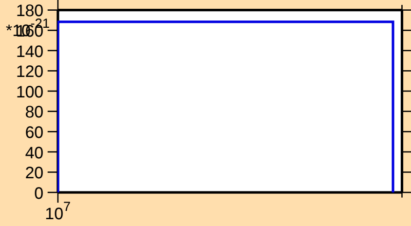
\sigma vs. E for ^{88}\text{Sr}(n,2n\alpha)
