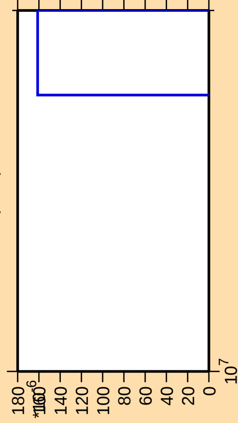
\Delta\sigma/\sigma vs. E for ^{89}\text{Sr}(n,\text{nt})
