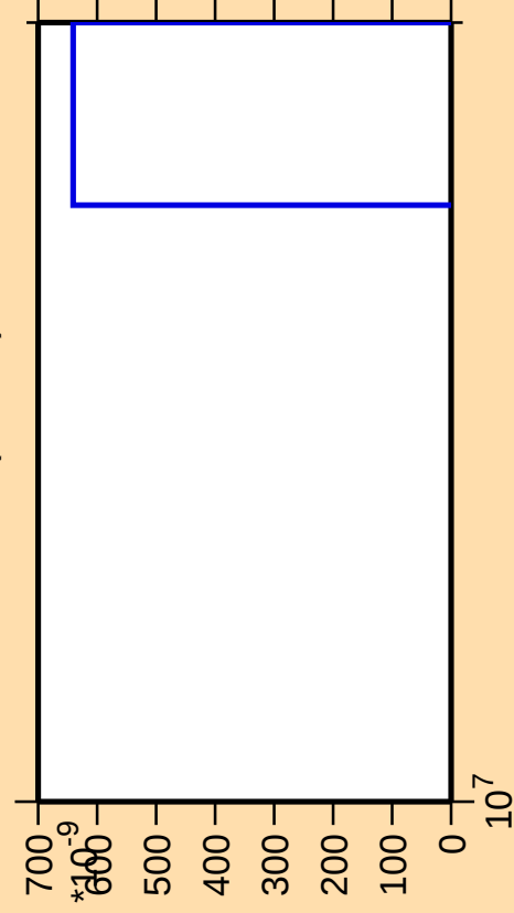
\Delta\sigma/\sigma vs. E for ^{89}\text{Sr}(\text{mt } 34)
