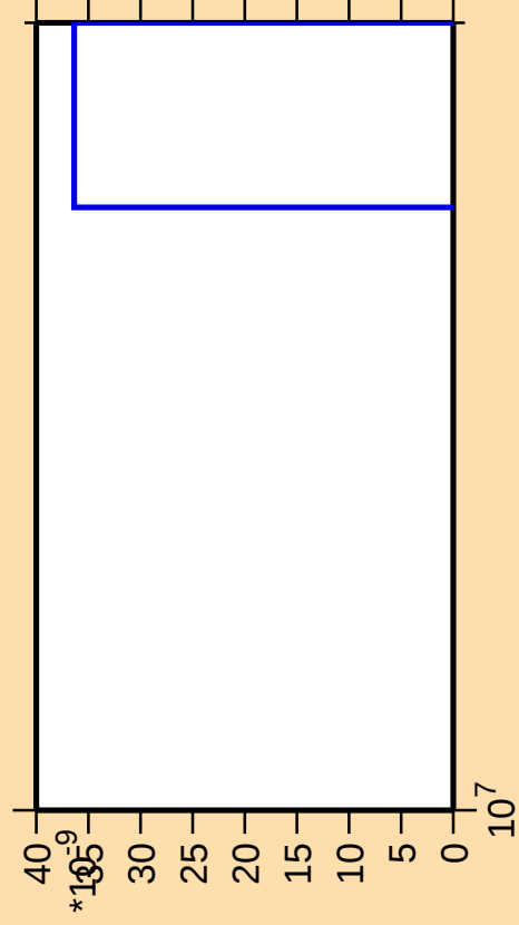
\Delta\sigma/\sigma vs. E for ^{89}\text{Sr}(n,\text{pd})
