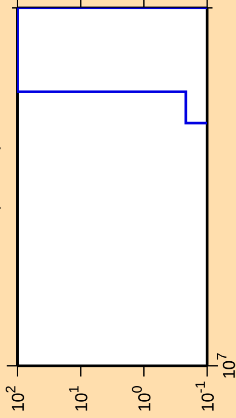
\Delta\sigma/\sigma vs. E for ^{89}\text{Sr}(n,\text{He}3)
