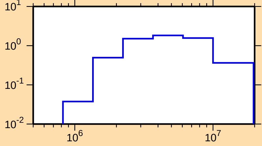
\sigma vs. E for ^{89}\text{Sr}(n,\text{inel.})
