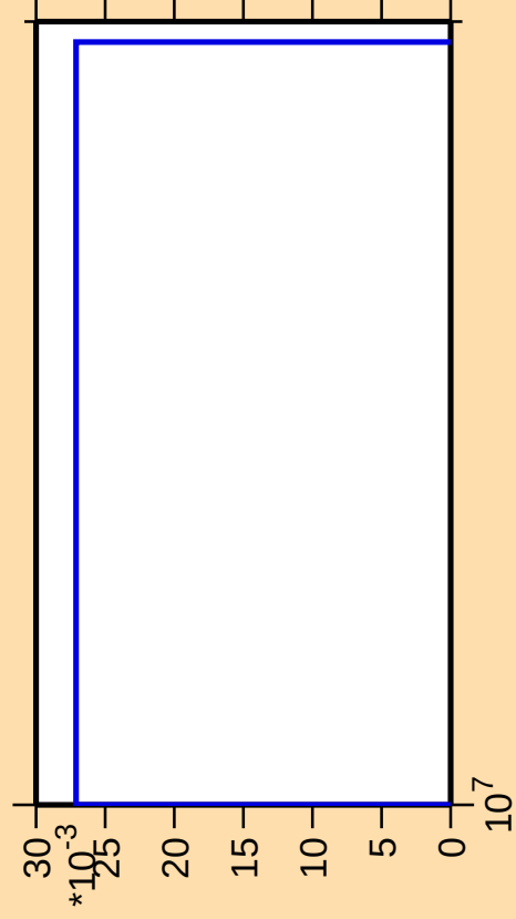
\Delta\sigma/\sigma vs. E for ^{89}\text{Sr}(n,p\alpha)
