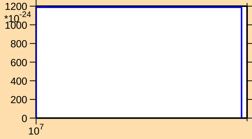
\sigma vs. E for ^{89}\text{Sr}(\text{mt } 34)
