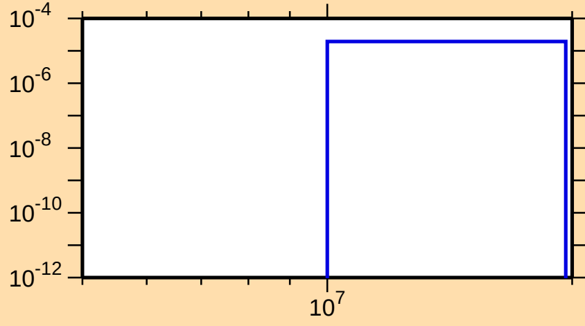
\sigma vs. E for ^{89}\text{Sr}(n,n\alpha)
