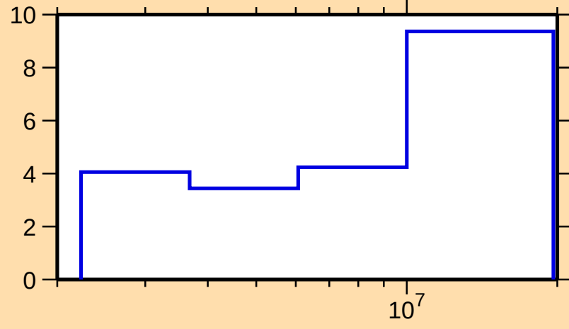
\Delta\sigma/\sigma vs. E for ^{89}\text{Sr}(n,\text{tot.})
