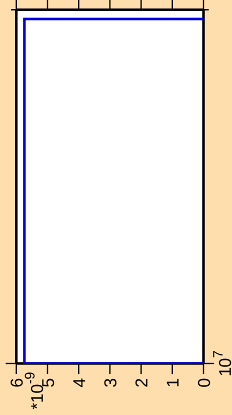
\Delta\sigma/\sigma vs. E for ^{89}\text{Sr}(\text{mt } 34)
