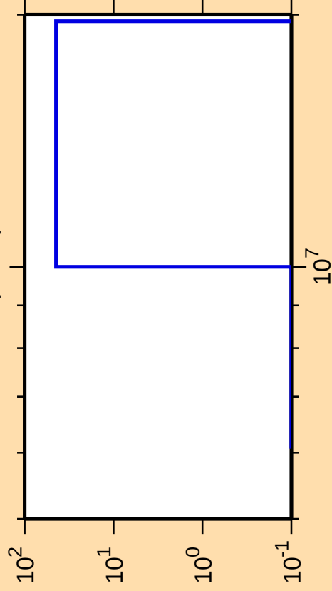
\Delta\sigma/\sigma vs. E for ^{89}\text{Sr}(n,n\alpha)
