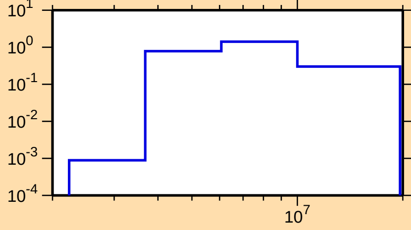
\sigma vs. E for ^{89}\text{Sr}(n,n\text{cont.})
