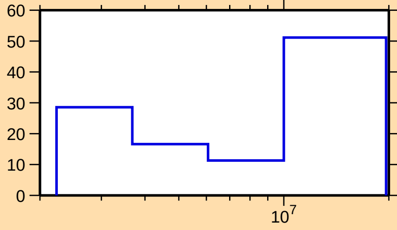
\Delta\sigma/\sigma vs. E for ^{89}\text{Sr}(n,n\text{cont.})
