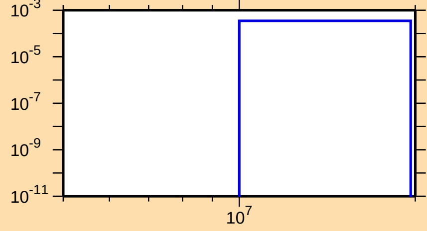
\sigma vs. E for ^{89}\text{Sr}(n,d)
