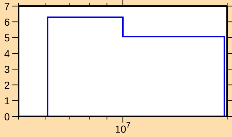
\Delta\sigma/\sigma vs. E for ^{89}\text{Sr}(n,\text{nonel.})
