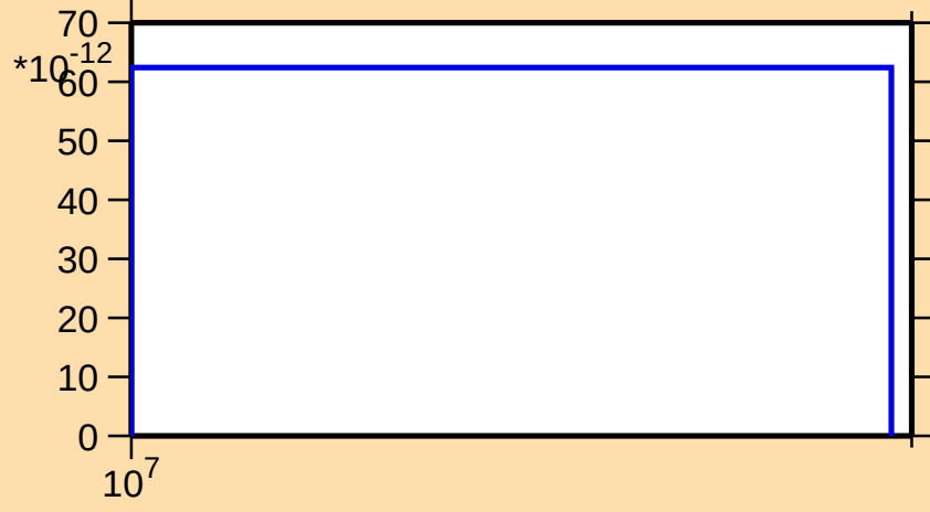
\sigma vs. E for ^{89}\text{Sr}(n,2np)
