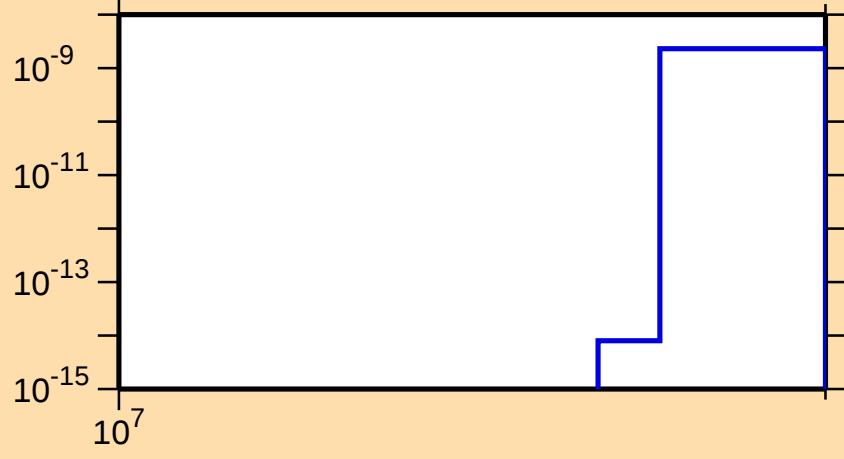
\sigma vs. E for ^{90}\text{Sr}(n,\text{nt})
