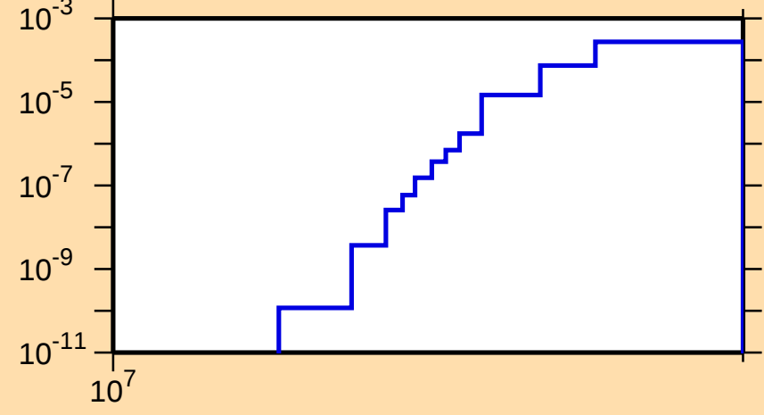
\sigma vs. E for ^{90}\text{Sr}(n,t)
