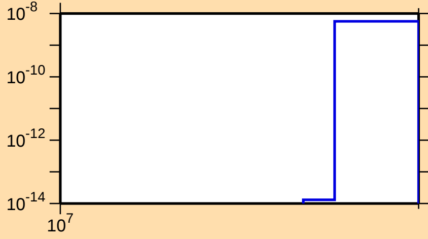
\sigma vs. E for ^{90}\text{Sr}(n,\text{nd})
