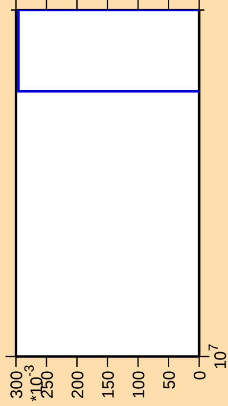
\Delta\sigma/\sigma vs. E for ^{90}\text{Sr}(n,2np)
