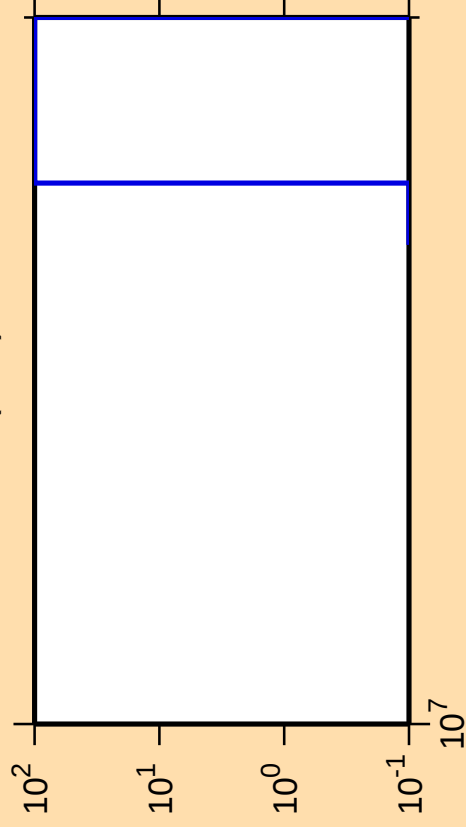
\Delta\sigma/\sigma vs. E for ^{90}\text{Sr}(n,\text{nt})
