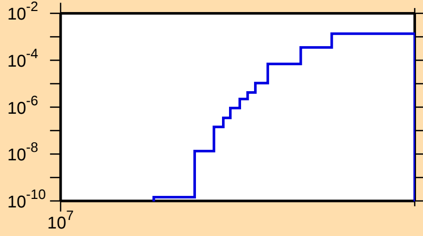
\sigma vs. E for ^{90}\text{Sr}(n,np)
