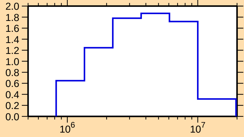
\sigma vs. E for ^{90}\text{Sr}(\text{n,inel.})
