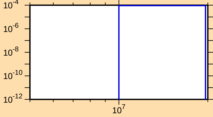
\sigma vs. E for ^{90}\text{Sr}(n,d)
