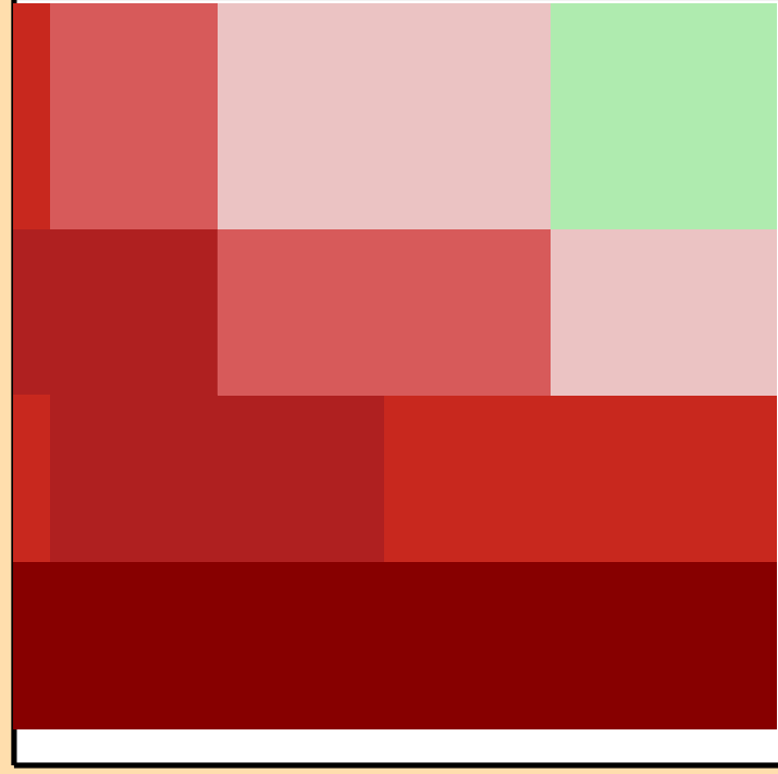
\Delta\sigma/\sigma vs. E for ^{90}\text{Sr}(n,\text{nonel.})
