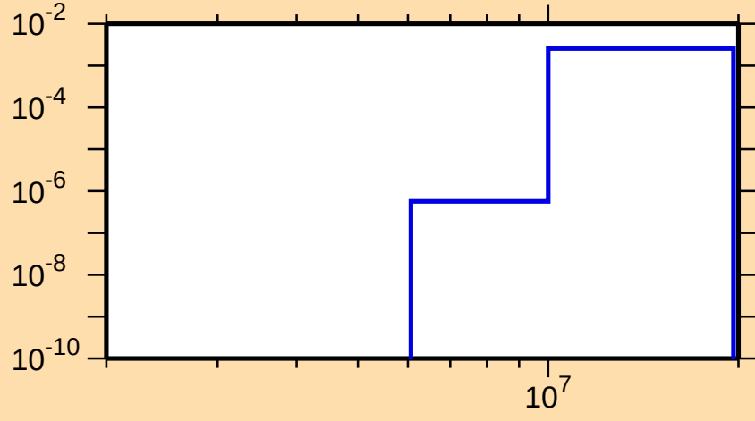
\sigma vs. E for ^{90}\text{Sr}(n,p)
