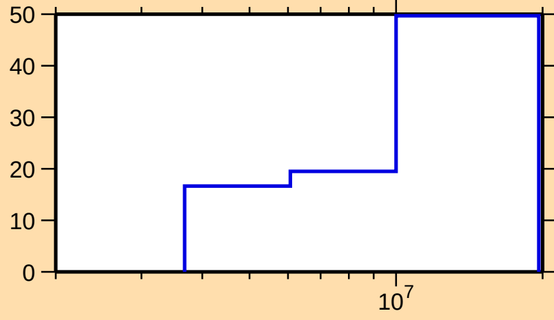
\Delta\sigma/\sigma vs. E for ^{90}\text{Sr}(n,n\text{cont.})
