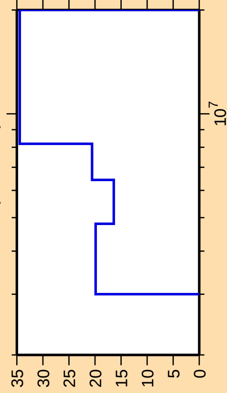
\Delta\sigma/\sigma vs. E for ^{90}\text{Sr}(n,n\text{cont.})
