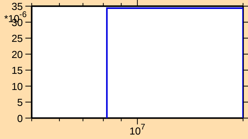
\sigma vs. E for ^{90}\text{Sr}(n,np)
