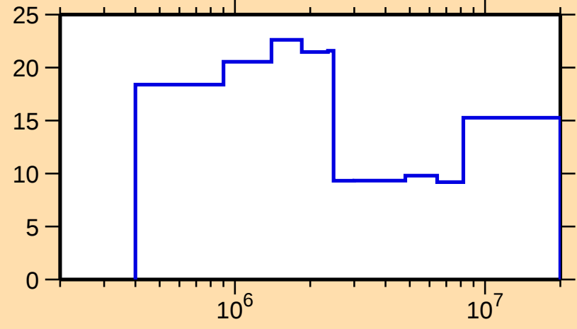
\Delta\sigma/\sigma vs. E for ^{90}\text{Sr}(\text{n,el.})
