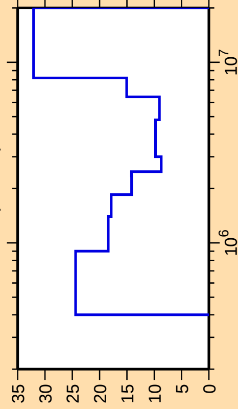
\Delta\sigma/\sigma vs. E for ^{90}\text{Sr}(\text{n,inel.})
