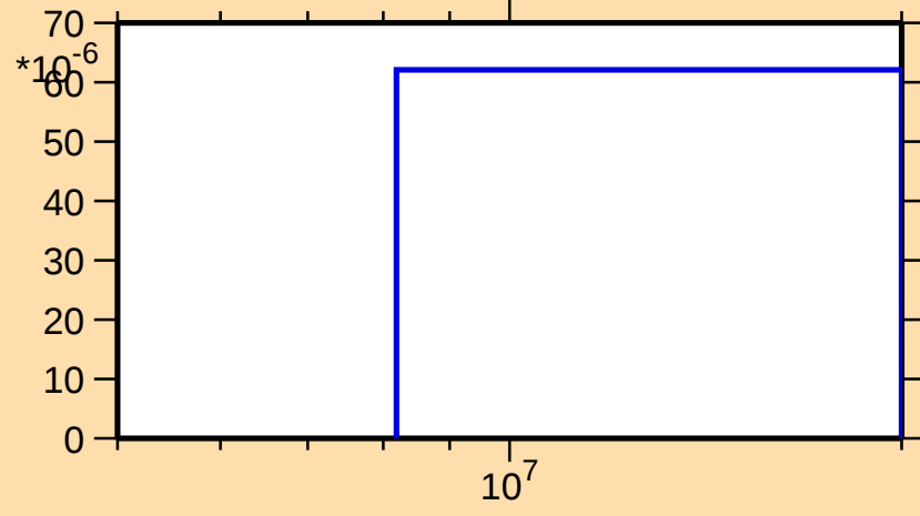
\sigma vs. E for ^{90}\text{Sr}(n,n\alpha)
