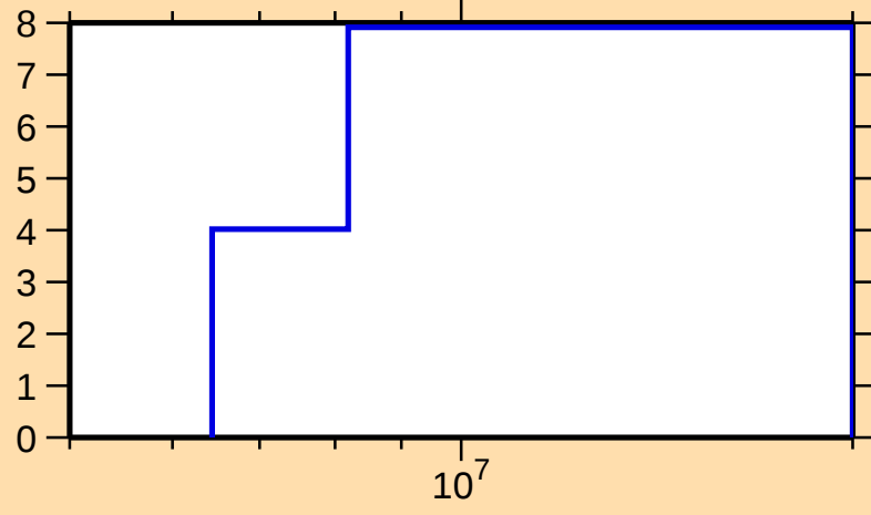
\Delta\sigma/\sigma vs. E for ^{90}\text{Sr}(n,\text{tot.})
