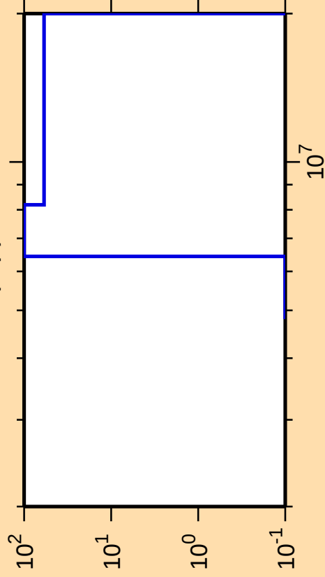
\Delta\sigma/\sigma vs. E for ^{90}\text{Sr}(n,p)
