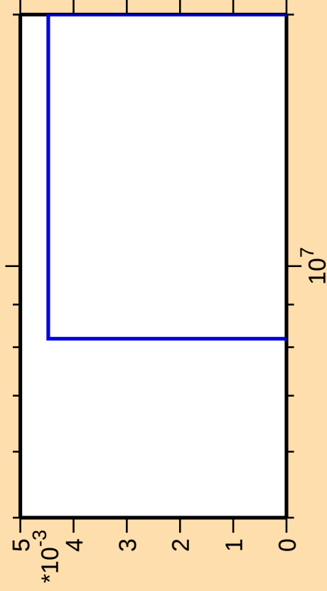
\Delta\sigma/\sigma vs. E for ^{90}\text{Sr}(n,2n\alpha)
