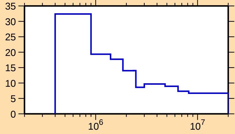
\Delta\sigma/\sigma vs. E for ^{90}\text{Sr}(\text{n,nonel.})
