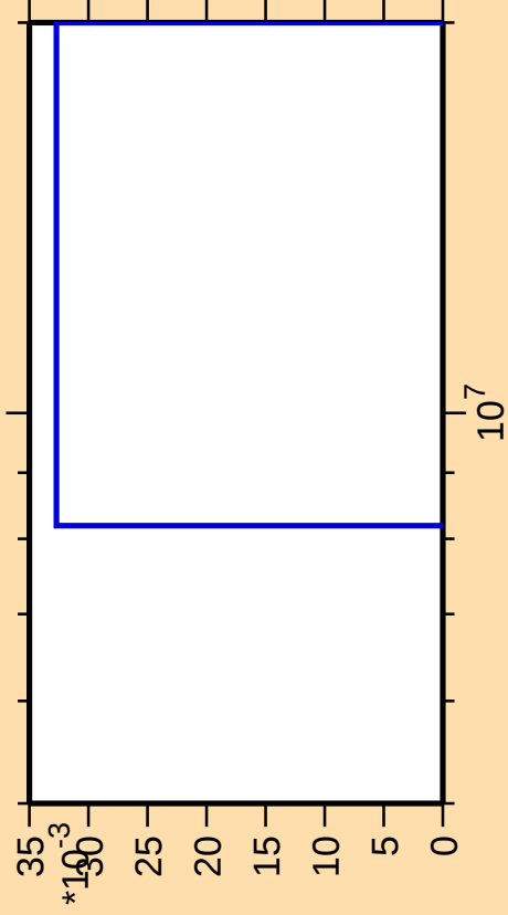
\Delta\sigma/\sigma vs. E for ^{90}\text{Sr}(n,\text{He}3)
