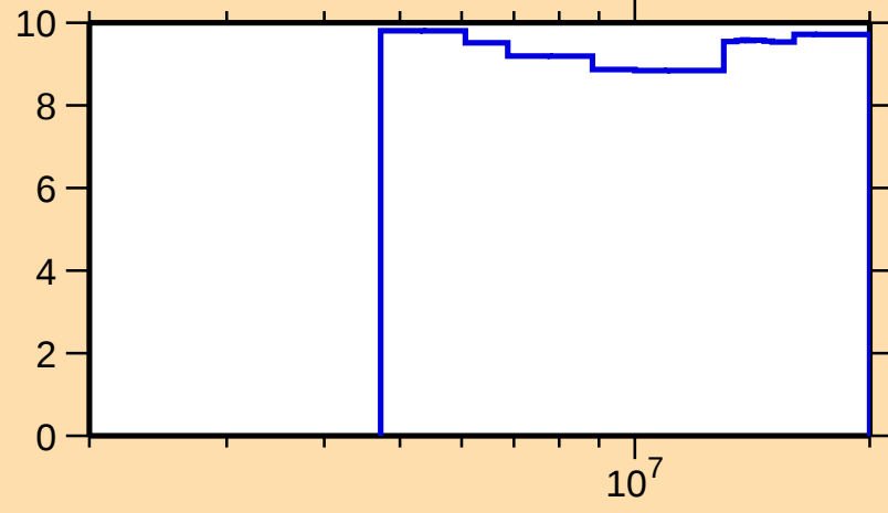
\Delta\sigma/\sigma vs. E for ^{91}\text{Sr}(n,\text{nonel.})
