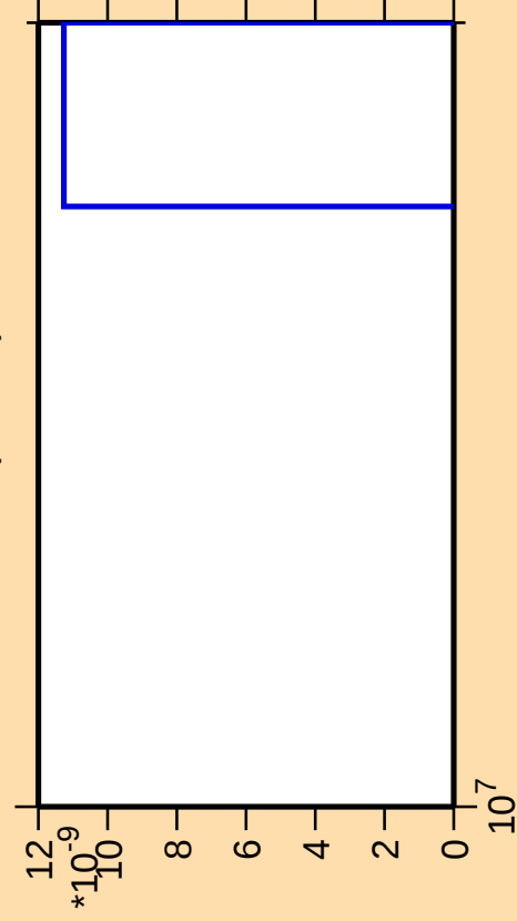
\Delta\sigma/\sigma vs. E for ^{91}\text{Sr}(\text{mt } 34)
