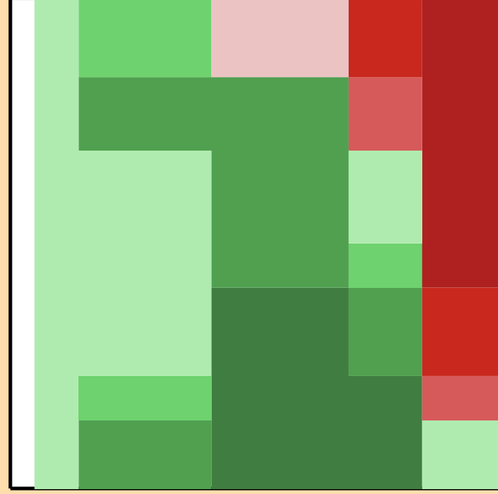
\Delta\sigma/\sigma vs. E for ^{91}\text{Sr}(n,2n)
