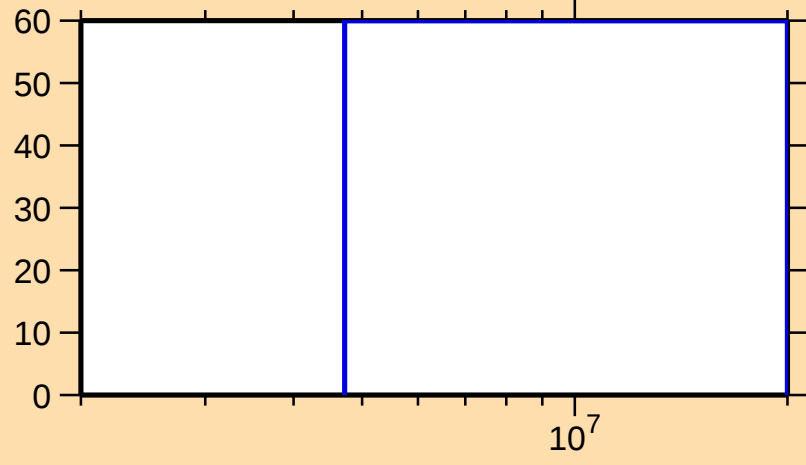
\Delta\sigma/\sigma vs. E for ^{91}\text{Sr}(n,\gamma)
