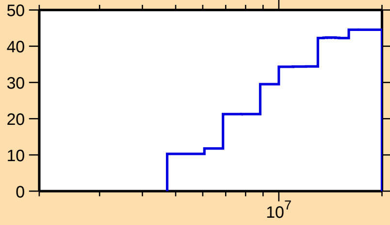
\Delta\sigma/\sigma vs. E for ^{91}\text{Sr}(n,\text{inel.})
