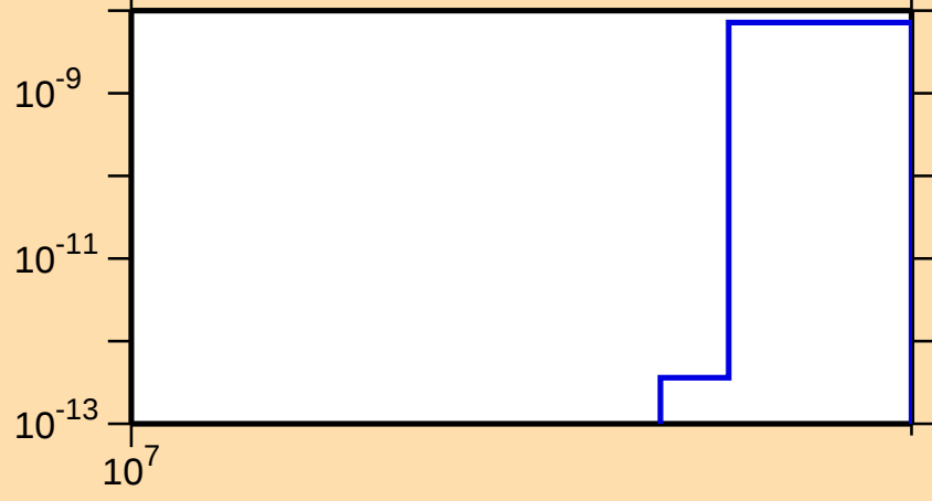
\sigma vs. E for ^{91}\text{Sr}(n,\text{nt})
