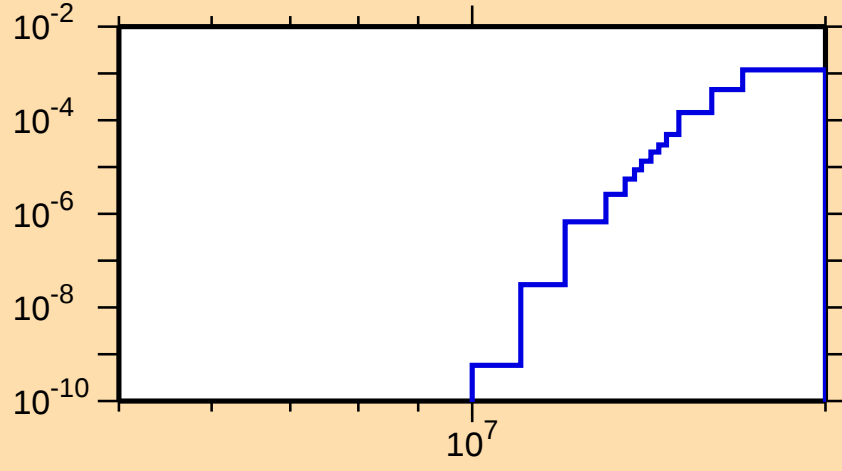
\sigma vs. E for ^{91}\text{Sr}(n,n\alpha)
