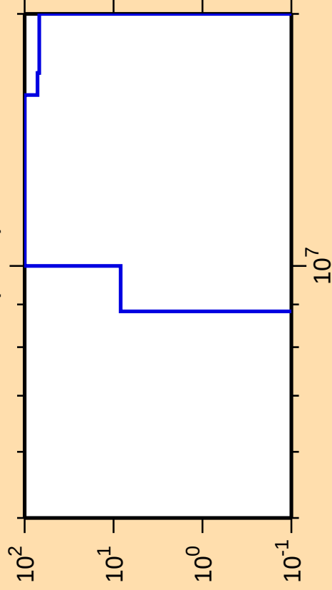
\Delta\sigma/\sigma vs. E for ^{91}\text{Sr}(n,n\alpha)
