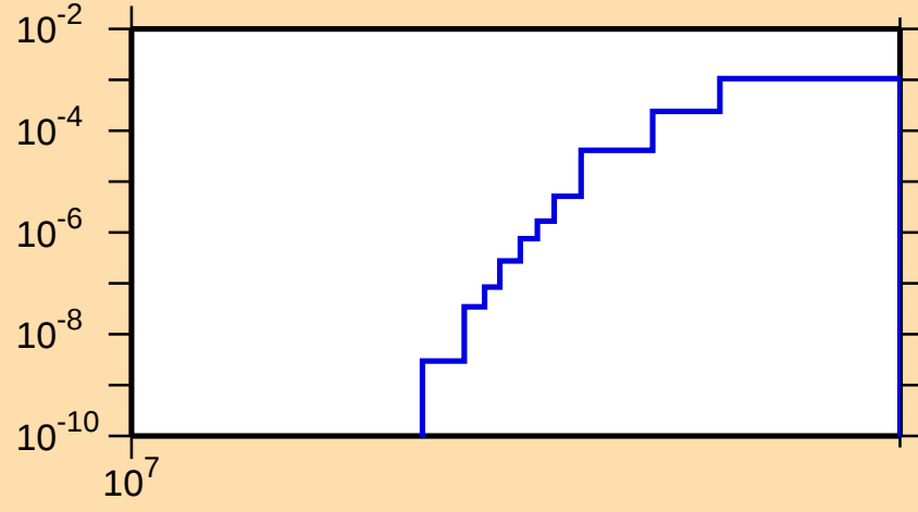
\sigma vs. E for ^{91}\text{Sr}(n,np)
