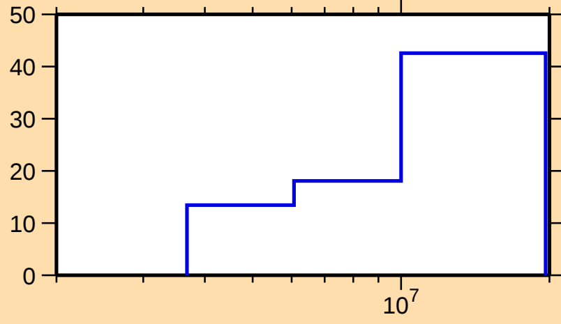
\Delta\sigma/\sigma vs. E for ^{91}\text{Sr}(n,n\text{cont.})
