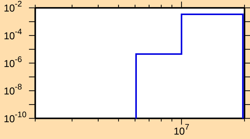
\sigma vs. E for ^{91}\text{Sr}(n,p)
