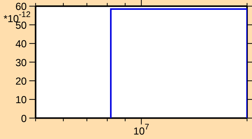
\sigma vs. E for ^{91}\text{Sr}(n,nt)
