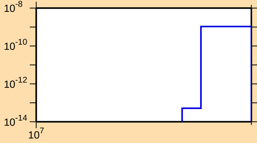
\sigma vs. E for ^{92}\text{Sr}(n,2n\alpha)
