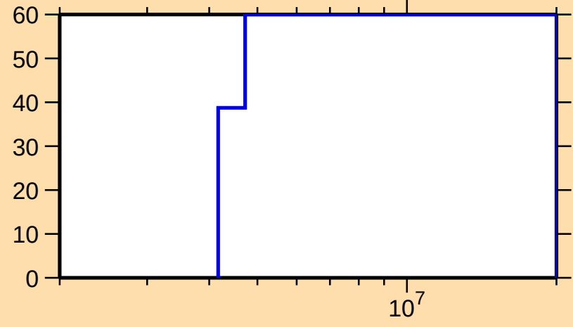
\Delta\sigma/\sigma vs. E for ^{92}\text{Sr}(n,n_1)
