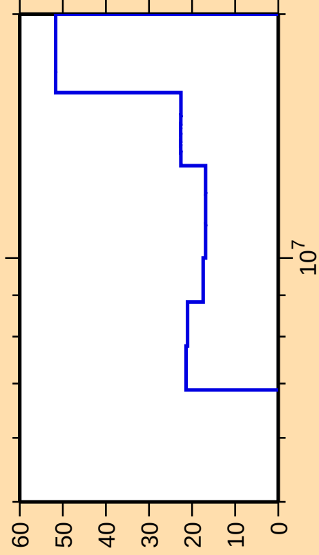
\Delta\sigma/\sigma vs. E for ^{92}\text{Sr}(n,2n)
