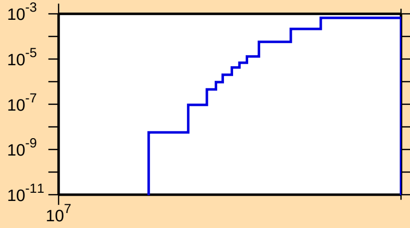
\sigma vs. E for ^{92}\text{Sr}(n,d)
