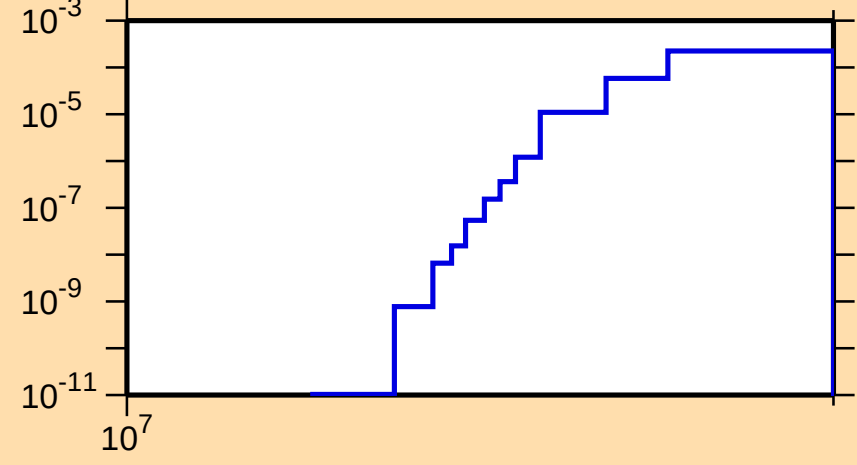
\sigma vs. E for ^{92}\text{Sr}(n,t)
