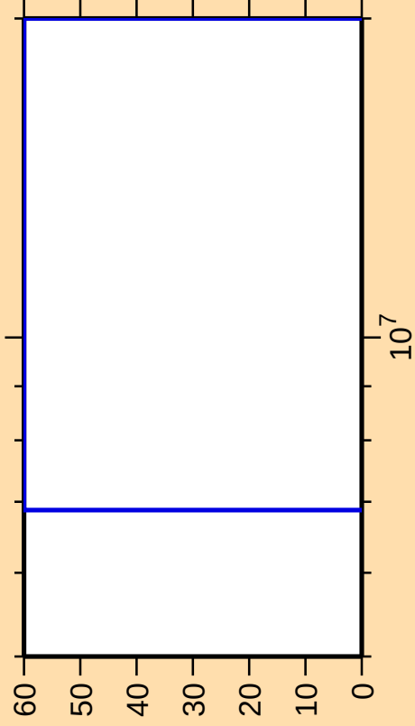
\Delta\sigma/\sigma vs. E for ^{92}\text{Sr}(n,n_1)
