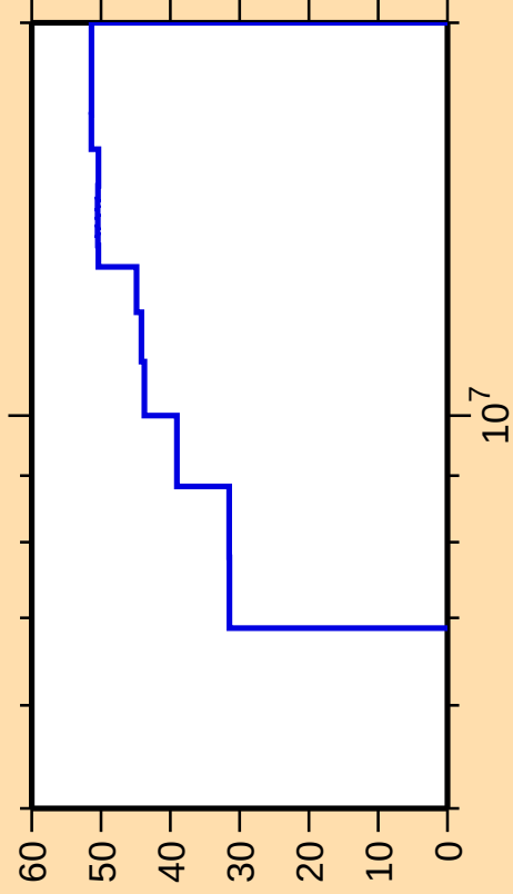
\Delta\sigma/\sigma vs. E for ^{92}\text{Sr}(n,n\text{cont.})
