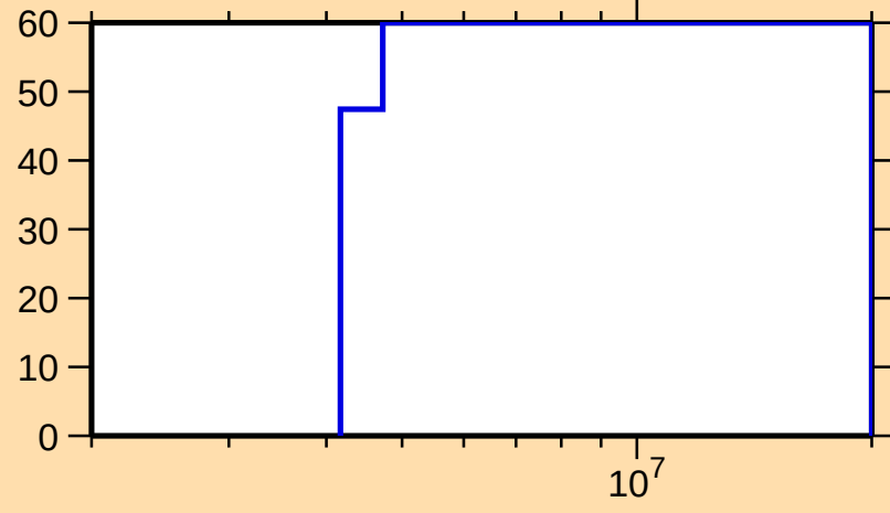
\Delta\sigma/\sigma vs. E for ^{92}\text{Sr}(n,\gamma)
