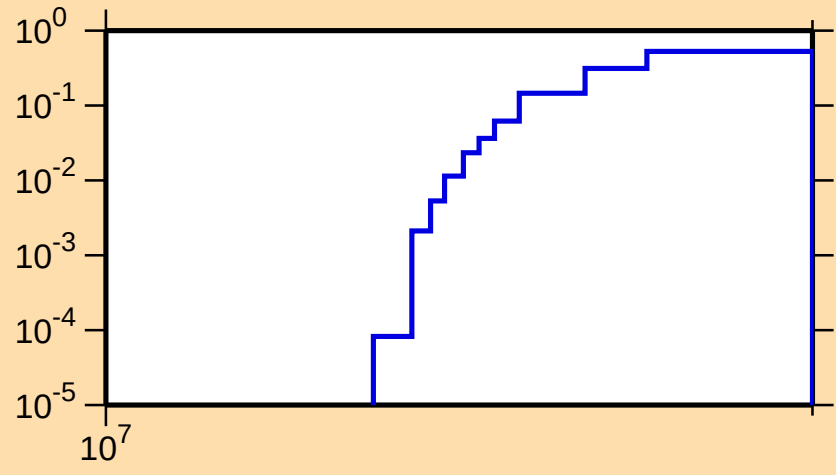
\sigma vs. E for ^{92}\text{Sr}(n,3n)
