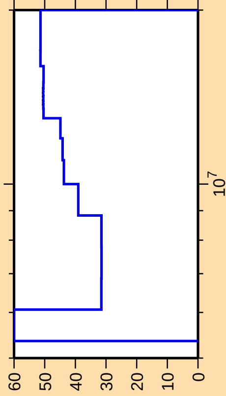
\Delta\sigma/\sigma vs. E for ^{92}\text{Sr}(n,\text{ncont.})
