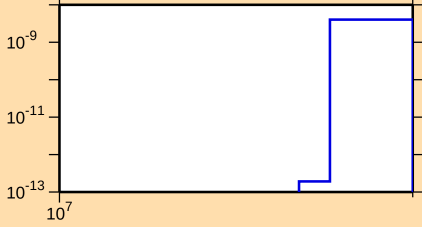
\sigma vs. E for ^{92}\text{Sr}(n,\text{nt})
