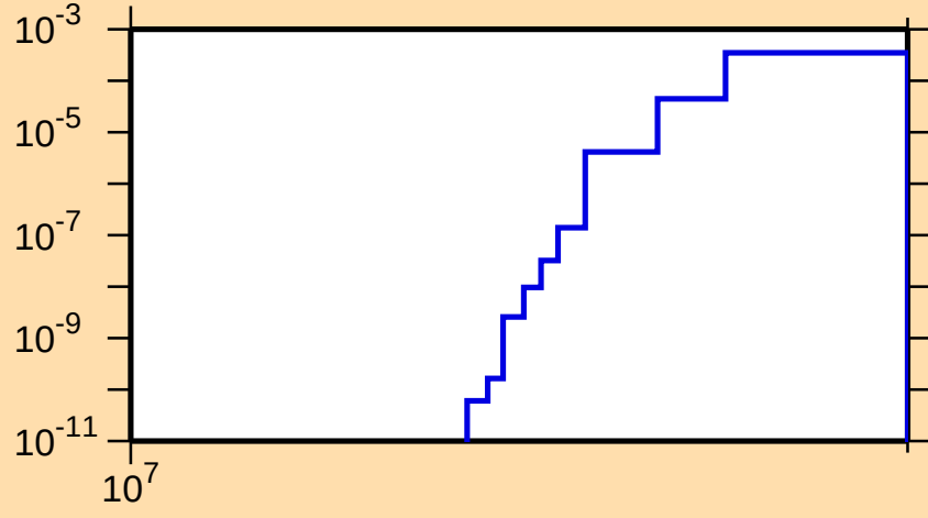
\sigma vs. E for ^{92}\text{Sr}(n,np)
