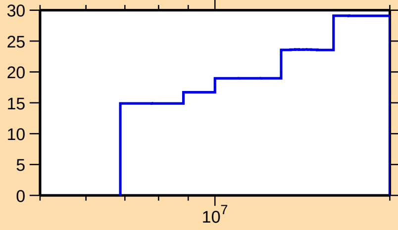
\Delta\sigma/\sigma vs. E for ^{92}\text{Sr}(n,\text{el.})
