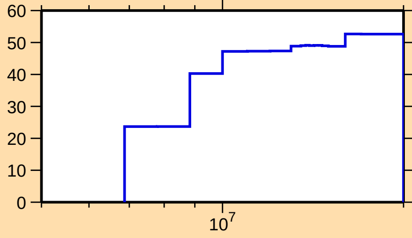
\Delta\sigma/\sigma vs. E for ^{92}\text{Sr}(n,\text{inel.})
