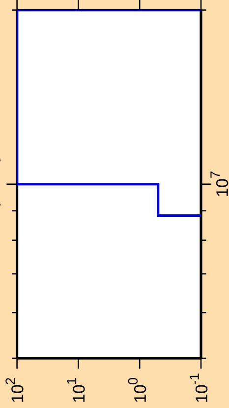
\Delta\sigma/\sigma vs. E for ^{92}\text{Sr}(n,n\alpha)
