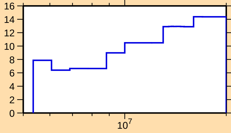
\Delta\sigma/\sigma vs. E for ^{92}\text{Sr}(n,\text{tot.})
