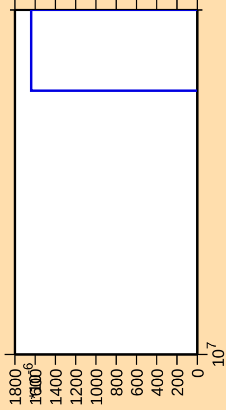
\Delta\sigma/\sigma vs. E for ^{92}\text{Sr}(n,2np)
