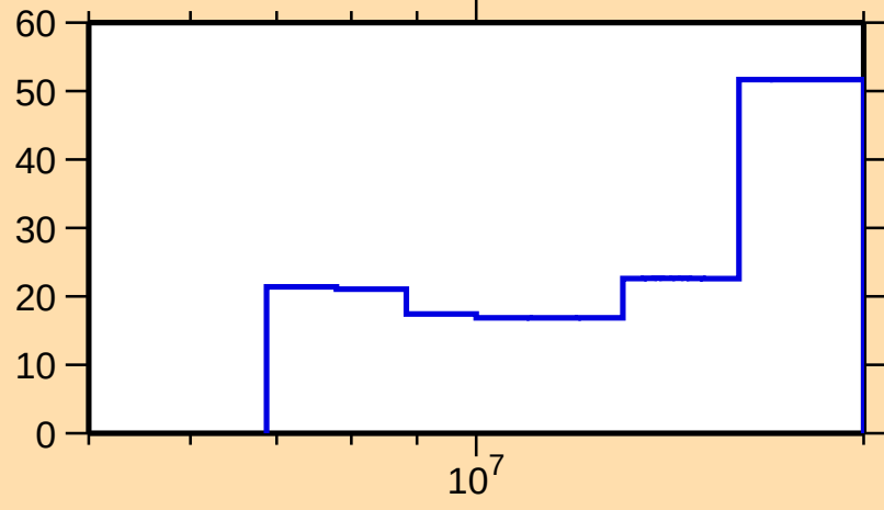
\Delta\sigma/\sigma vs. E for ^{92}\text{Sr}(n,2n)
