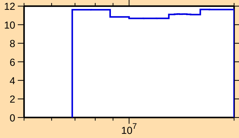
\Delta\sigma/\sigma vs. E for ^{92}\text{Sr}(n,\text{nonel.})
