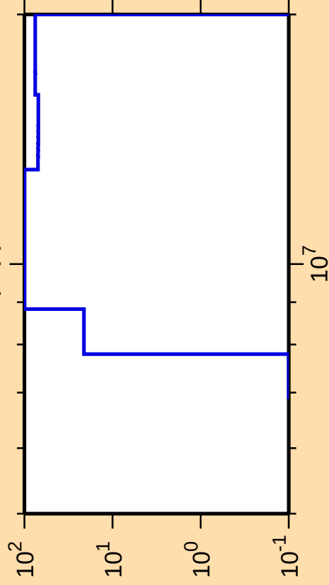
\Delta\sigma/\sigma vs. E for ^{92}\text{Sr}(n,p)
