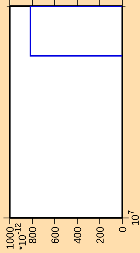
\Delta\sigma/\sigma vs. E for ^{92}\text{Sr}(n,3n\alpha)
