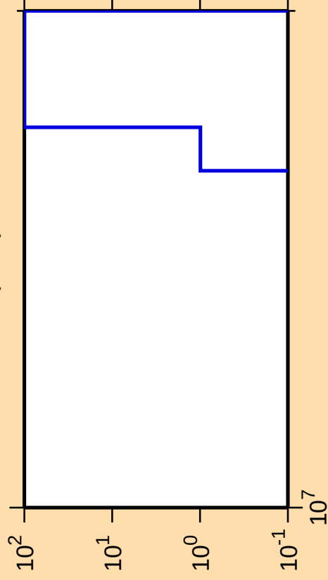
\Delta\sigma/\sigma vs. E for ^{92}\text{Sr}(n,\text{nt})
