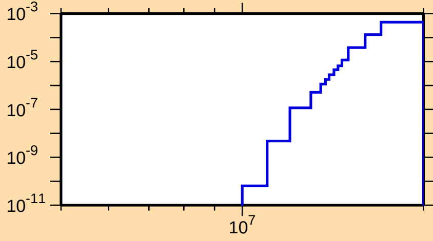
\sigma vs. E for ^{92}\text{Sr}(n,n\alpha)
