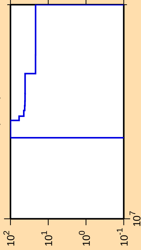
\Delta\sigma/\sigma vs. E for ^{92}\text{Sr}(n,3n)
