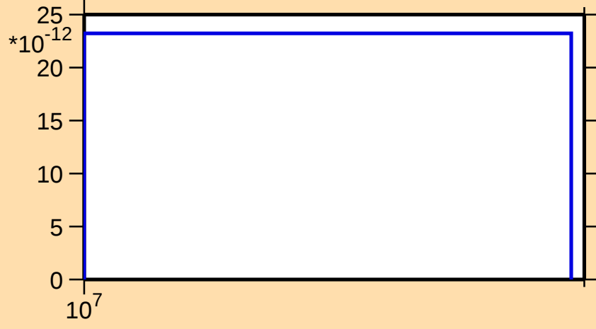
\sigma vs. E for ^{92}\text{Sr}(n,\text{nt})
