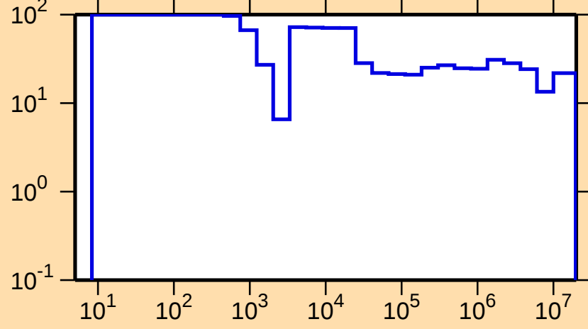
\Delta\sigma/\sigma vs. E for ^{92}\text{Sr}(n,\text{el.})
