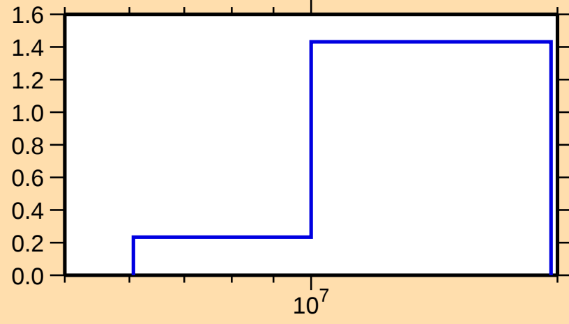
\sigma vs. E for ^{92}\text{Sr}(n,2n)
