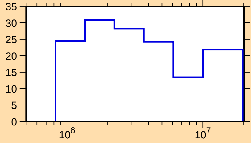
\Delta\sigma/\sigma vs. E for ^{92}\text{Sr}(\text{n,el.})
