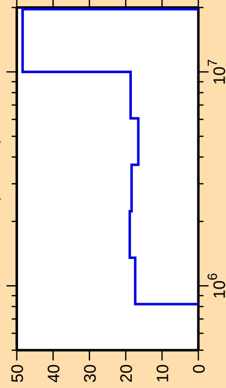
\Delta\sigma/\sigma vs. E for ^{92}\text{Sr}(\text{n,inel.})
