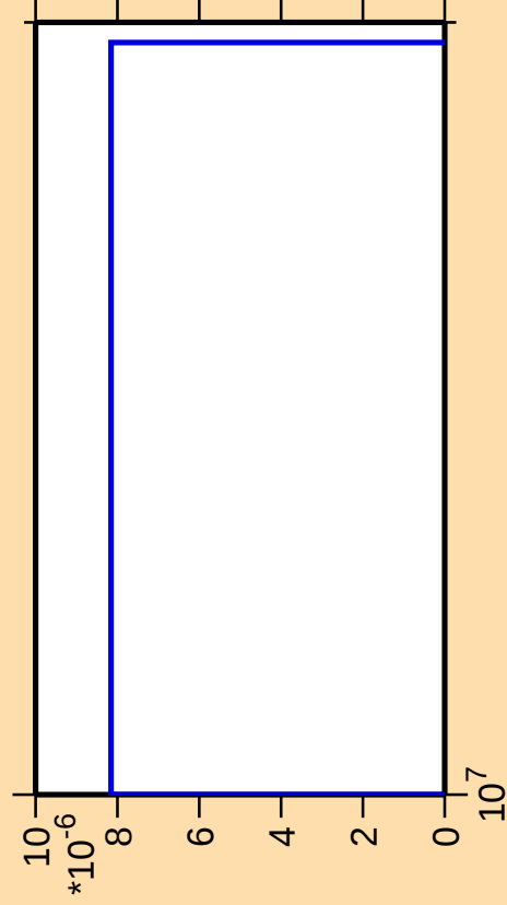
\Delta\sigma/\sigma vs. E for ^{92}\text{Sr}(n,2np)
