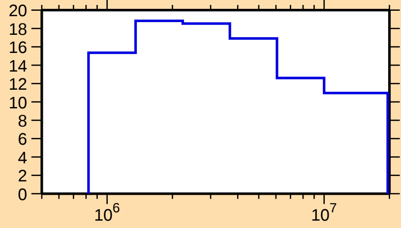
\Delta\sigma/\sigma vs. E for ^{92}\text{Sr}(\text{n,nonel.})
