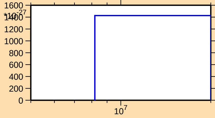
\sigma vs. E for ^{92}\text{Sr}(n,3n\alpha)
