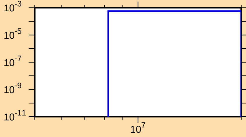
\sigma vs. E for ^{92}\text{Sr}(n,p)
