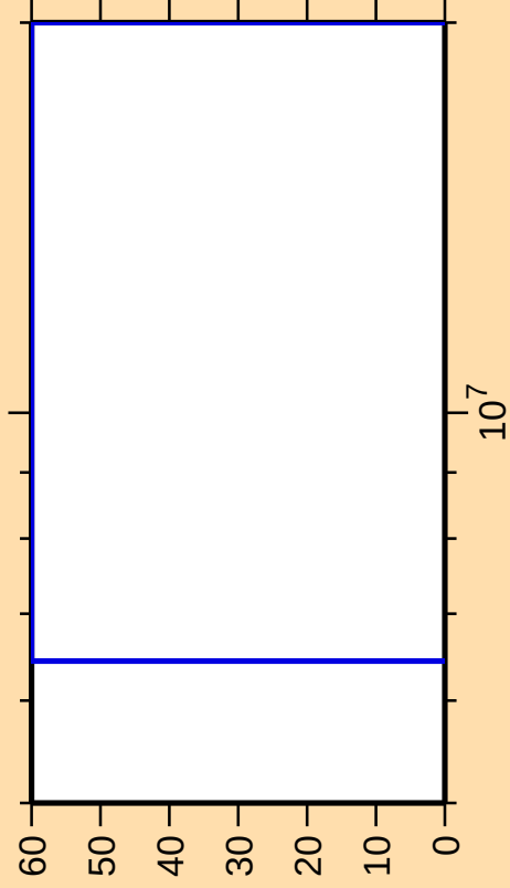
\Delta\sigma/\sigma vs. E for ^{92}\text{Sr}(n,\gamma)
