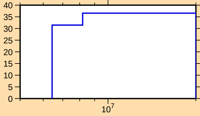
\Delta\sigma/\sigma vs. E for ^{92}\text{Sr}(n,n\text{cont.})
