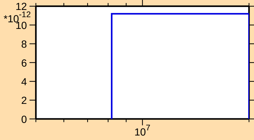
\sigma vs. E for ^{92}\text{Sr}(n,\text{nd})
