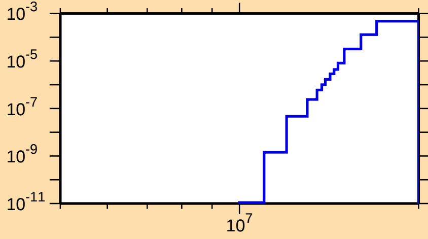
\sigma vs. E for ^{93}\text{Sr}(n,n\alpha)
