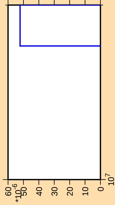
\Delta\sigma/\sigma vs. E for ^{93}\text{Sr}(n,3n\alpha)
