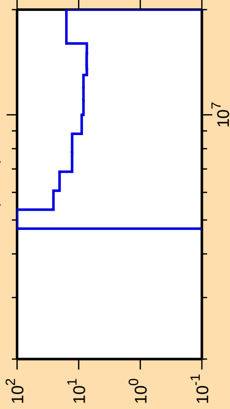
\Delta\sigma/\sigma vs. E for ^{93}\text{Sr}(n,2n)
