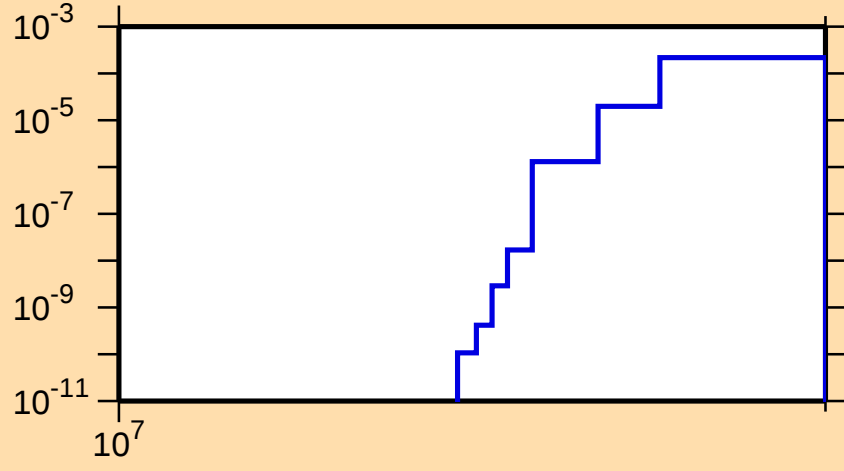
\sigma vs. E for ^{93}\text{Sr}(n,np)
