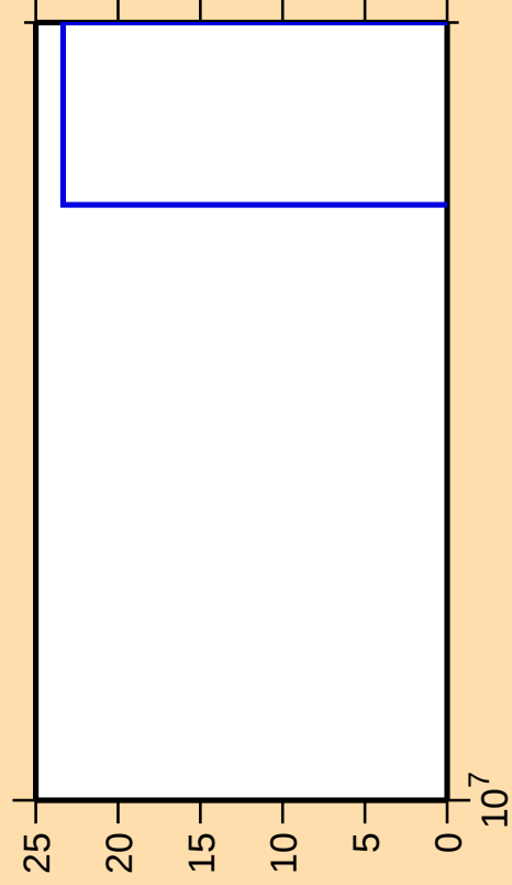
\Delta\sigma/\sigma vs. E for ^{93}\text{Sr}(n,2np)
