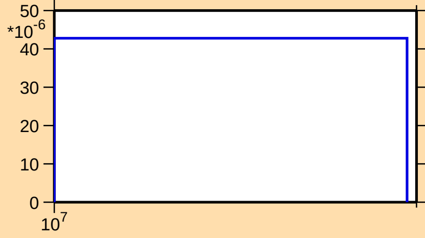
\sigma vs. E for ^{93}\text{Sr}(n,d)
