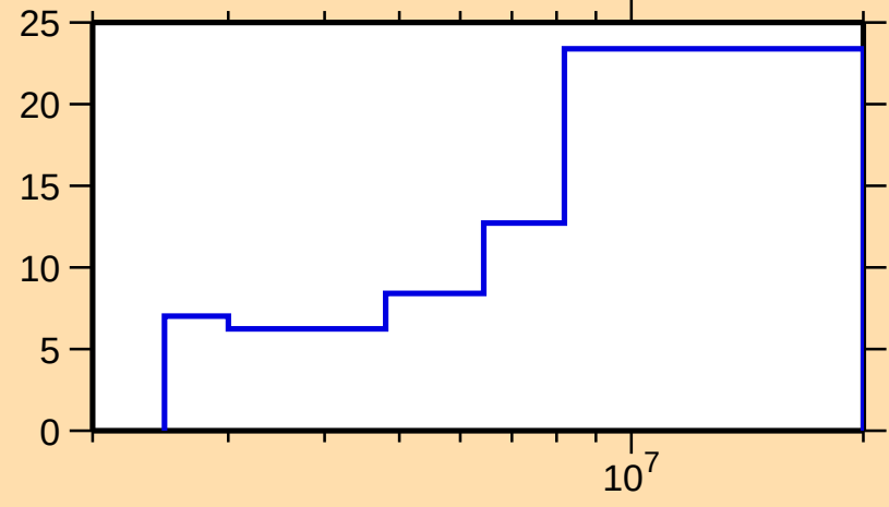
\Delta\sigma/\sigma vs. E for ^{93}\text{Sr}(n,\text{inel.})
