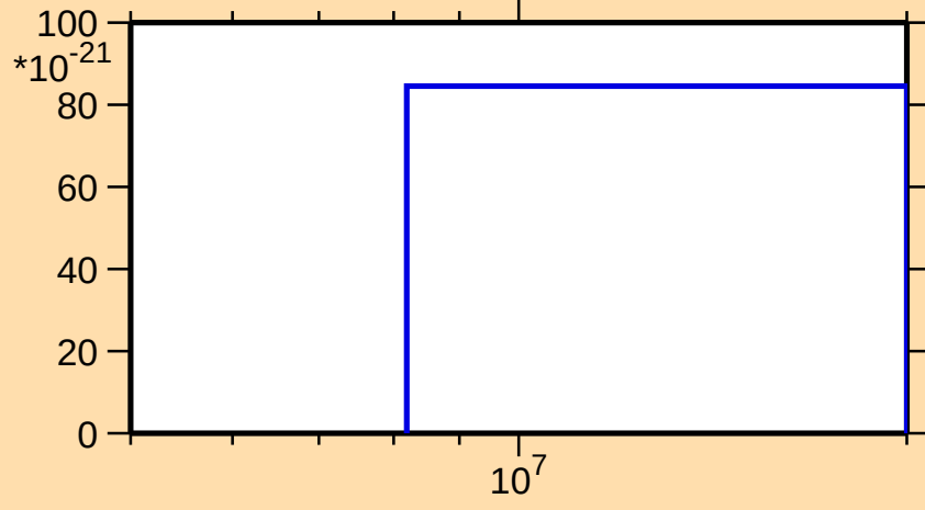
\sigma vs. E for ^{93}\text{Sr}(n,3n\alpha)
