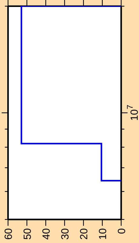
\Delta\sigma/\sigma vs. E for ^{93}\text{Sr}(n,p)
