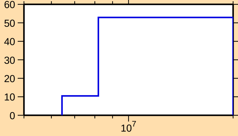
\Delta\sigma/\sigma vs. E for ^{93}\text{Sr}(n,p)
