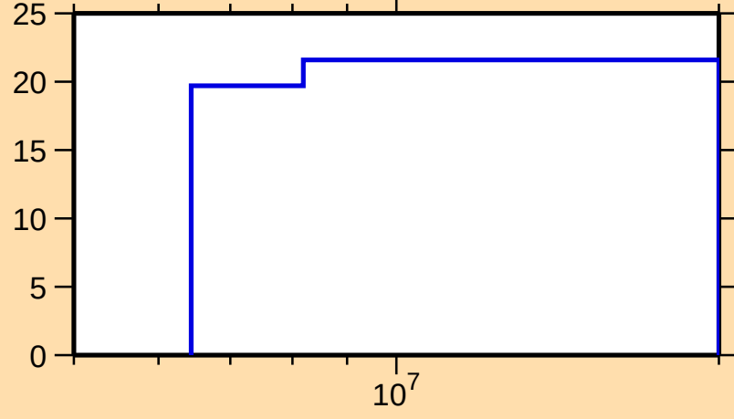
\Delta\sigma/\sigma vs. E for ^{93}\text{Sr}(n,n_1)
