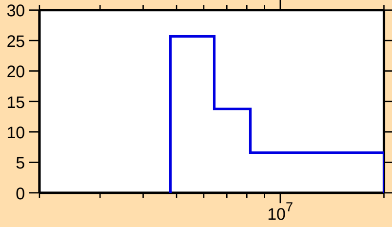
\Delta\sigma/\sigma vs. E for ^{93}\text{Sr}(n,2n)
