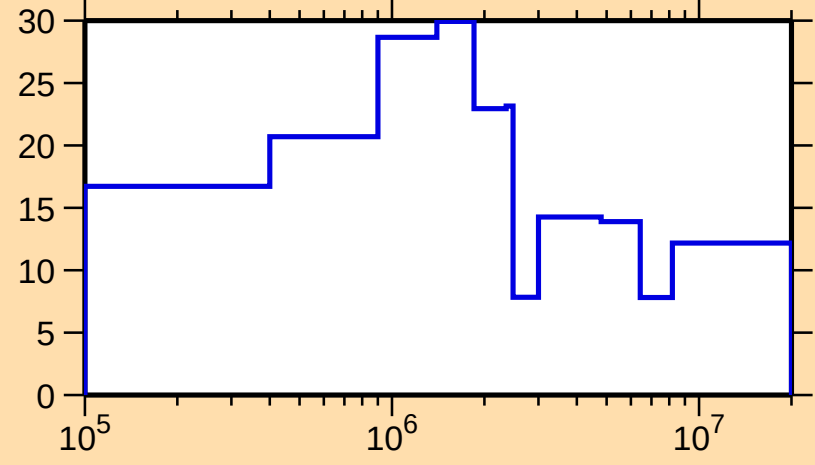
\Delta\sigma/\sigma vs. E for ^{93}\text{Sr}(n,\text{el.})
