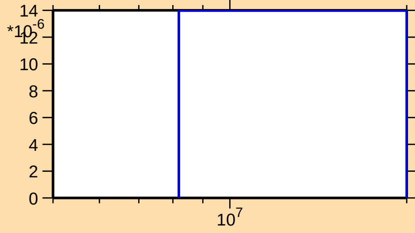
\sigma vs. E for ^{93}\text{Sr}(n,n\alpha)
