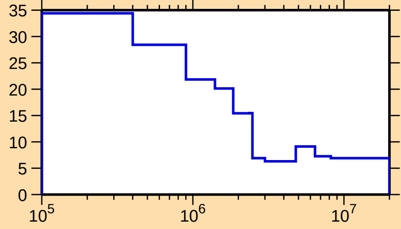
\Delta\sigma/\sigma vs. E for ^{93}\text{Sr}(\text{n,nonel.})
