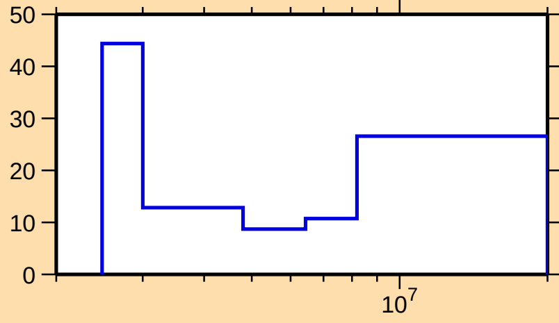
\Delta\sigma/\sigma vs. E for ^{93}\text{Sr}(n,n\text{cont.})
