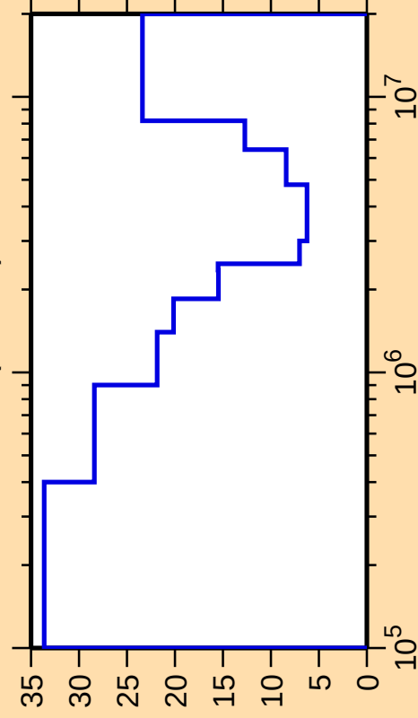
\Delta\sigma/\sigma vs. E for ^{93}\text{Sr}(\text{n,inel.})
