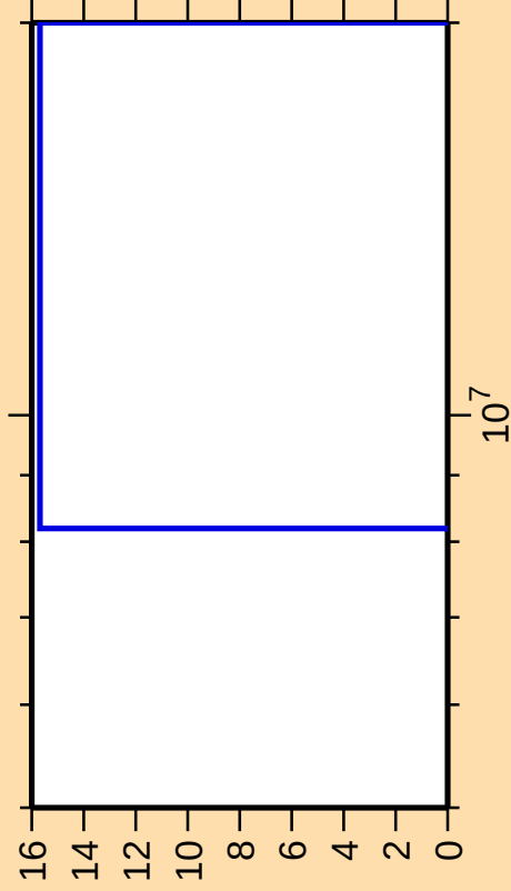
\Delta\sigma/\sigma vs. E for ^{93}\text{Sr}(n,3n)
