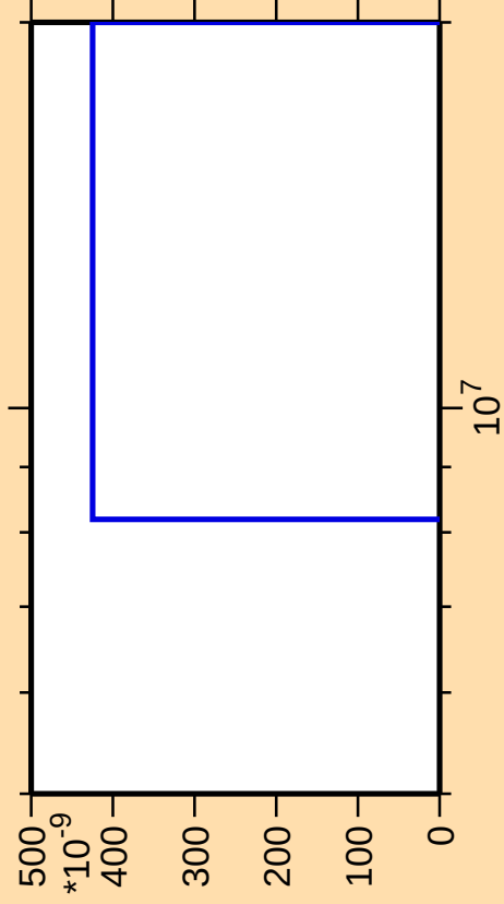
\Delta\sigma/\sigma vs. E for ^{93}\text{Sr}(n,3n\alpha)
