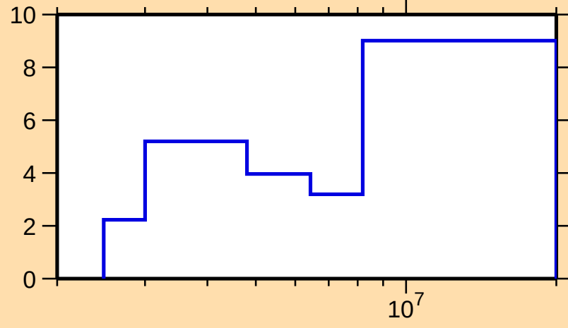
\Delta\sigma/\sigma vs. E for ^{93}\text{Sr}(n,\text{tot.})
