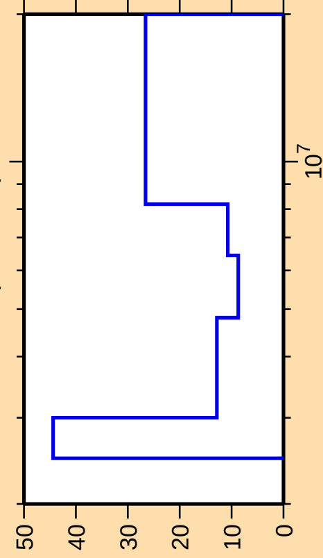
\Delta\sigma/\sigma vs. E for ^{93}\text{Sr}(n,n\text{cont.})
