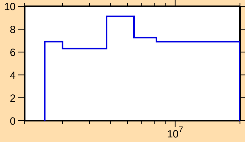
\Delta\sigma/\sigma vs. E for ^{93}\text{Sr}(n,\text{nonel.})
