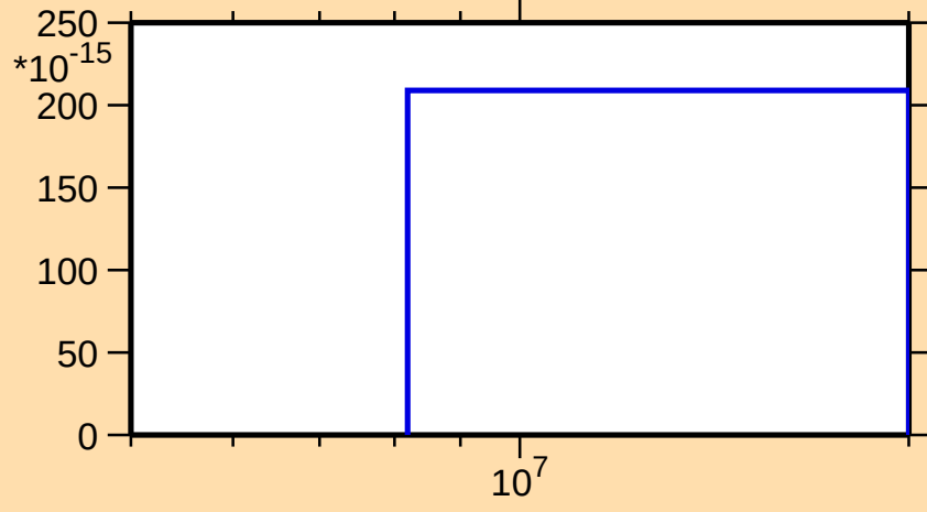
\sigma vs. E for ^{93}\text{Sr}(n,2np)
