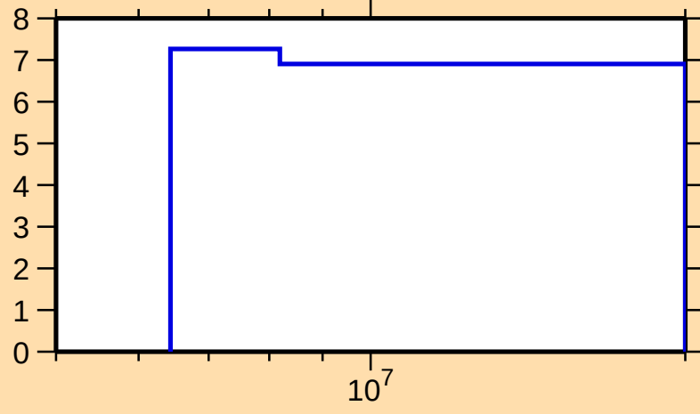
\Delta\sigma/\sigma vs. E for ^{93}\text{Sr}(n,\text{nonel.})
