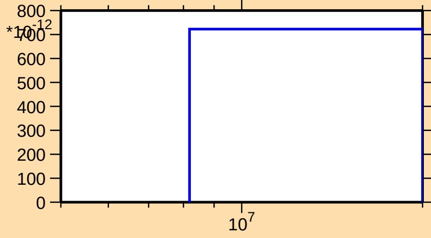
\sigma vs. E for ^{93}\text{Sr}(n,\text{nd})
