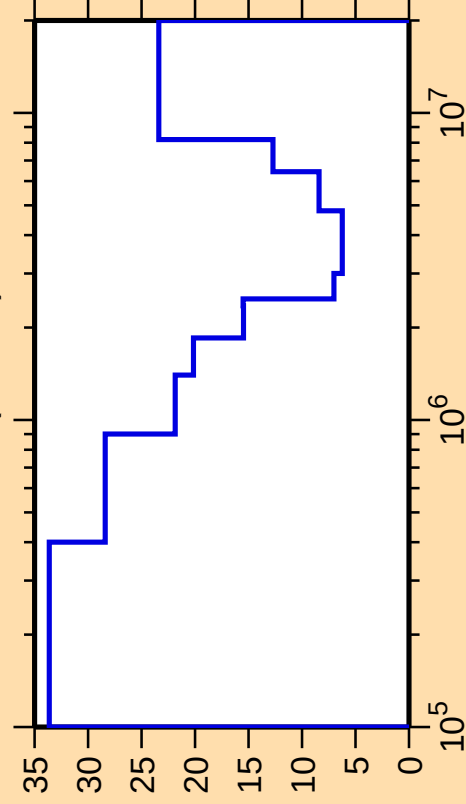
\Delta\sigma/\sigma vs. E for ^{93}\text{Sr}(n,\text{inel.})
