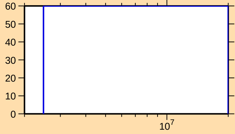
\Delta\sigma/\sigma vs. E for ^{93}\text{Sr}(n,\gamma)
