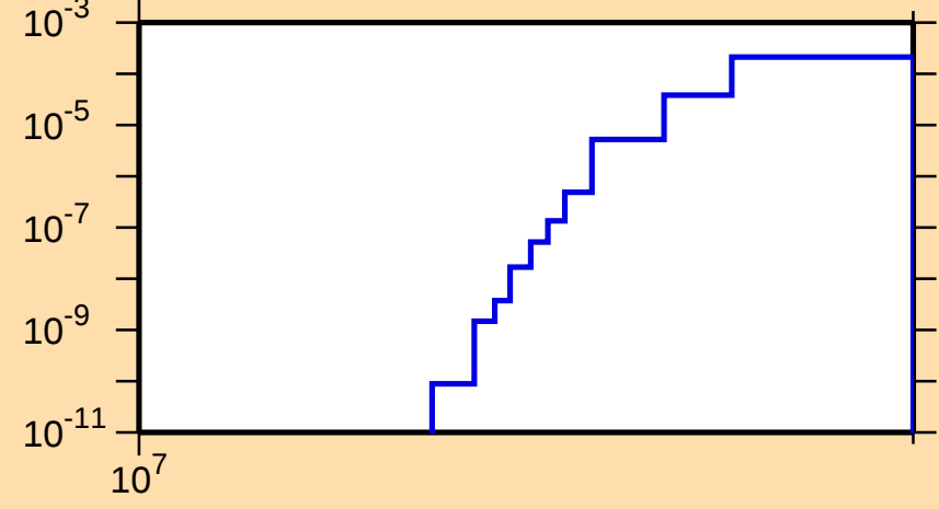
\sigma vs. E for ^{94}\text{Sr}(n,d)
