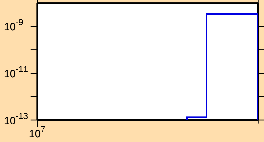
\sigma vs. E for ^{94}\text{Sr}(n,\text{nt})
