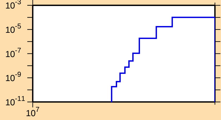
\sigma vs. E for ^{94}\text{Sr}(n,t)
