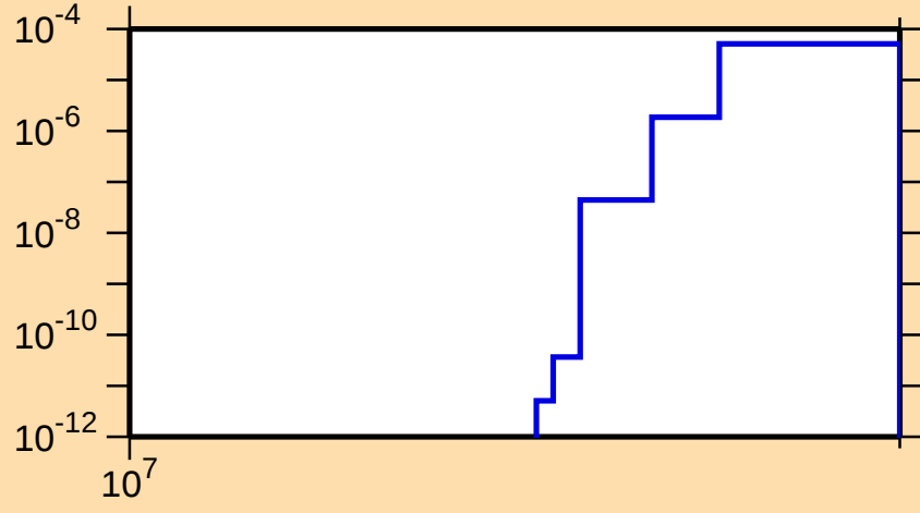
\sigma vs. E for ^{94}\text{Sr}(n,np)
