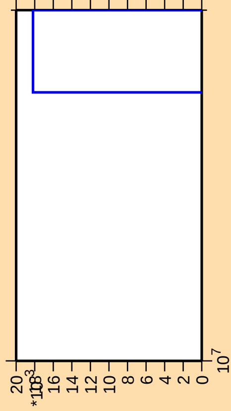
\Delta\sigma/\sigma vs. E for ^{94}\text{Sr}(n,2np)
