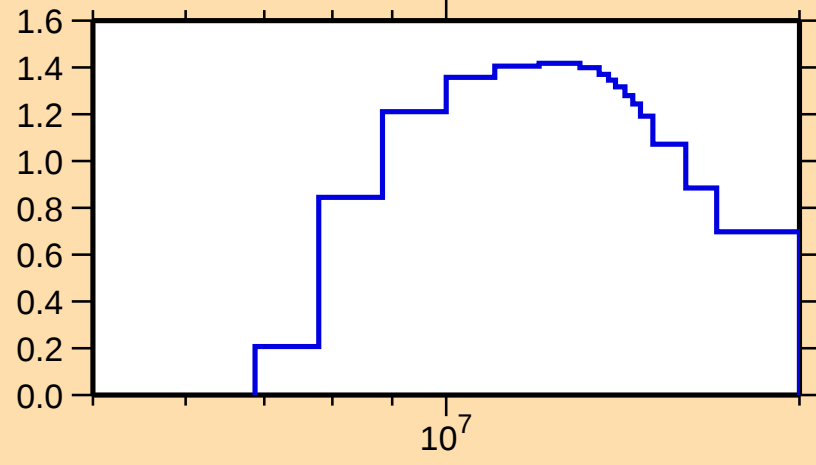
\sigma vs. E for ^{94}\text{Sr}(n,2n)
