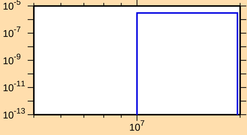
\sigma vs. E for ^{94}\text{Sr}(n,n\alpha)
