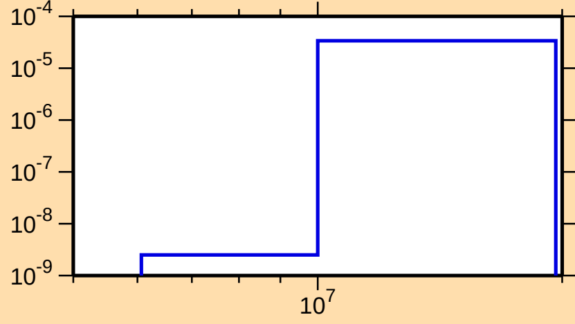
\sigma vs. E for ^{94}\text{Sr}(n,\alpha)
