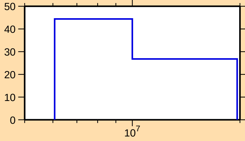
\Delta\sigma/\sigma vs. E for ^{94}\text{Sr}(n,2n)
