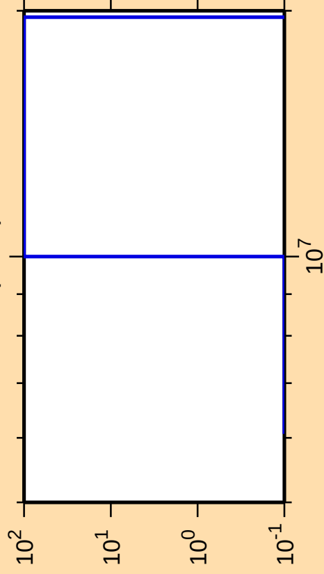
\Delta\sigma/\sigma vs. E for ^{94}\text{Sr}(n,n\alpha)
