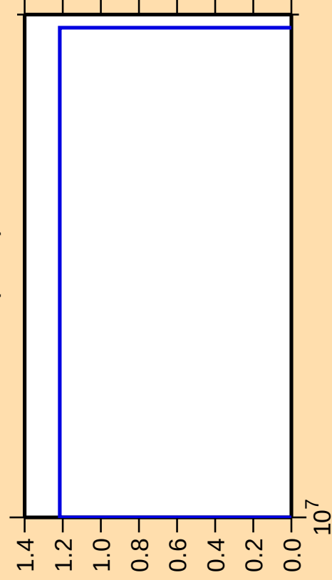
\Delta\sigma/\sigma vs. E for ^{94}\text{Sr}(n,\text{nd})
