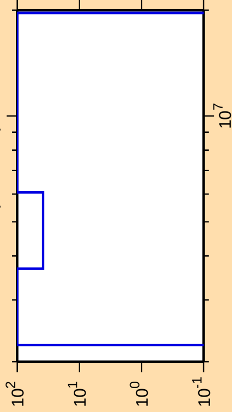
\Delta\sigma/\sigma vs. E for ^{94}\text{Sr}(n,\text{ncont.})
