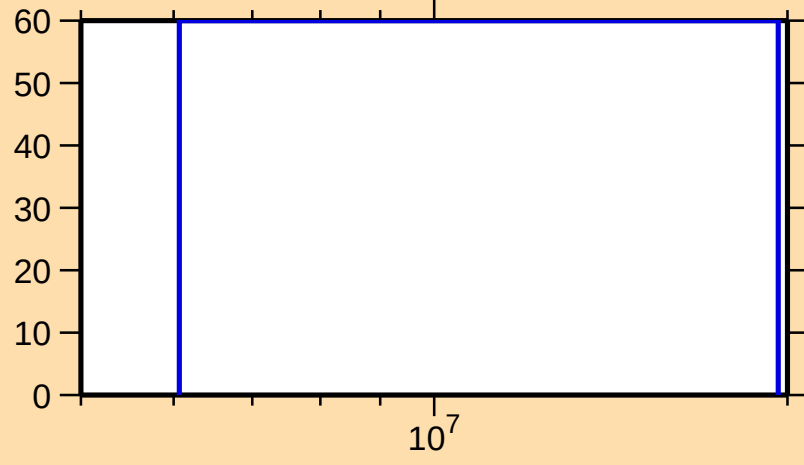
\Delta\sigma/\sigma vs. E for ^{94}\text{Sr}(n,n\text{cont.})
