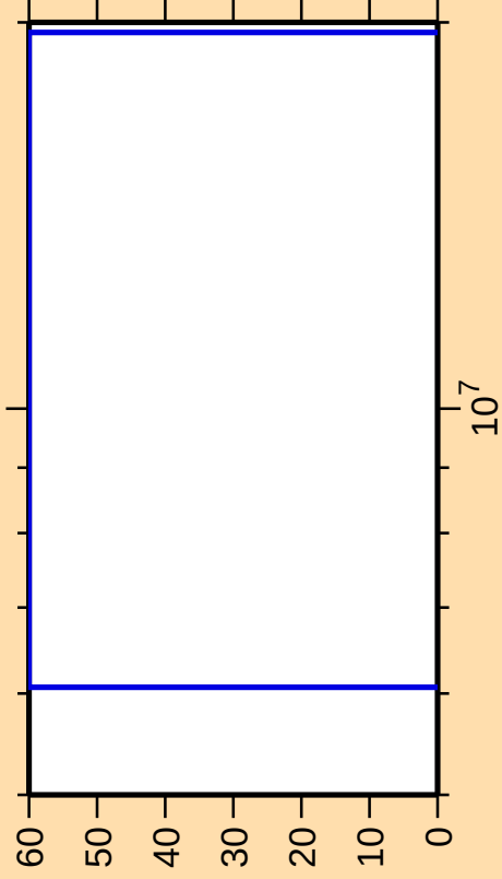
\Delta\sigma/\sigma vs. E for ^{94}\text{Sr}(n,n_1)
