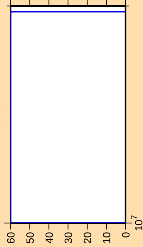
\Delta\sigma/\sigma vs. E for ^{94}\text{Sr}(n,\text{nt})
