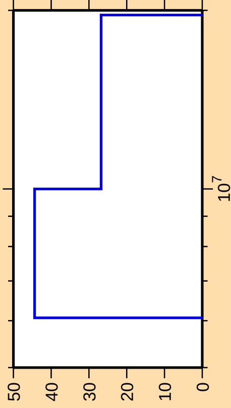
\Delta\sigma/\sigma vs. E for ^{94}\text{Sr}(n,2n)
