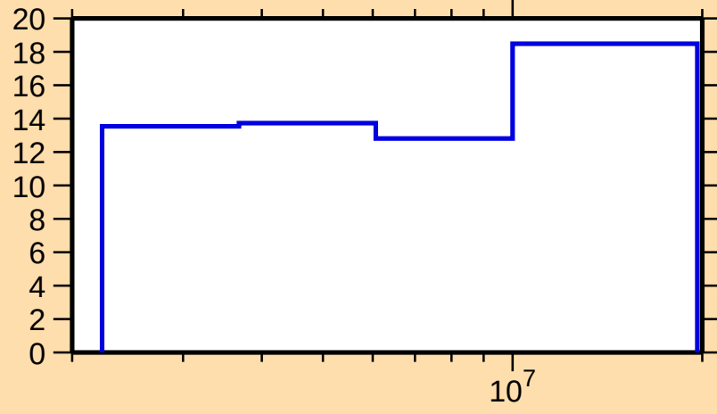
\Delta\sigma/\sigma vs. E for ^{94}\text{Sr}(n,\text{tot.})
