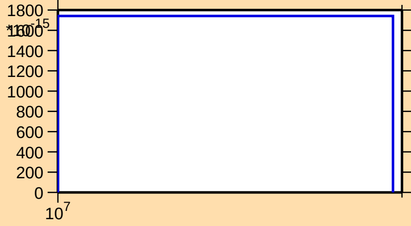
\sigma vs. E for ^{94}\text{Sr}(n,2n\alpha)
