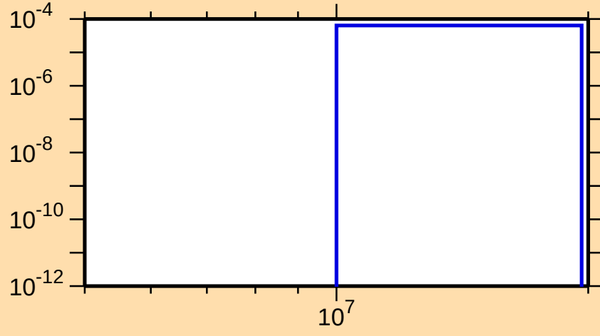
\sigma vs. E for ^{94}\text{Sr}(n,p)
