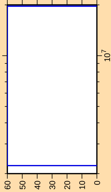
\Delta\sigma/\sigma vs. E for ^{94}\text{Sr}(n,\gamma)
