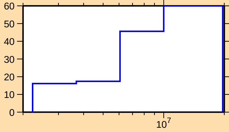
\Delta\sigma/\sigma vs. E for ^{94}\text{Sr}(n,\text{inel.})
