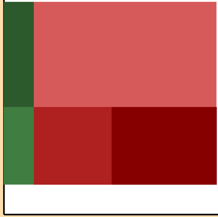
\Delta\sigma/\sigma vs. E for ^{94}\text{Sr}(n,\text{inel.})
