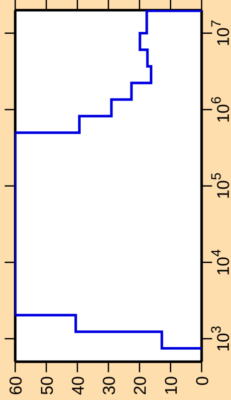
\Delta\sigma/\sigma vs. E for ^{94}\text{Sr}(n,\text{nonel.})
