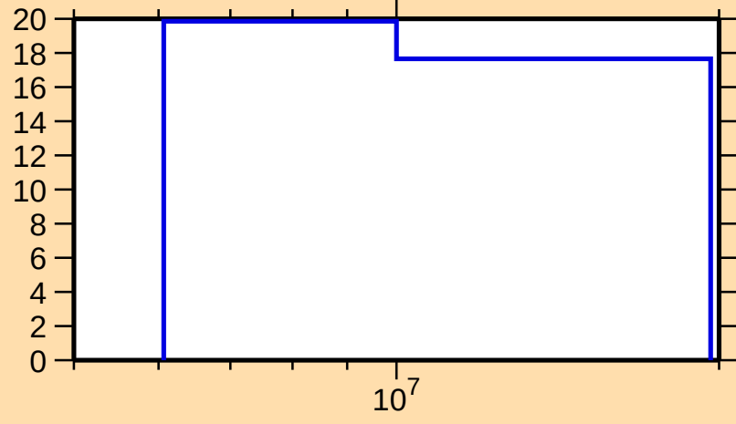
\Delta\sigma/\sigma vs. E for ^{94}\text{Sr}(n,\text{nonel.})
