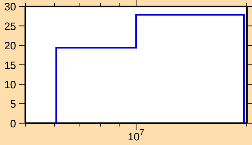
\Delta\sigma/\sigma vs. E for ^{94}\text{Sr}(n,\text{el.})
