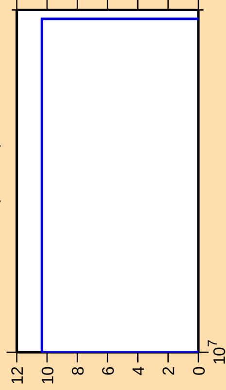
\Delta\sigma/\sigma vs. E for ^{94}\text{Sr}(n,2n\alpha)
