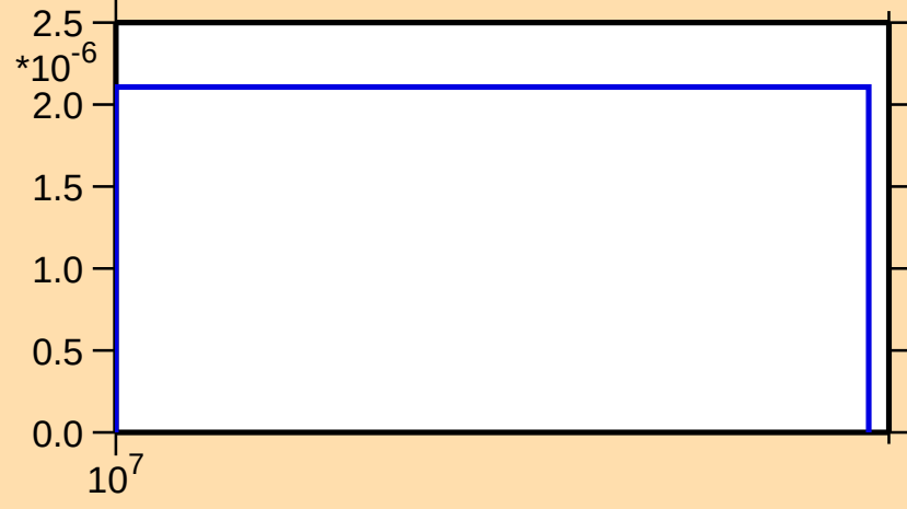
\sigma vs. E for ^{94}\text{Sr}(n,t)
