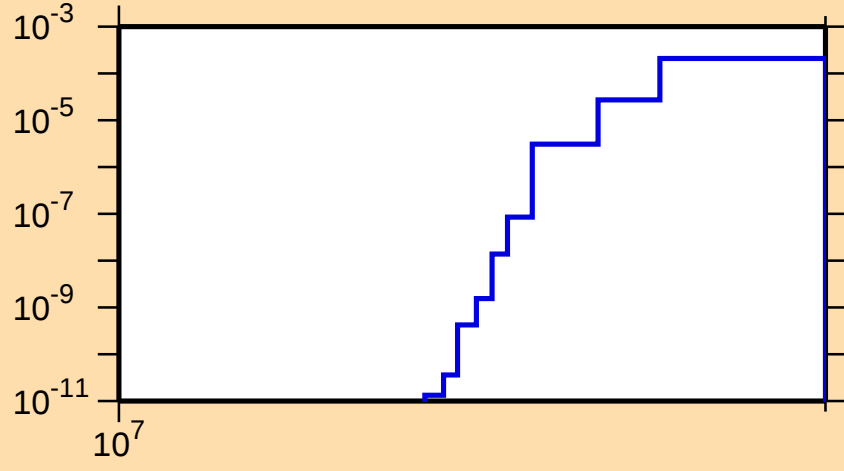
\sigma vs. E for ^{95}\text{Sr}(n,d)
