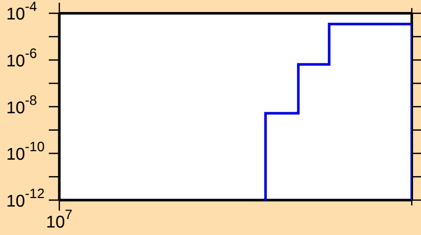
\sigma vs. E for ^{95}\text{Sr}(n,np)
