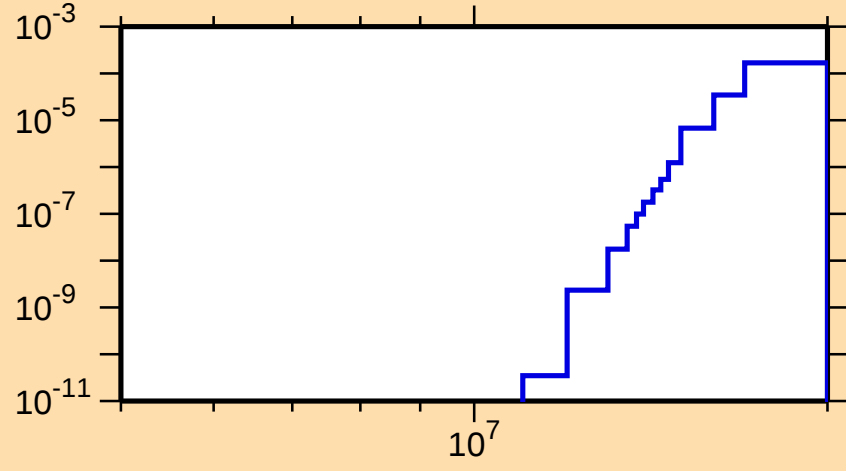
\sigma vs. E for ^{95}\text{Sr}(n,\alpha)
