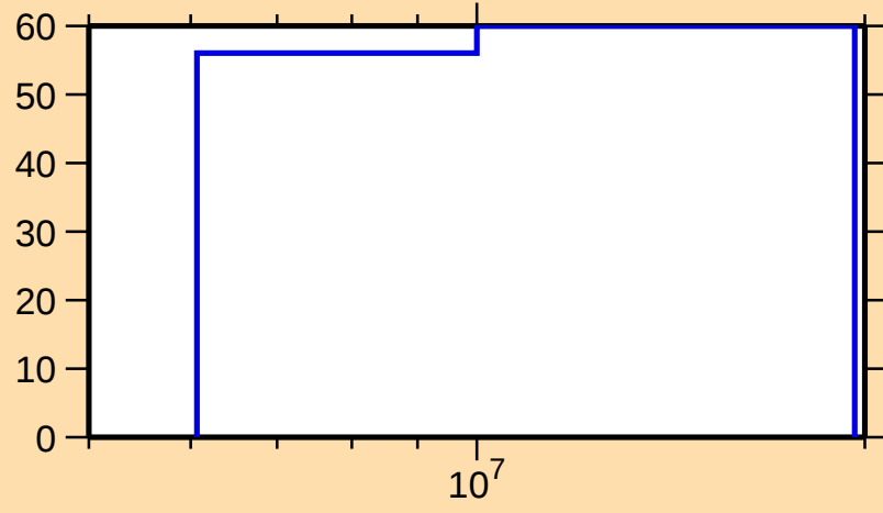
\Delta\sigma/\sigma vs. E for ^{95}\text{Sr}(n,\text{inel.})
