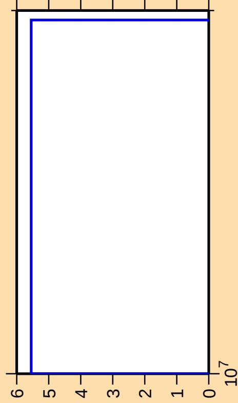
\Delta\sigma/\sigma vs. E for ^{95}\text{Sr}(n,2np)
