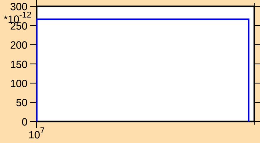
\sigma vs. E for ^{95}\text{Sr}(n,2n\alpha)
