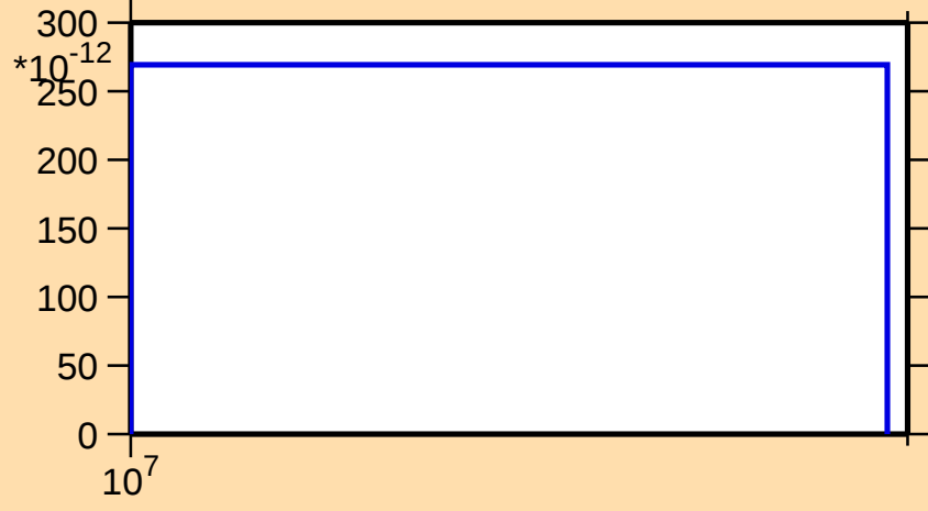
\sigma vs. E for ^{95}\text{Sr}(n,\text{nt})
