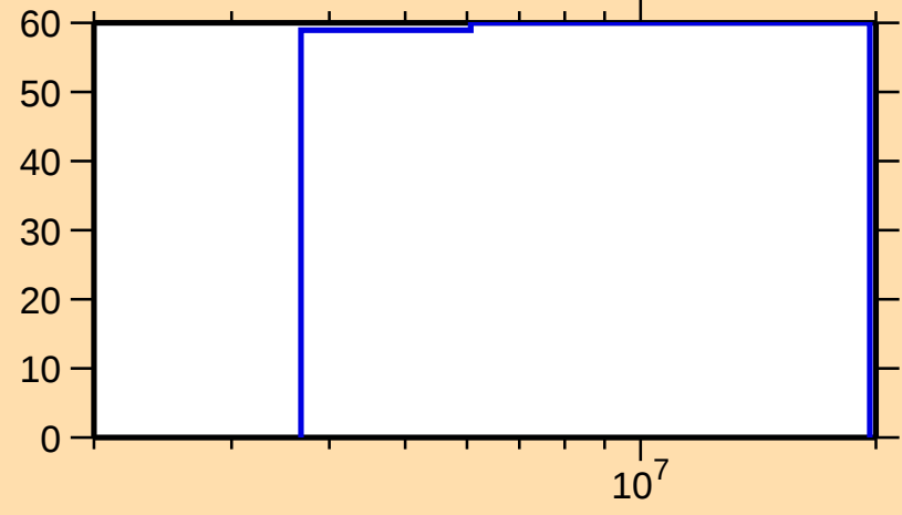
\Delta\sigma/\sigma vs. E for ^{95}\text{Sr}(n,n\text{cont.})
