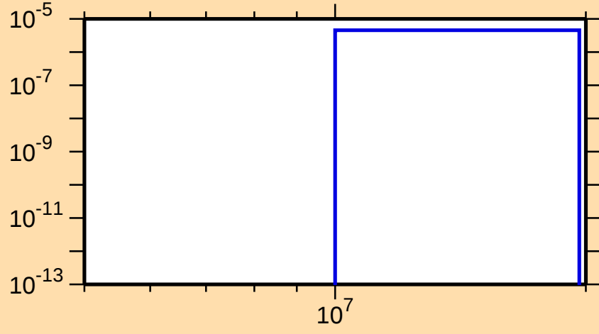
\sigma vs. E for ^{95}\text{Sr}(n,n\alpha)
