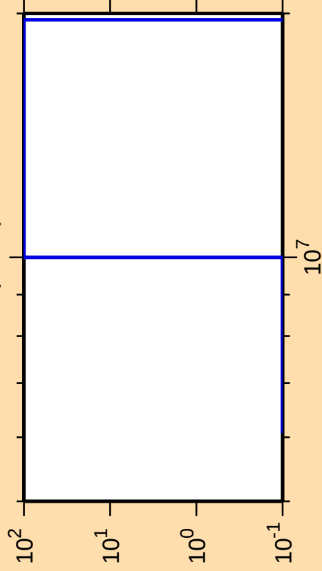
\Delta\sigma/\sigma vs. E for ^{95}\text{Sr}(n,n\alpha)
