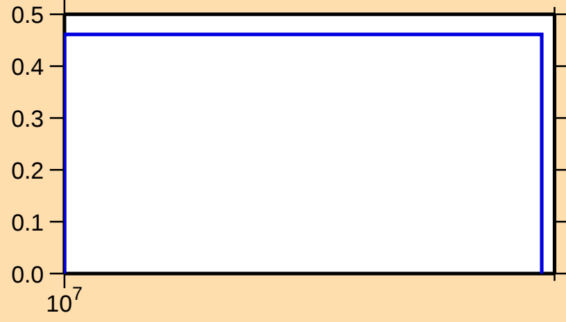
\sigma vs. E for ^{95}\text{Sr}(n,3n)
