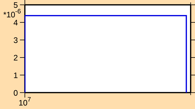
\sigma vs. E for ^{95}\text{Sr}(n,t)
