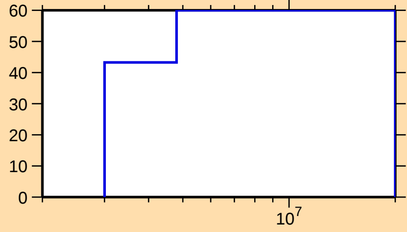
\Delta\sigma/\sigma vs. E for ^{95}\text{Sr}(n,\text{ncont.})
