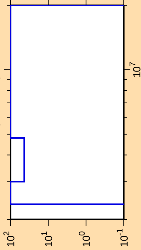
\Delta\sigma/\sigma vs. E for ^{95}\text{Sr}(n,n\text{cont.})
