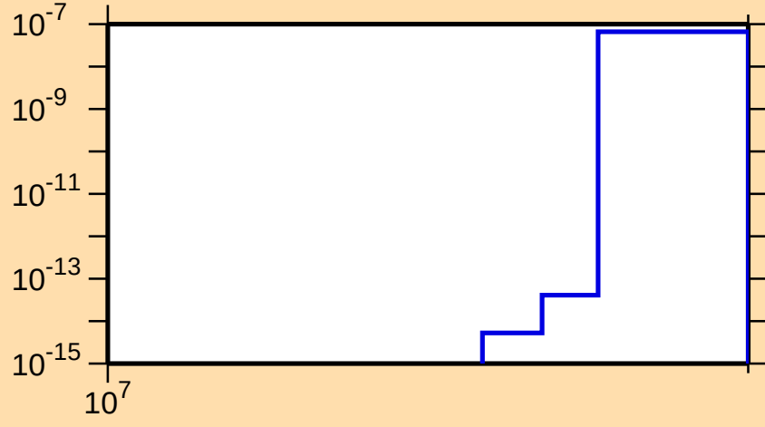
\sigma vs. E for ^{96}\text{Sr}(n,\text{nt})
