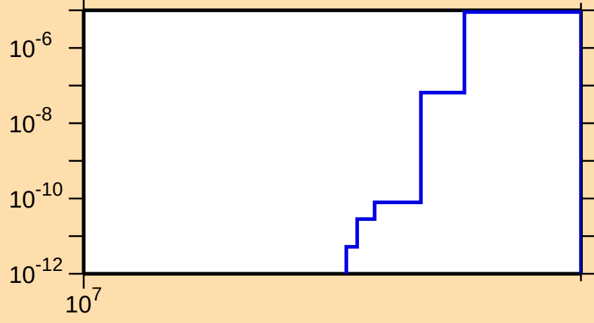
\sigma vs. E for ^{96}\text{Sr}(n,np)
