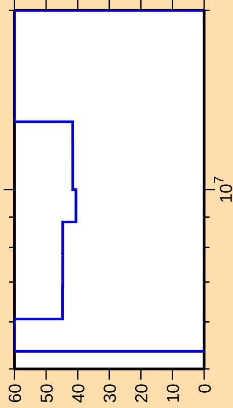
\Delta\sigma/\sigma vs. E for ^{96}\text{Sr}(n,2n)
