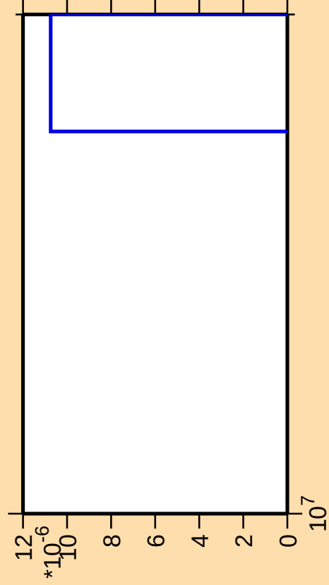
\Delta\sigma/\sigma vs. E for ^{96}\text{Sr}(n,2np)
