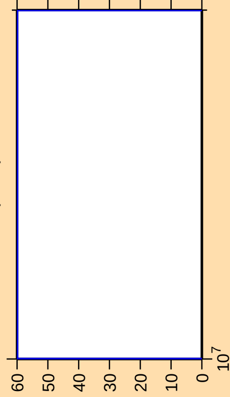
\Delta\sigma/\sigma vs. E for ^{96}\text{Sr}(n,3n)
