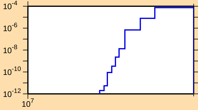
\sigma vs. E for ^{96}\text{Sr}(n,d)
