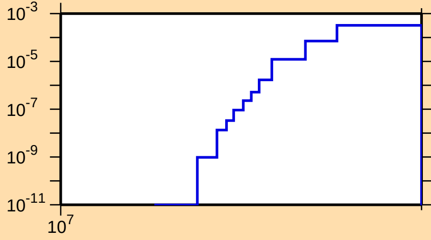
\sigma vs. E for ^{96}\text{Sr}(n,p)
