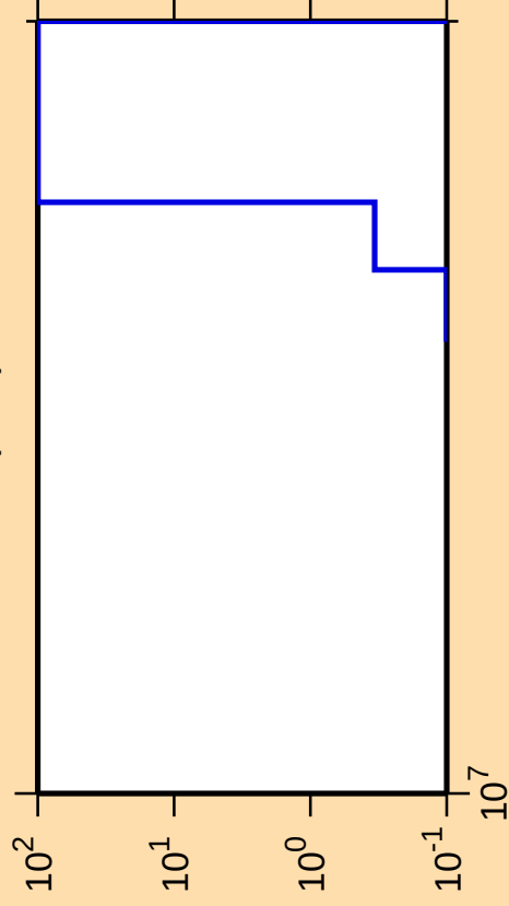
\Delta\sigma/\sigma vs. E for ^{96}\text{Sr}(n,\text{nt})
