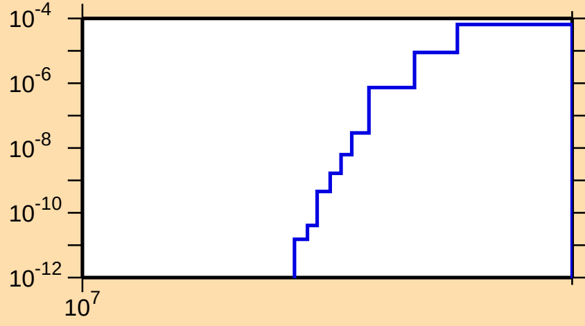
\sigma vs. E for ^{96}\text{Sr}(n,t)
