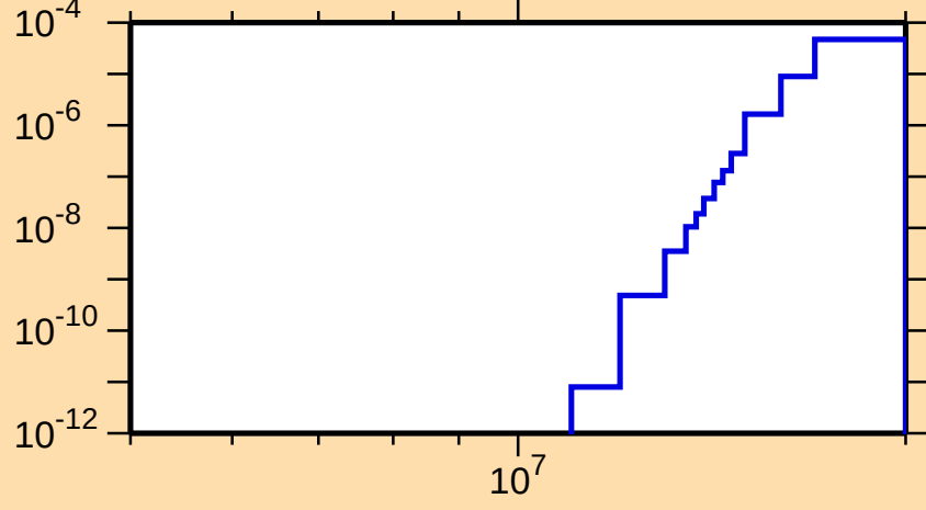
\sigma vs. E for ^{96}\text{Sr}(n,\alpha)
