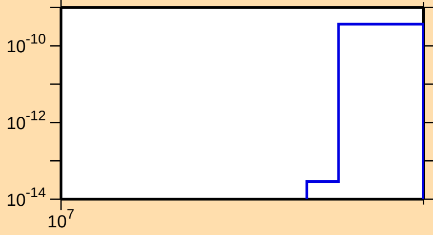
\sigma vs. E for ^{96}\text{Sr}(n,2n\alpha)
