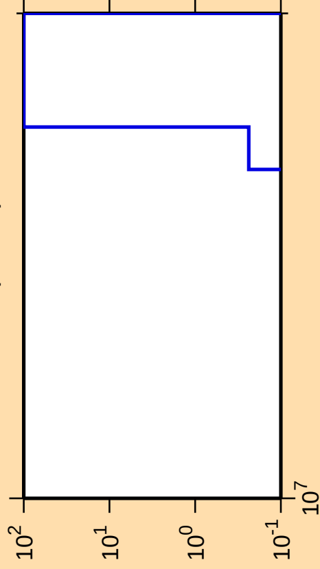
\Delta\sigma/\sigma vs. E for ^{96}\text{Sr}(n,2n\alpha)
