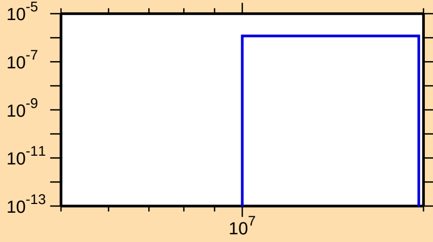
\sigma vs. E for ^{96}\text{Sr}(n,n\alpha)
