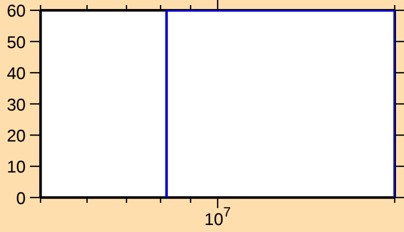
\Delta\sigma/\sigma vs. E for ^{96}\text{Sr}(n,ncont.)
