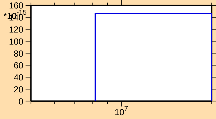
\sigma vs. E for ^{96}\text{Sr}(n,\text{nd})
