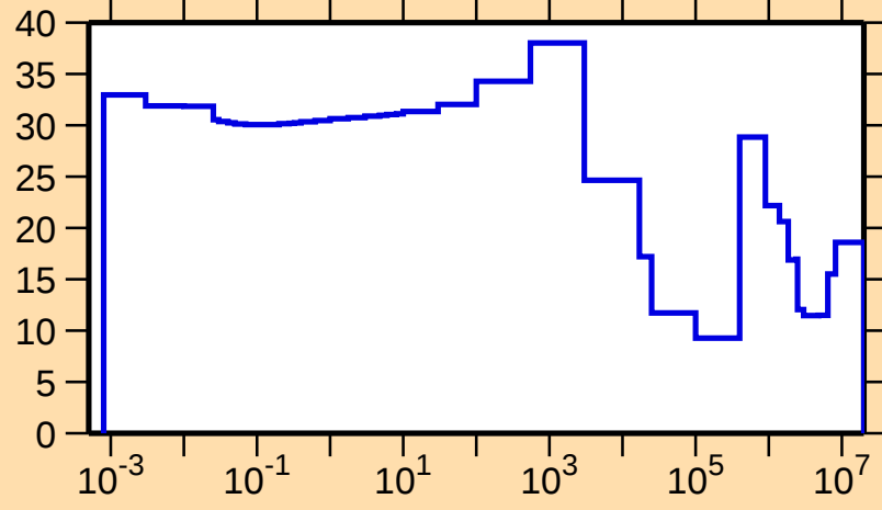
\Delta\sigma/\sigma vs. E for ^{96}\text{Sr}(n,\text{tot.})
