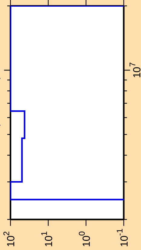
\Delta\sigma/\sigma vs. E for ^{96}\text{Sr}(n,n\text{cont.})
