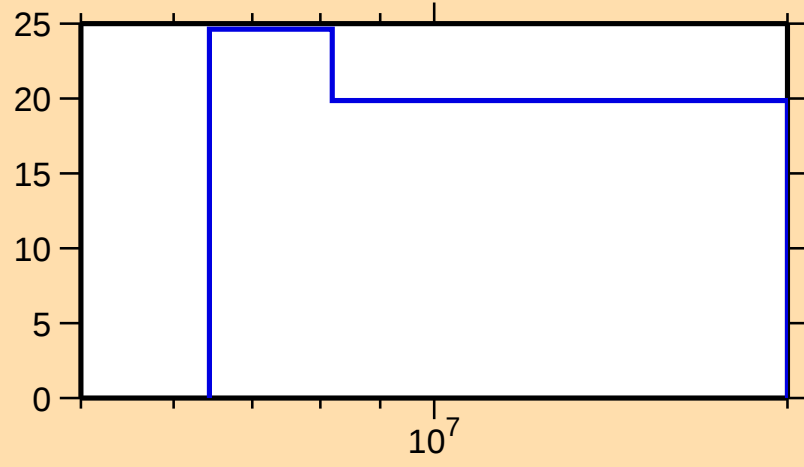
\Delta\sigma/\sigma vs. E for ^{96}\text{Sr}(n,\text{nonel.})
