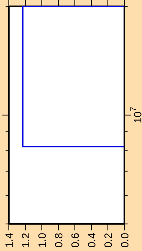
\Delta\sigma/\sigma vs. E for ^{96}\text{Sr}(n,\text{nd})
