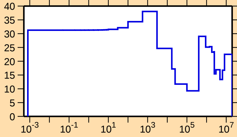
\Delta\sigma/\sigma vs. E for ^{96}\text{Sr}(n,\text{el.})
