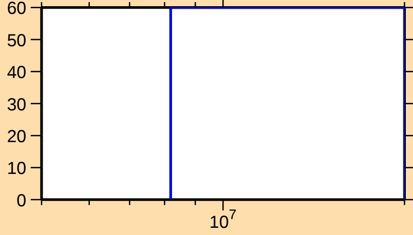
\Delta\sigma/\sigma vs. E for ^{96}\text{Sr}(n,p)
