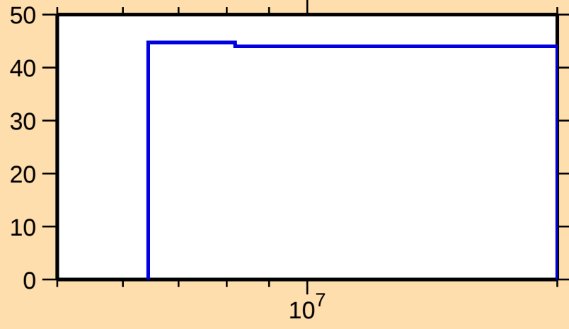
\Delta\sigma/\sigma vs. E for ^{96}\text{Sr}(n,2n)
