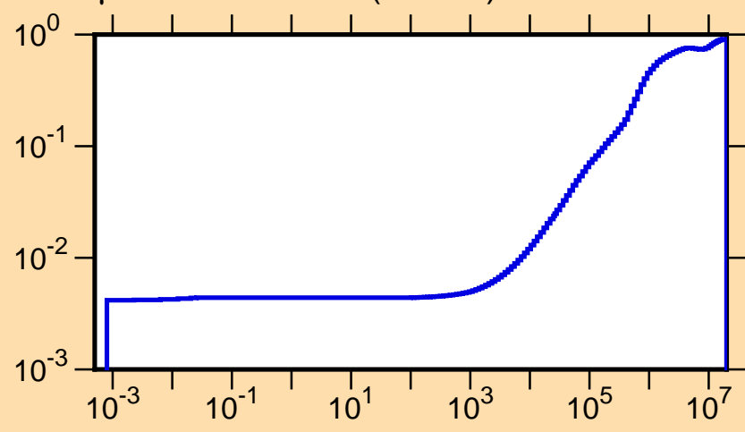
\mu vs. E for ^{162}\text{Ta}(\text{mt251})
