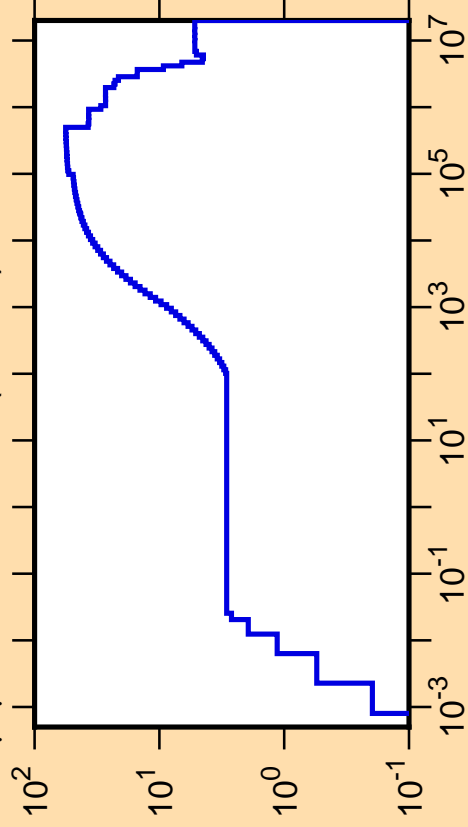
\Delta\mu/\mu vs. E for ^{162}\text{Ta}(\text{mt251})
