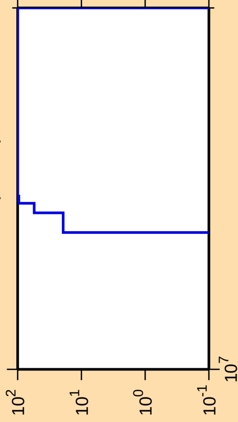
\Delta\sigma/\sigma vs. E for ^{162}\text{Ta}(\text{mt } 34)
