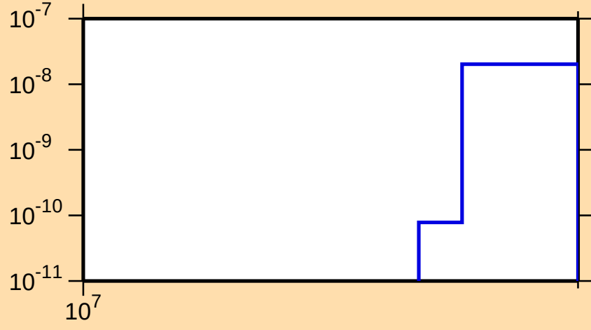
\sigma vs. E for ^{162}\text{Ta}(n,\text{nt})
