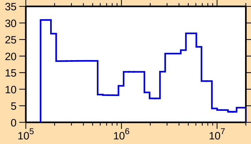
\Delta\sigma/\sigma vs. E for ^{162}\text{Ta}(n,\text{el.})
