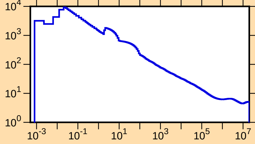
\sigma vs. E for ^{162}\text{Ta}(n,\text{tot.})
