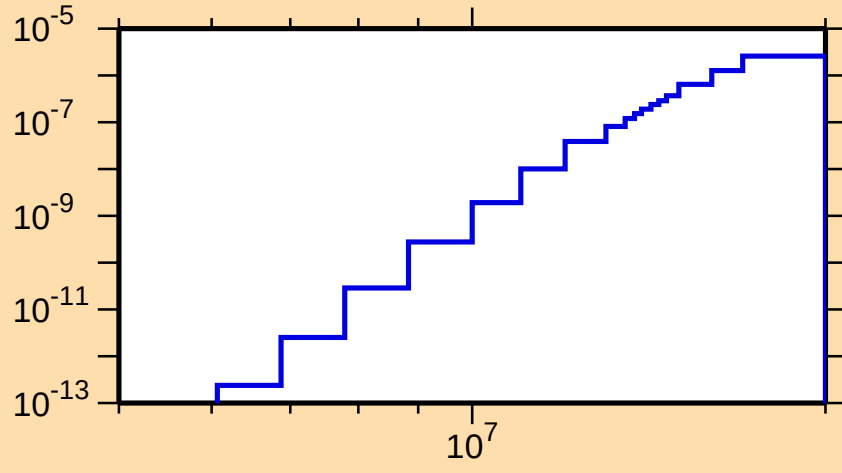
\sigma vs. E for ^{162}\text{Ta}(\text{mt117})
