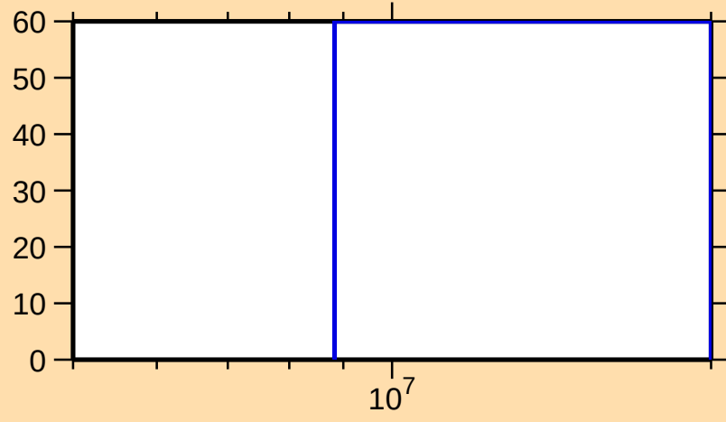
\Delta\sigma/\sigma vs. E for ^{162}\text{Ta}(n,\text{inel.})
