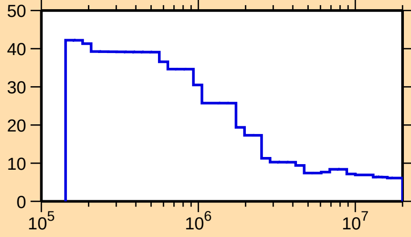
\Delta\sigma/\sigma vs. E for ^{162}\text{Ta}(n,\text{nonel.})
