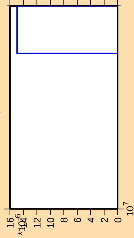
\Delta\sigma/\sigma vs. E for ^{162}\text{Ta}(\text{mt } 11)
