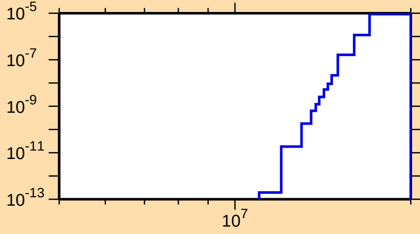
\sigma vs. E for ^{162}\text{Ta}(n,\text{pt})
