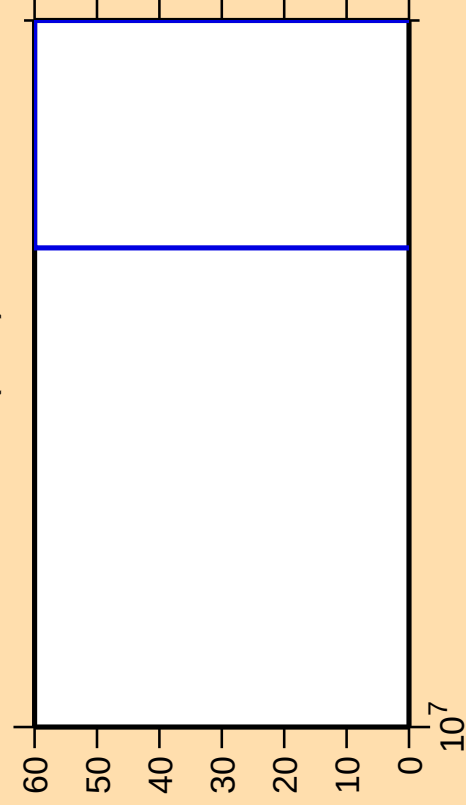
\Delta\sigma/\sigma vs. E for ^{162}\text{Ta}(n,\text{nt})
