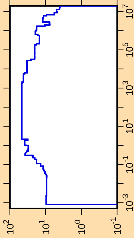
\Delta\sigma/\sigma vs. E for ^{162}\text{Ta}(n,\text{tot.})
