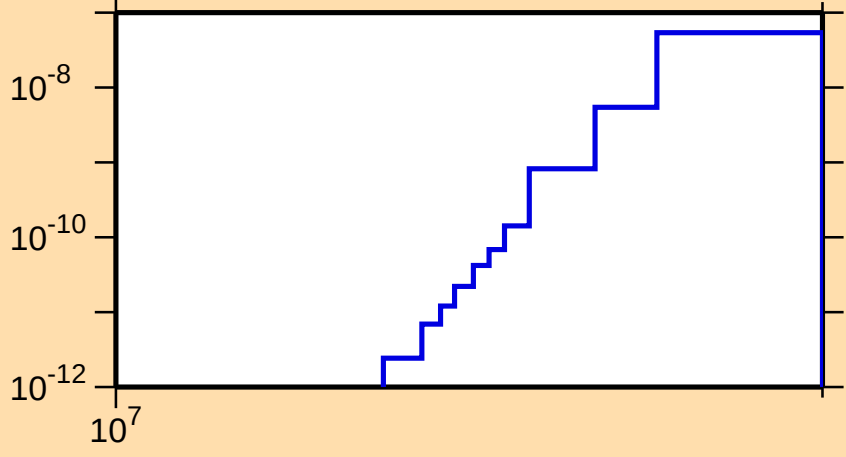
\sigma vs. E for ^{162}\text{Ta}(\text{mt } 34)
