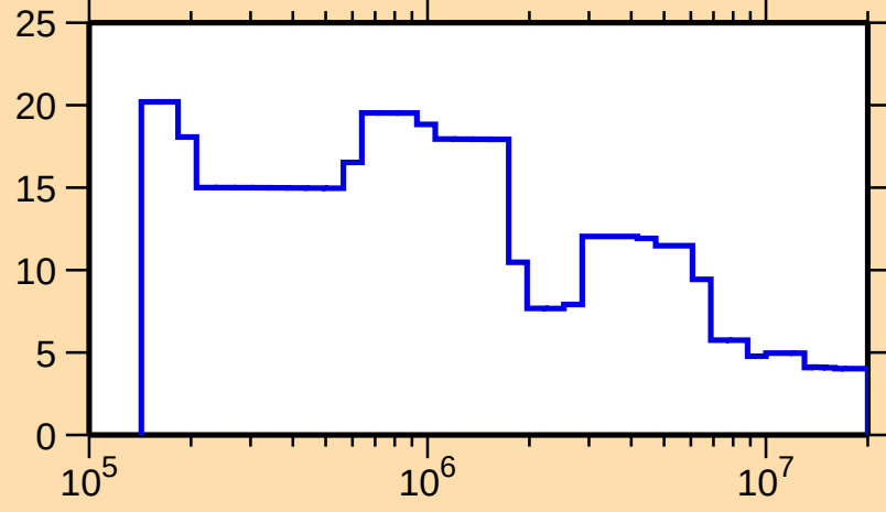
\Delta\sigma/\sigma vs. E for ^{162}\text{Ta}(n,\text{tot.})
