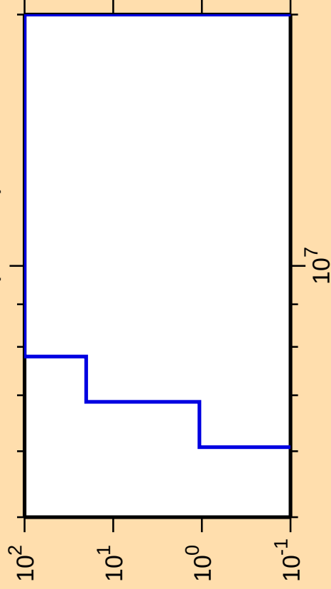
\Delta\sigma/\sigma vs. E for ^{162}\text{Ta}(\text{mt117})
