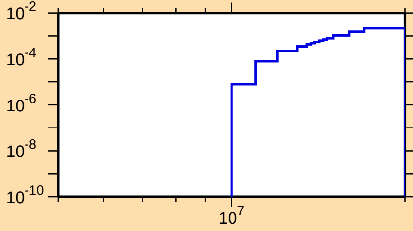
\sigma vs. E for ^{162}\text{Ta}(n,2n\alpha)
