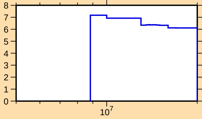
\Delta\sigma/\sigma vs. E for ^{162}\text{Ta}(n,\text{nonel.})
