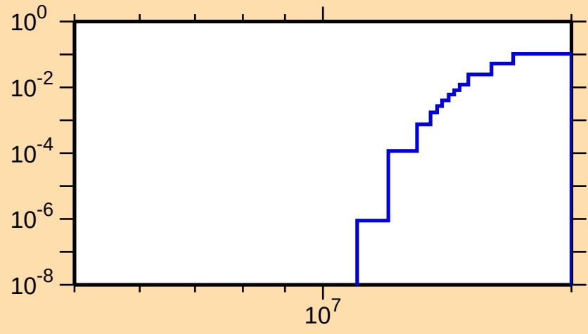
\sigma vs. E for ^{162}\text{Ta}(n,2np)
