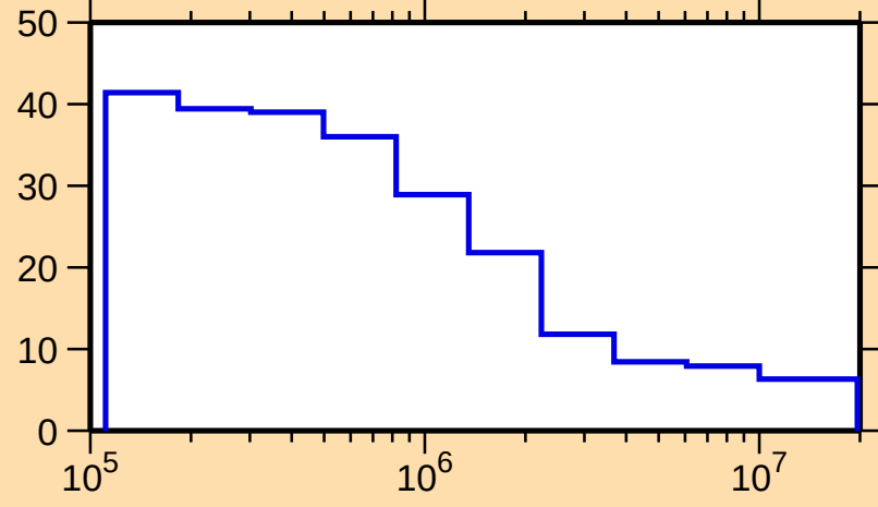
\Delta\sigma/\sigma vs. E for ^{162}\text{Ta}(n,n\text{onel.})
