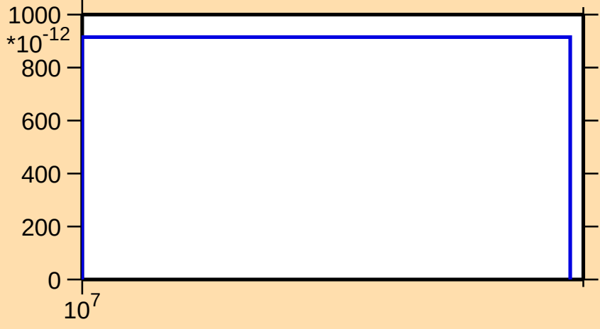
\sigma vs. E for ^{162}\text{Ta} (mt 34)
