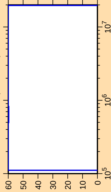
\Delta\sigma/\sigma vs. E for ^{162}\text{Ta}(n,n\text{cont.})
