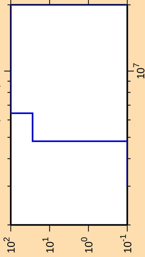
\Delta\sigma/\sigma vs. E for ^{162}\text{Ta}(\text{mt } 45)
