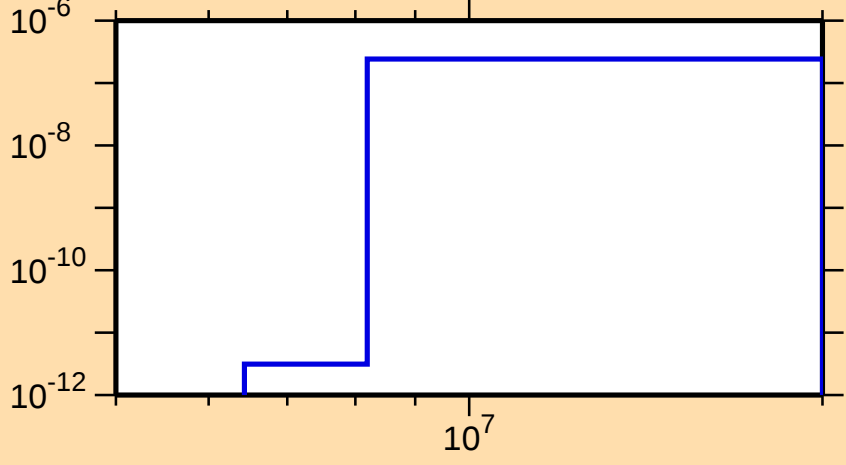
\sigma vs. E for ^{162}\text{Ta}(\text{mt117})
