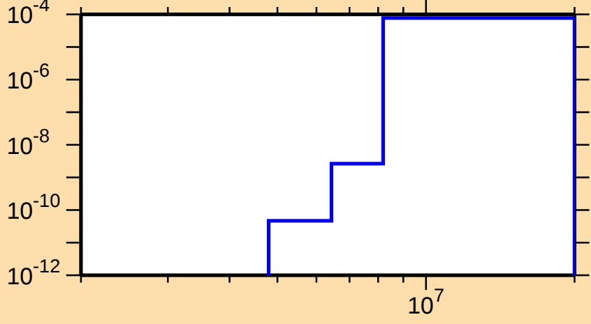
\sigma vs. E for ^{162}\text{Ta}(n,\text{He3})
