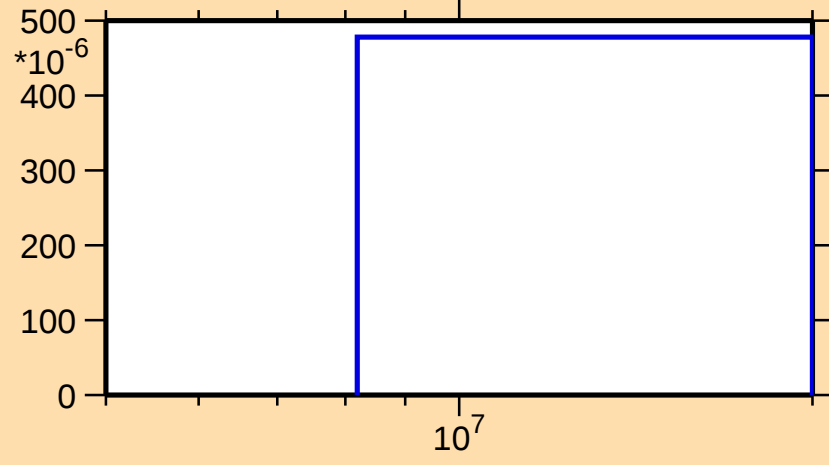
\sigma vs. E for ^{162}\text{Ta}(n,2n\alpha)
