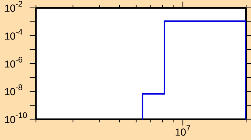
\sigma vs. E for ^{162}\text{Ta}(n,t)
