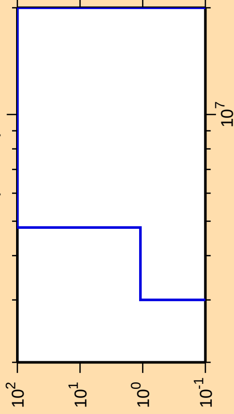
\Delta\sigma/\sigma vs. E for ^{162}\text{Ta}(n,\text{He3})
