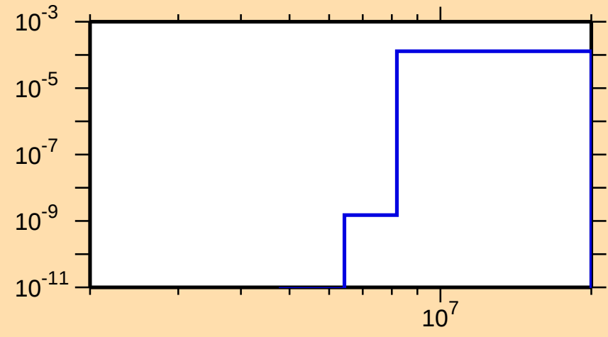
\sigma vs. E for ^{162}\text{Ta}(\text{mt } 45)
