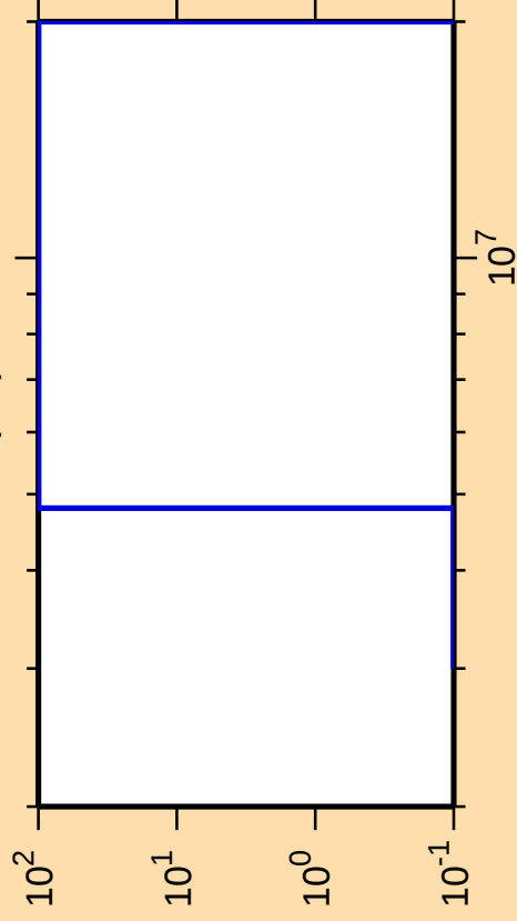
\Delta\sigma/\sigma vs. E for ^{162}\text{Ta}(n,t)
