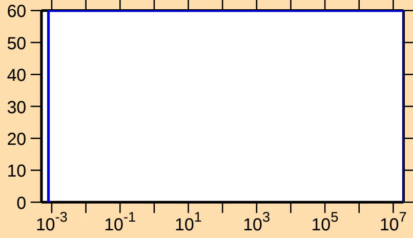
\Delta\sigma/\sigma vs. E for ^{166}\text{Ta}(n,p)
