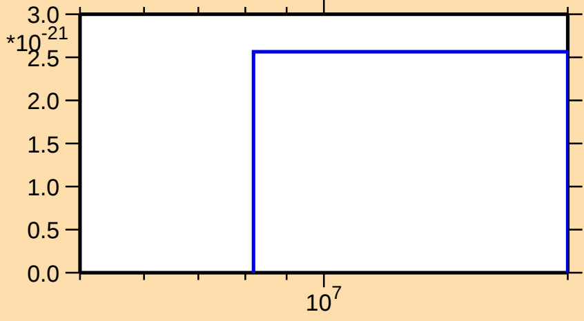
\sigma vs. E for ^{166}\text{Ta}(\text{mt } 11)
