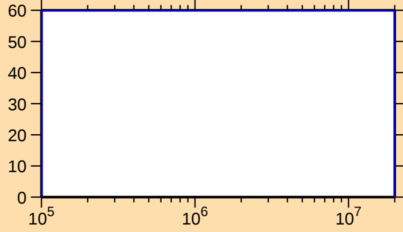
\Delta\sigma/\sigma vs. E for ^{166}\text{Ta}(n,n_1)
