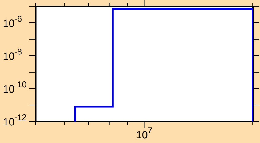
\sigma vs. E for ^{166}\text{Ta}(n,\text{He3})
