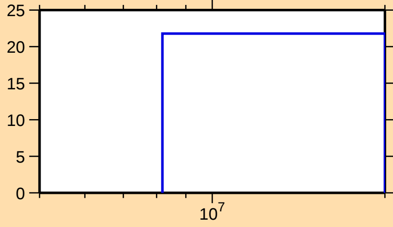
\Delta\sigma/\sigma vs. E for ^{166}\text{Ta}(n,\text{nonel.})
