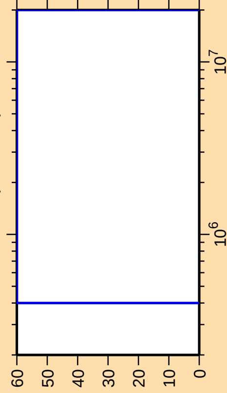
\Delta\sigma/\sigma vs. E for ^{166}\text{Ta}(n,\text{ncont.})
