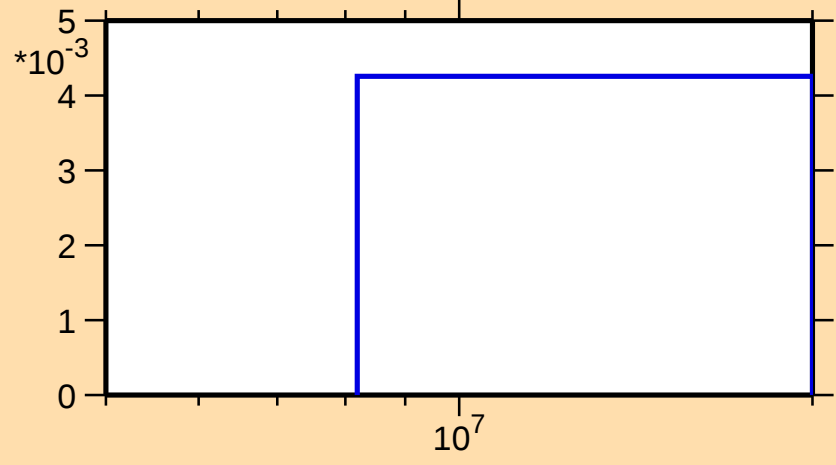
\sigma vs. E for ^{166}\text{Ta}(n,2np)
