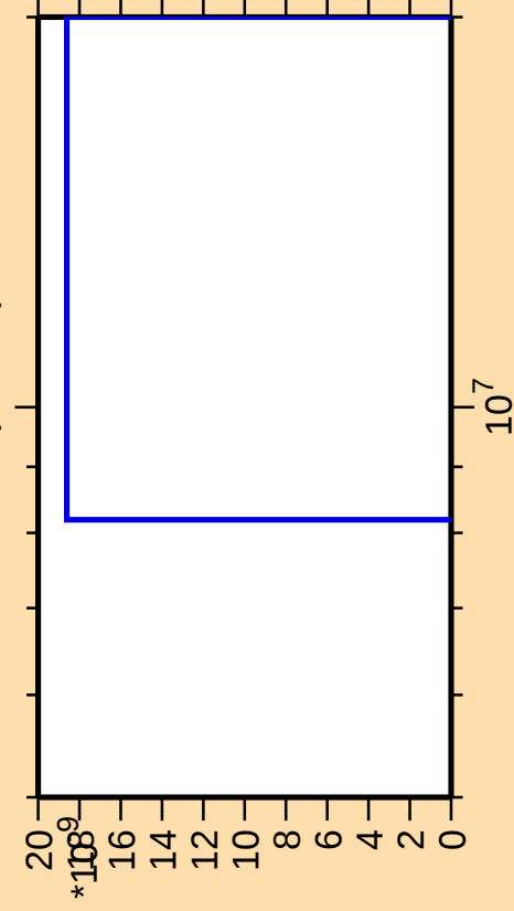
\Delta\sigma/\sigma vs. E for ^{166}\text{Ta}(\text{mt } 11)
