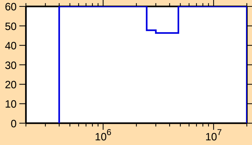
\Delta\sigma/\sigma vs. E for ^{166}\text{Ta}(n,\text{inel.})
