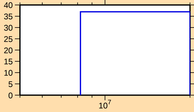
\Delta\sigma/\sigma vs. E for ^{166}\text{Ta}(n,\text{el.})
