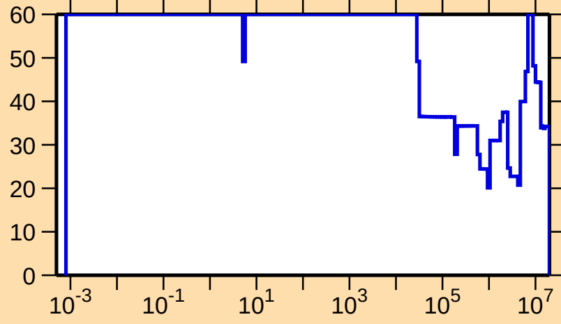
\Delta\sigma/\sigma vs. E for ^{167}\text{Ta}(n,\text{el.})
