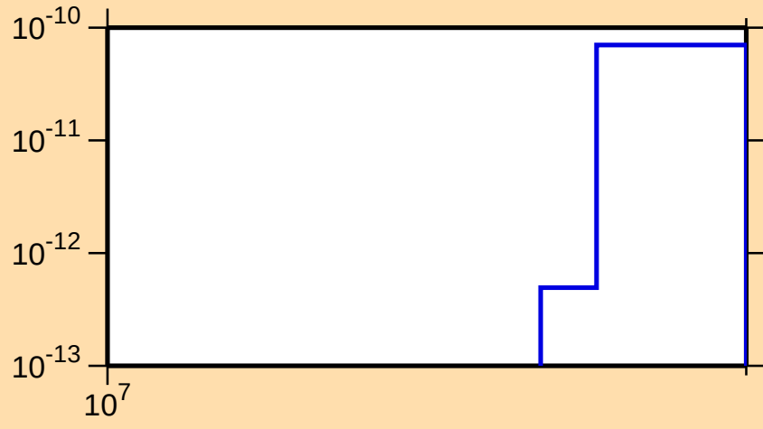
\sigma vs. E for ^{167}\text{Ta}(n,\text{pt})
