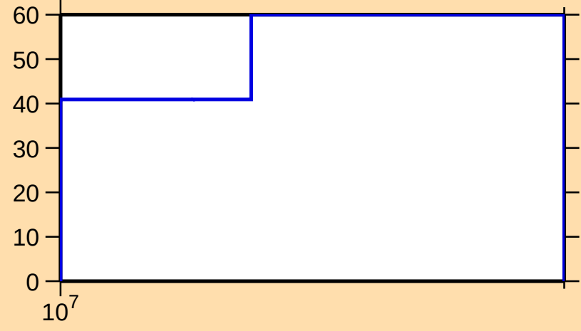
\Delta\sigma/\sigma vs. E for ^{167}\text{Ta}(n,\text{inel.})
