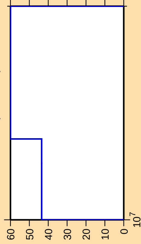
\Delta\sigma/\sigma vs. E for ^{167}\text{Ta}(n,n\text{cont.})
