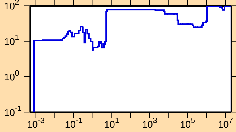
\Delta\sigma/\sigma vs. E for ^{167}\text{Ta}(n,\gamma)
