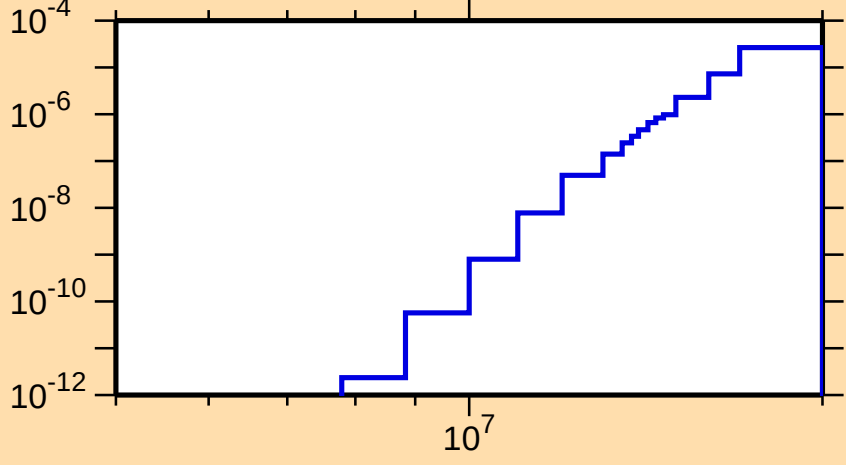
\sigma vs. E for ^{167}\text{Ta}(n,\text{He3})
