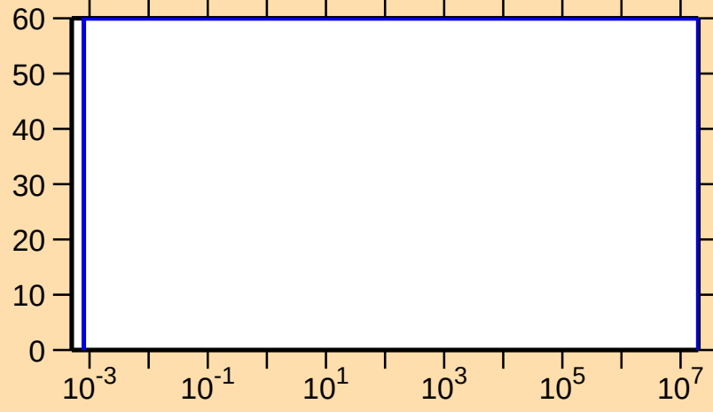
\Delta\sigma/\sigma vs. E for ^{167}\text{Ta}(n,p)
