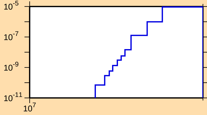
\sigma vs. E for ^{167}\text{Ta}(n,2n\alpha)
