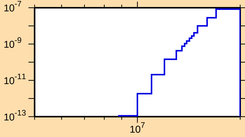
\sigma vs. E for ^{167}\text{Ta}(\text{mt117})
