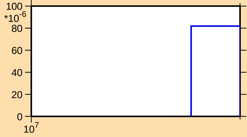
\sigma vs. E for ^{167}\text{Ta}(n,3n)
