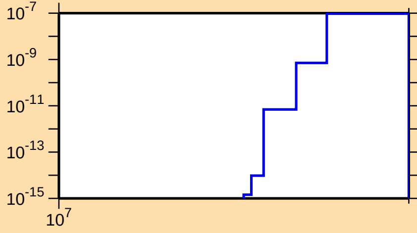
\sigma vs. E for ^{167}\text{Ta}(n,nt)
