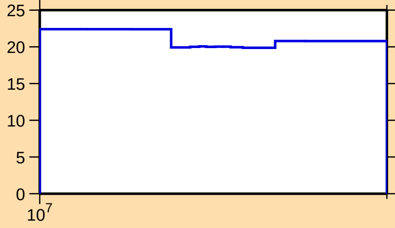
\Delta\sigma/\sigma vs. E for ^{167}\text{Ta}(n,\text{tot.})
