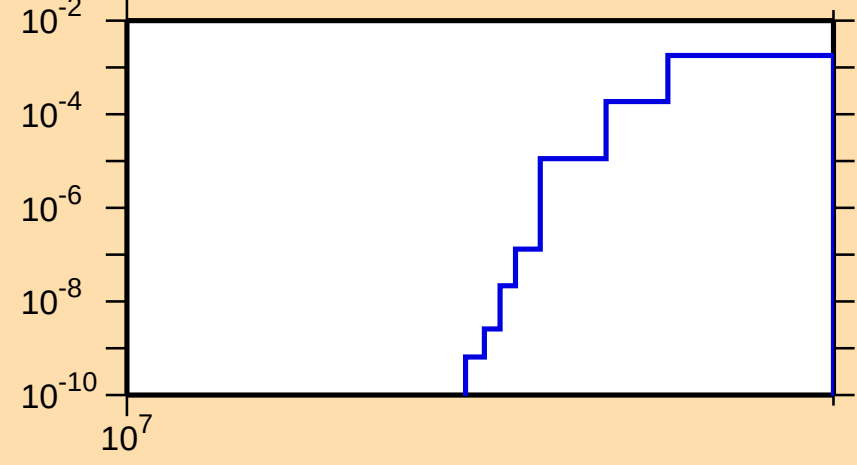
\sigma vs. E for ^{167}\text{Ta}(n,2np)
