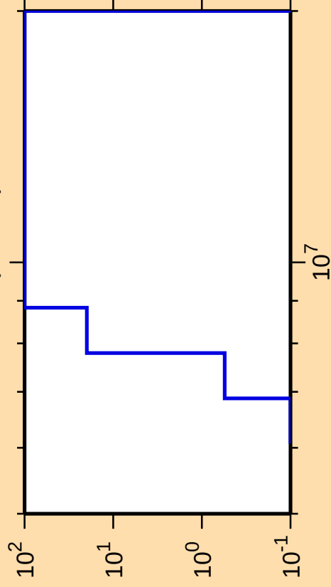
\Delta\sigma/\sigma vs. E for ^{167}\text{Ta}(n,\text{He3})
