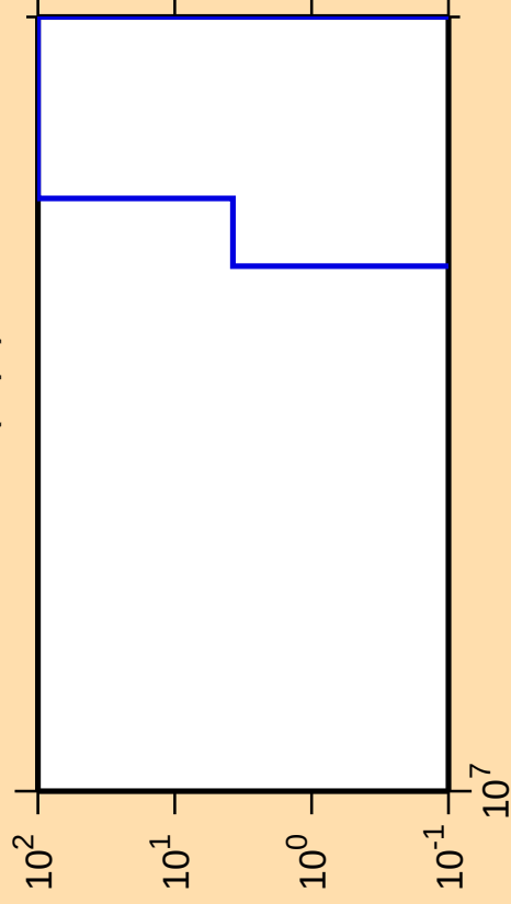
\Delta\sigma/\sigma vs. E for ^{167}\text{Ta}(n,\text{pt})
