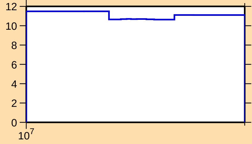
\Delta\sigma/\sigma vs. E for ^{167}\text{Ta}(n,\text{nonel.})
