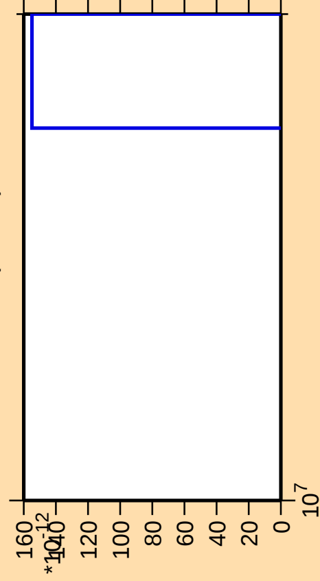
\Delta\sigma/\sigma vs. E for ^{180}\text{Ta}(\text{mt } 42)
