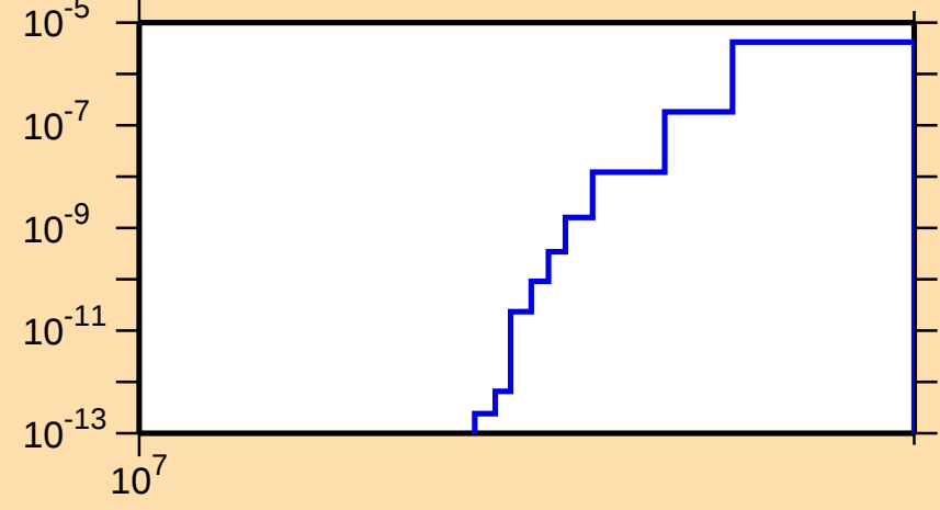
\sigma vs. E for ^{180}\text{Ta}(n,2np)
