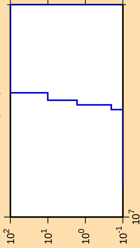
\Delta\sigma/\sigma vs. E for ^{180}\text{Ta}(n,\text{nt})
