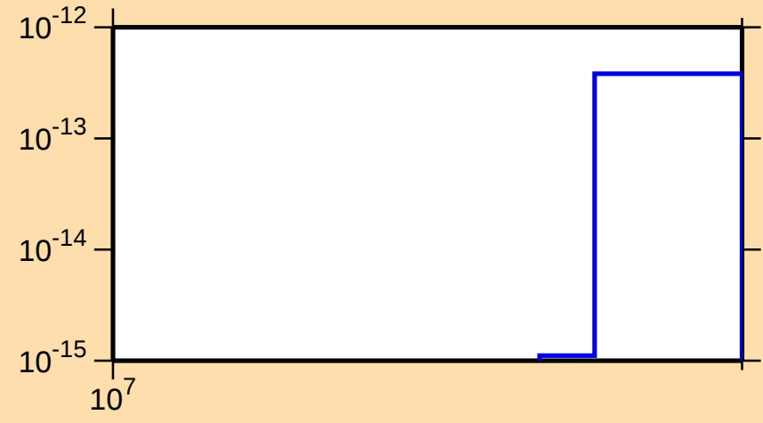
\sigma vs. E for ^{180}\text{Ta}(n,3n\alpha)
