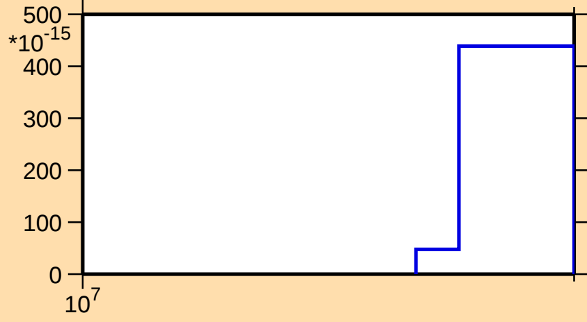
\sigma vs. E for ^{180}\text{Ta}(\text{mt117})
