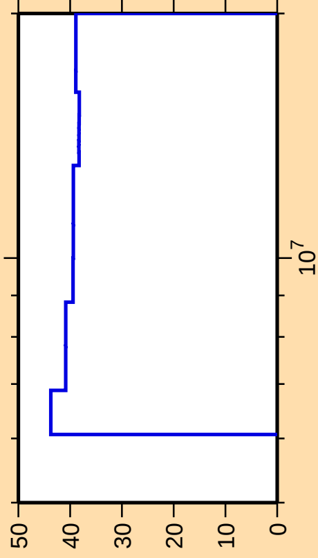
\Delta\sigma/\sigma vs. E for ^{180}\text{Ta}(n,p)
