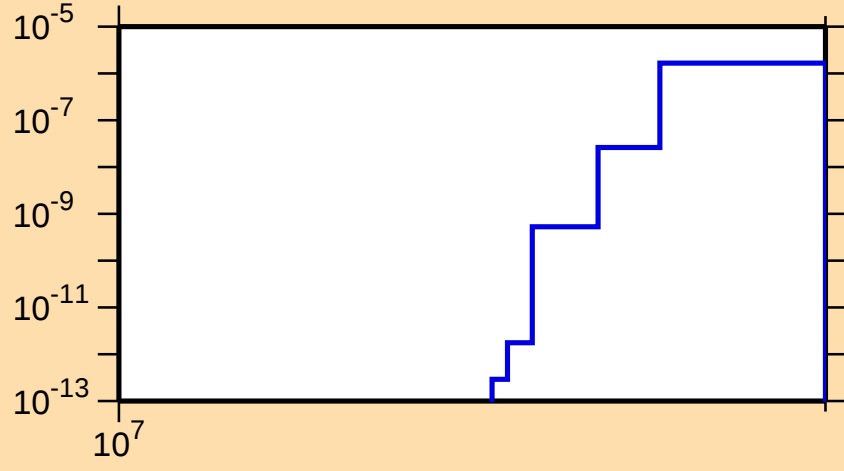
\sigma vs. E for ^{180}\text{Ta}(n,\text{nt})
