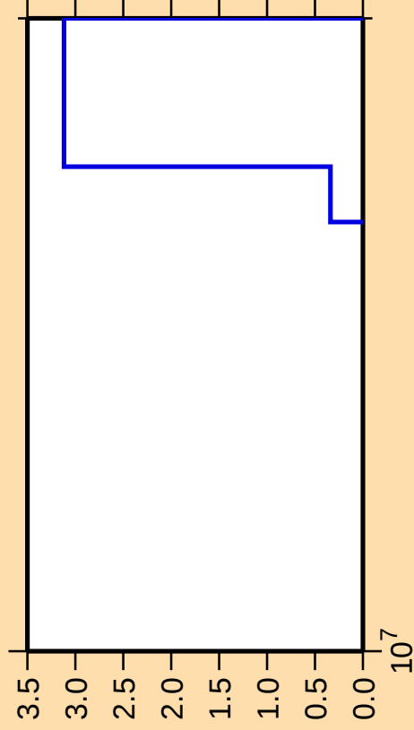
\Delta\sigma/\sigma vs. E for ^{180}\text{Ta}(\text{mt117})
