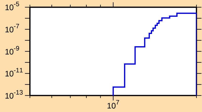
\sigma vs. E for ^{180}\text{Ta}(n,2n\alpha)
