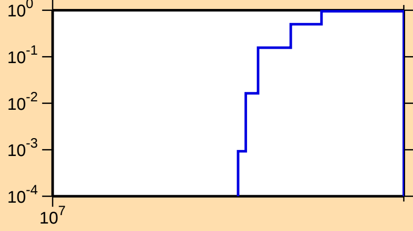
\sigma vs. E for ^{180}\text{Ta}(n,3n)
