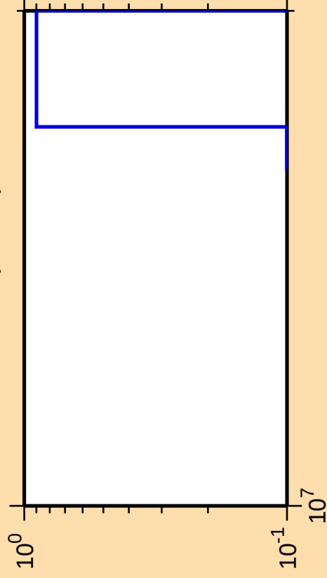
\Delta\sigma/\sigma vs. E for ^{180}\text{Ta}(n,3n\alpha)
