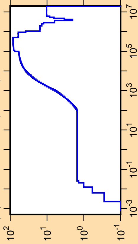
\Delta\mu/\mu vs. E for ^{183}\text{Ta}(\text{mt251})
