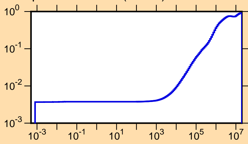
\mu vs. E for ^{183}\text{Ta}(\text{mt251})
