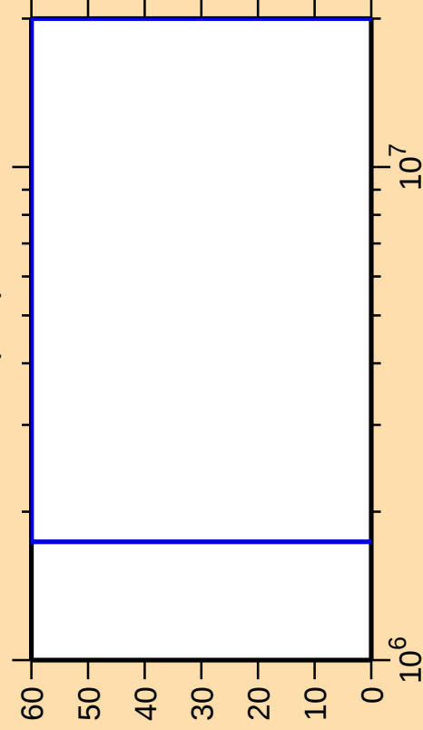
\Delta\sigma/\sigma vs. E for ^{183}\text{Ta}(n,\alpha)
