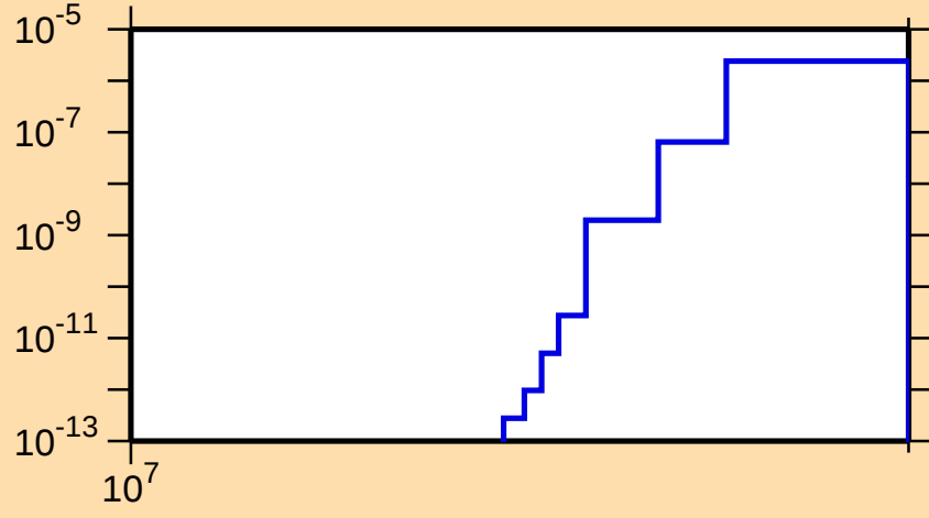
\sigma vs. E for ^{183}\text{Ta}(n,\text{nt})
