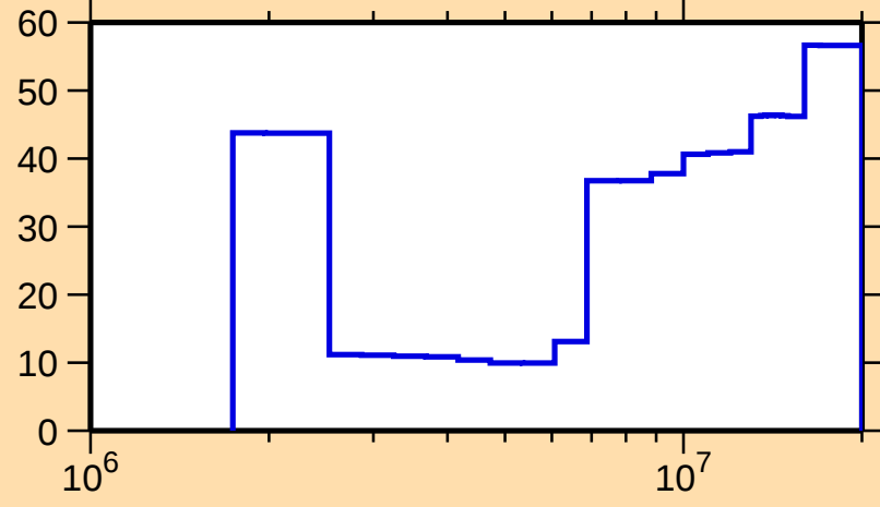
\Delta\sigma/\sigma vs. E for ^{183}\text{Ta}(n,n\text{cont.})
