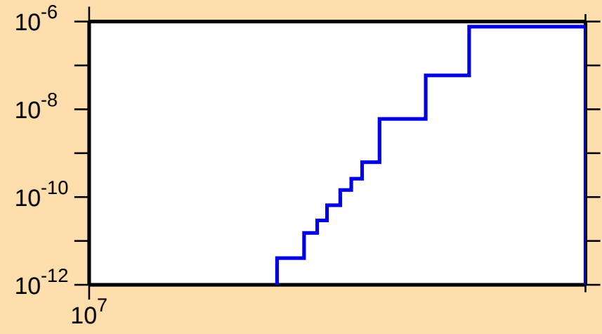
\sigma vs. E for ^{183}\text{Ta}(n,2n\alpha)
