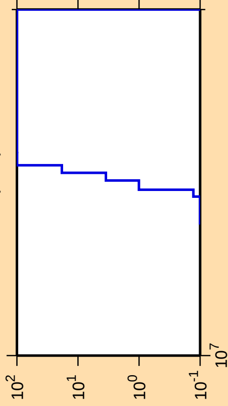
\Delta\sigma/\sigma vs. E for ^{183}\text{Ta}(n,\text{nt})
